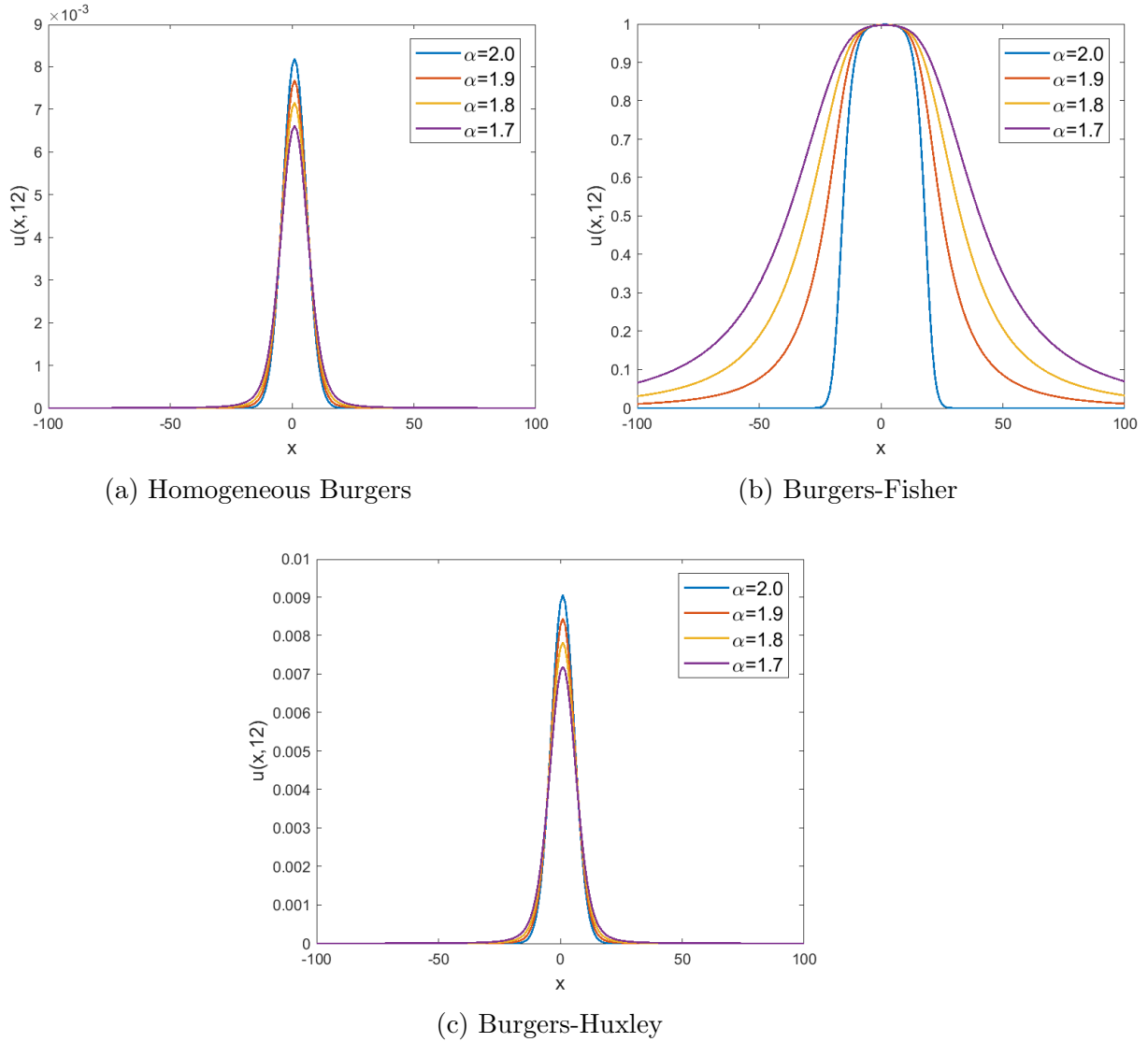
Figure 4.2: Comparison of solutions for various \alpha with \lambda = 0.1
