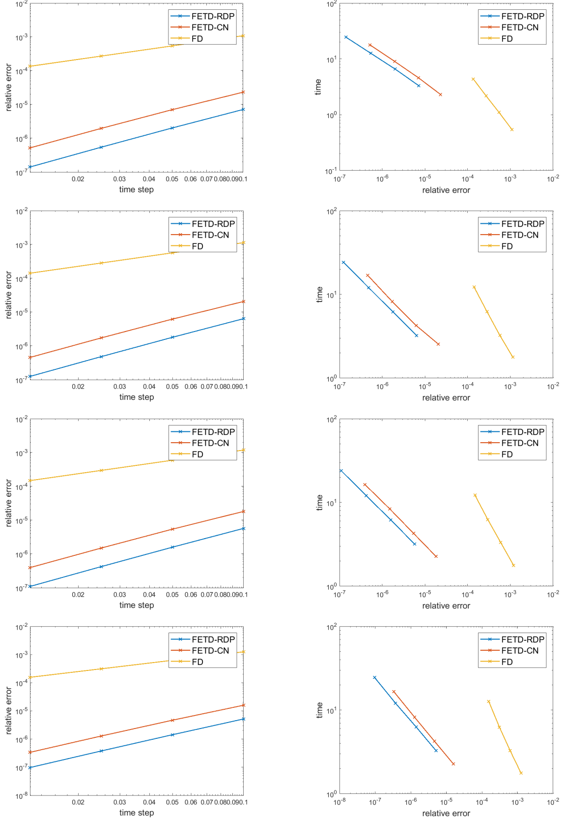
Figure 4.4: Homogeneous Burgers' equation with \lambda = 1 : convergence plots (left) and efficiency plots (right) for fractional parameters \alpha = 2.0, 1.9, 1.8, 1.7 (from top to bottom)
