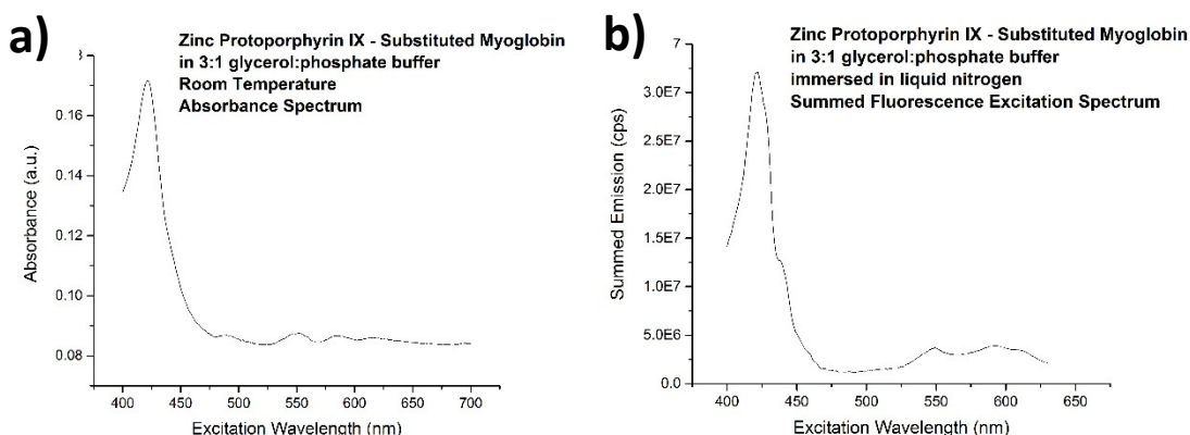
Figure 5.10. The summed fluorescence excitation method produces a comparable line shape to absorbance spectroscopy. a) Absorbance spectrum of zinc protoporphyrin IX-substituted myoglobin at room temperature. b) Summed fluorescence excitation spectrum of the same species at low temperature.
