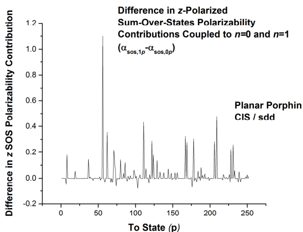
Figure 7.5c. Predictive plot for z-polarized states of influence on the Q_x transition of planar porphyrin.
