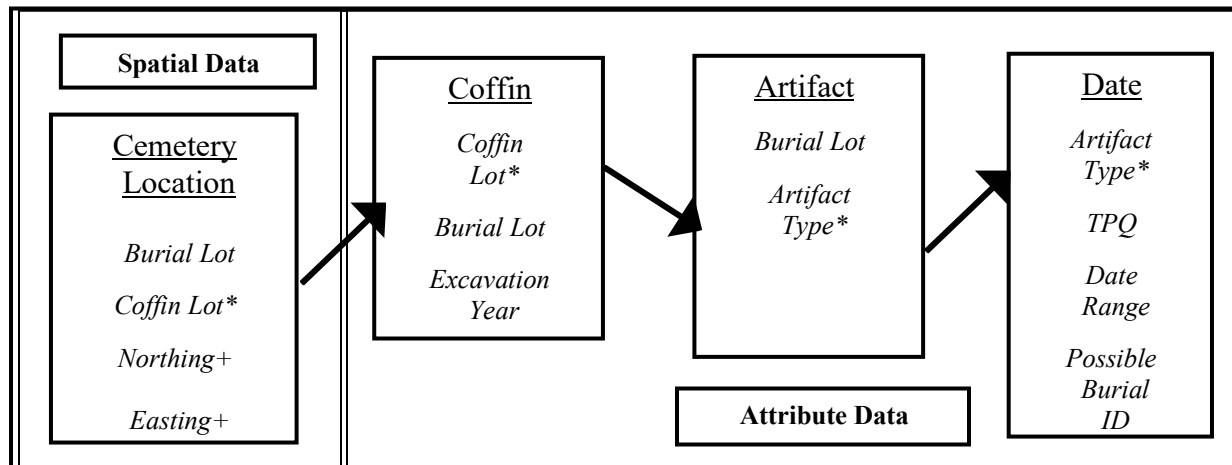
Figure 3.2: Entity-Relationship diagram for the database design (adapted from Conolly and Lake 2006:56) [boxes = entities and attributes, arrows = relationships, * = unique values, and + = spatial attribute]
