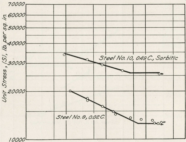
FIG. 34. S-N DIAGRAMS, OLSEN-FOSTER TESTS, 0.93 CARBON STEEL, 0.02 CARBON STEEL, AND 0.49 CARBON STEEL
