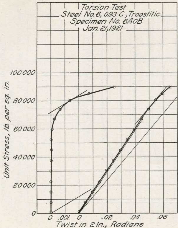
FIG. 23. REPRESENTATIVE STRESS-STRAIN DIAGRAMS FOR TORSION TESTS
