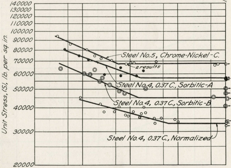
FIG. 25. S-N DIAGRAMS FOR CHROME-NICKEL STEEL AND FOR 0.37 CARBON STEEL, ROTATING-BEAM TESTS Logarithmic abscissas give thousands of cycles for rupture
