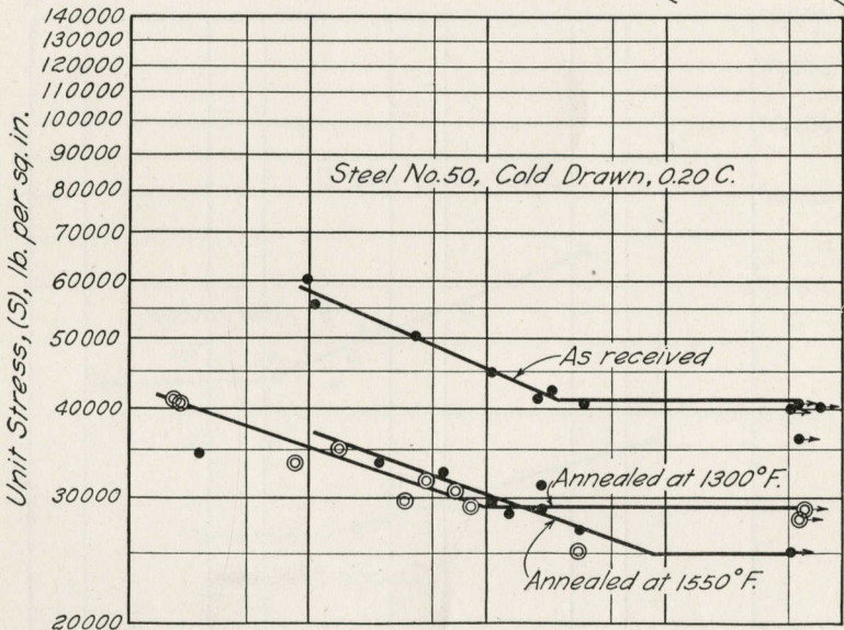
FIG. 27. S-N DIAGRAMS FOR HOT-ROLLED STEEL AND FOR COLD-DRAWN STEEL, ROTATING-BEAM TESTS
