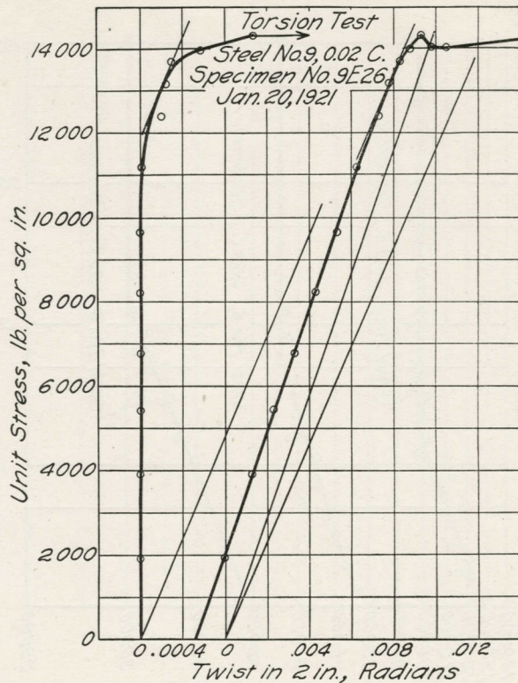
FIG. 23. REPRESENTATIVE STRESS-STRAIN DIAGRAMS FOR TORSION TESTS
