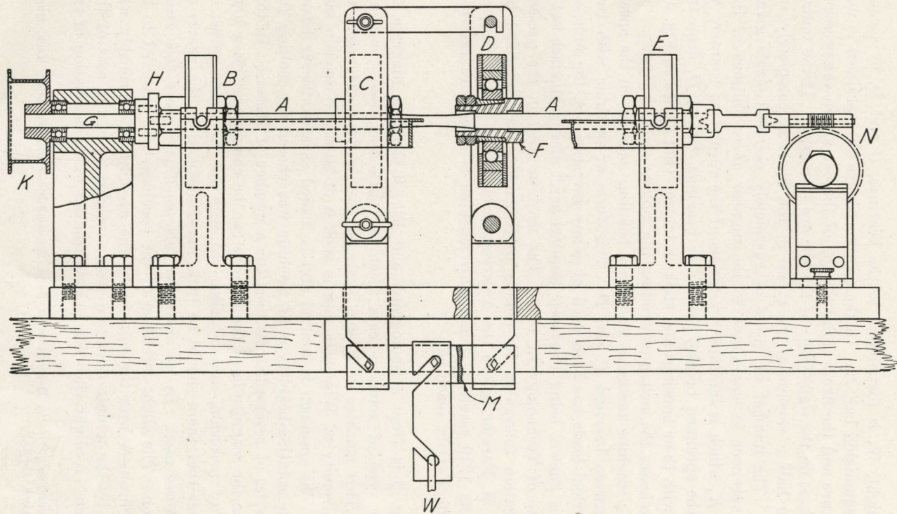
FIG. 4. DIAGRAM OF ROTATING-BEAM TESTING MACHINE (FARMER)
