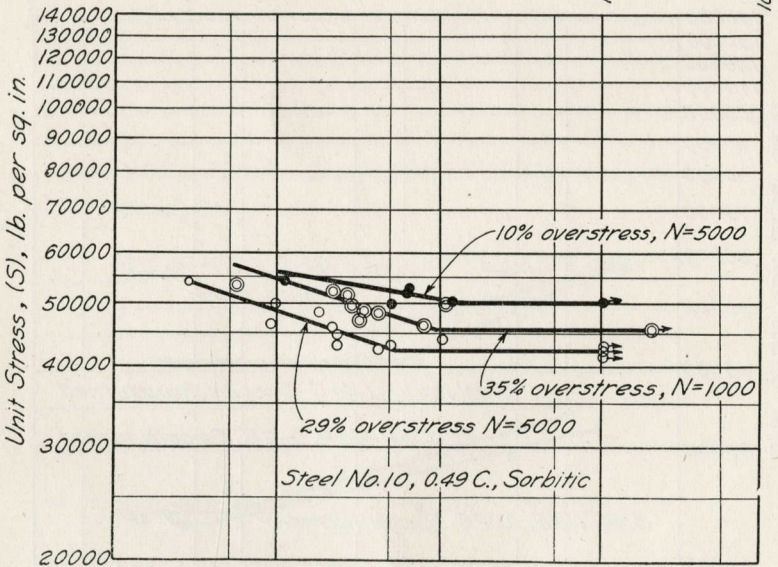
FIG. 30. S-N DIAGRAMS SHOWING EFFECT OF OVERSTRESS, 0.49 CARBON STEEL, ROTATING-BEAM TESTS
