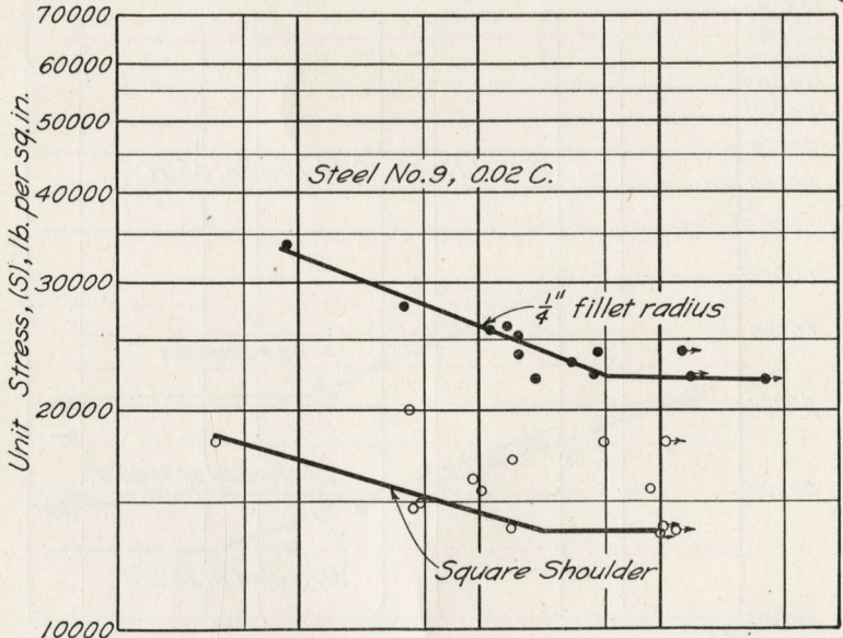
FIG. 28. S-N DIAGRAMS SHOWING EFFECT OF SHAPE OF SPECIMEN, ROTATING-BEAM TESTS Logarithmic abscissas give thousands of cycles for rupture
