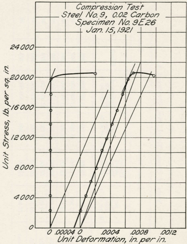
FIG. 22. REPRESENTATIVE STRESS-STRAIN DIAGRAMS FOR COMPRESSION TESTS
