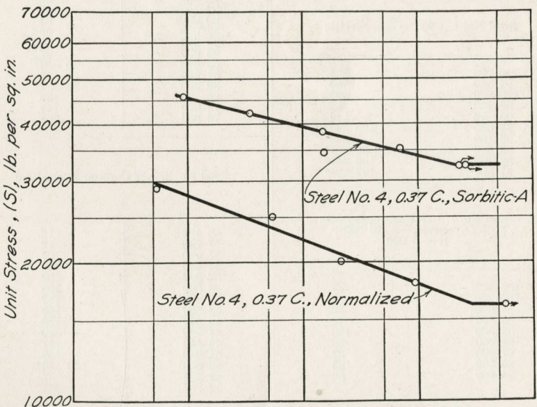
FIG. 35. S-N DIAGRAMS, OLSEN-FOSTER TESTS, 0.37 CARBON STEEL, AND CHROME-NICKEL STEEL
