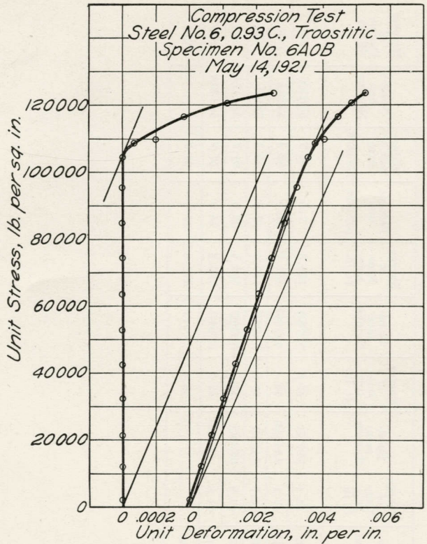
FIG. 22. REPRESENTATIVE STRESS-STRAIN DIAGRAMS FOR COMPRESSION TESTS
