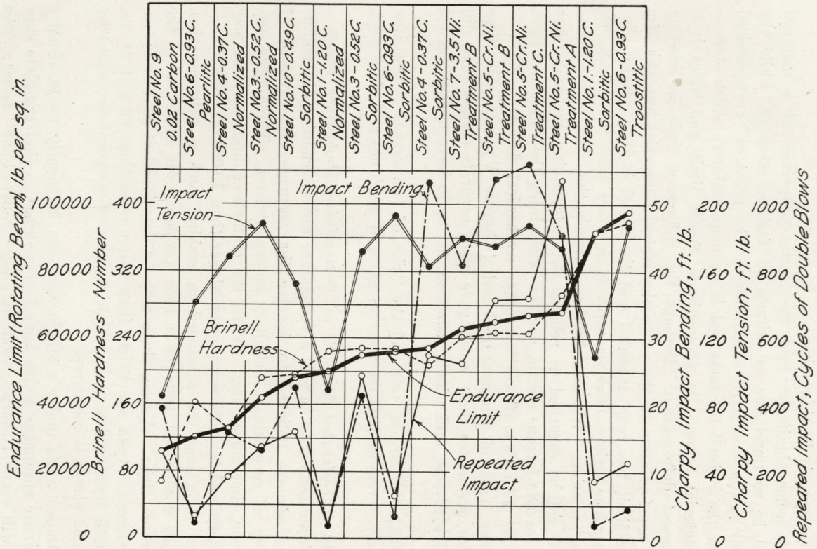
FIG. 38. COMPARISON OF ENDURANCE LIMITS WITH BRINELL HARDNESS, CHARPY IMPACT BENDING VALUES, CHARPY IMPACT-TENSION VALUES, AND REPEATED-IMPACT VALUES
