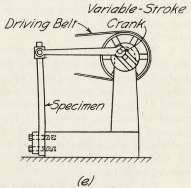
FIG. 45. DIAGRAMS OF TYPICAL REPEATED-STRESS TESTING MACHINES
