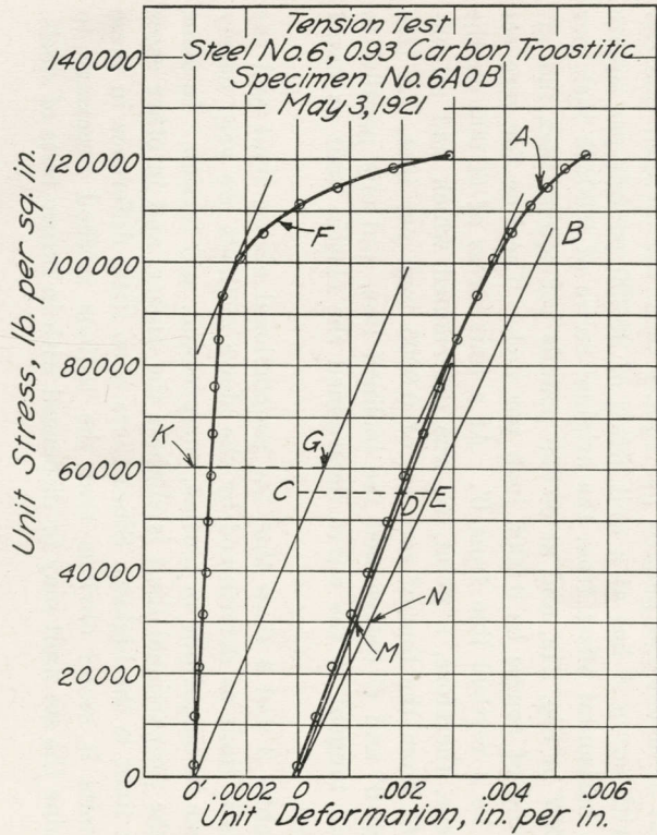
FIG. 21. REPRESENTATIVE STRESS-STRAIN DIAGRAMS FOR TENSION TESTS
