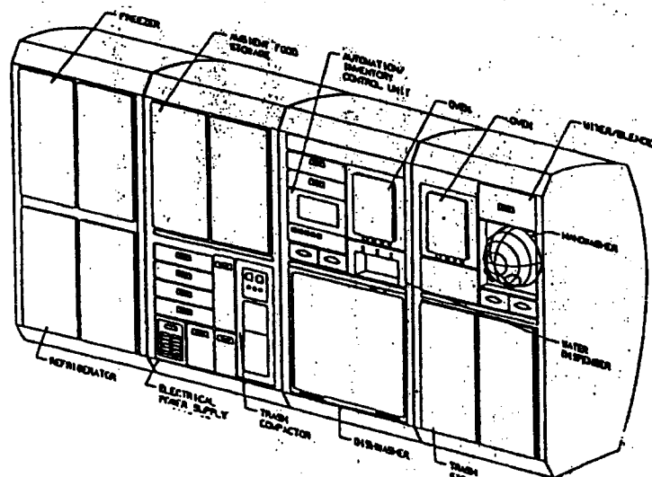
Figure 8.2.1 Galley Layout (NASA-JSC Crew Systems Review, 1988)
