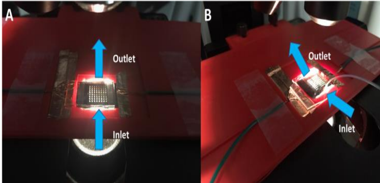
Figure 12. The inlet and outlet of the suggested LOC device: (A) using osmotic pressure; (B) using syringe pump
