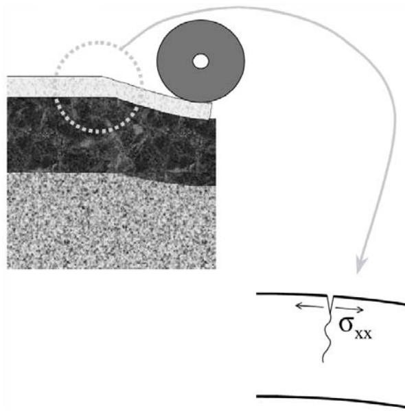
Figure 5. Corner cracking mechanism (Rasmussen et al. 2002)
