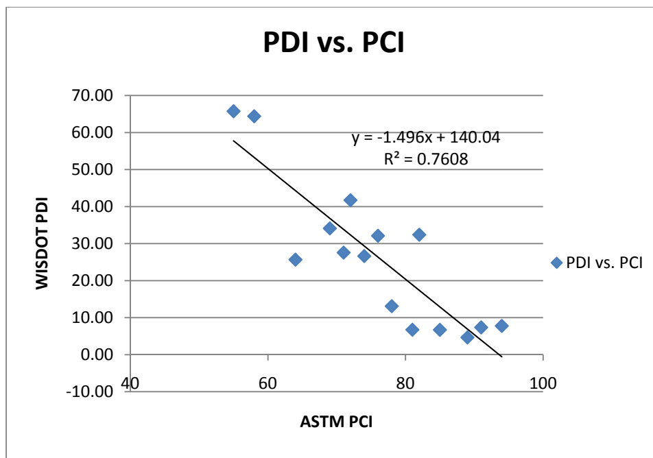
Figure 40. Linear Relationship between ASTM PCI and WisDOT PDI
