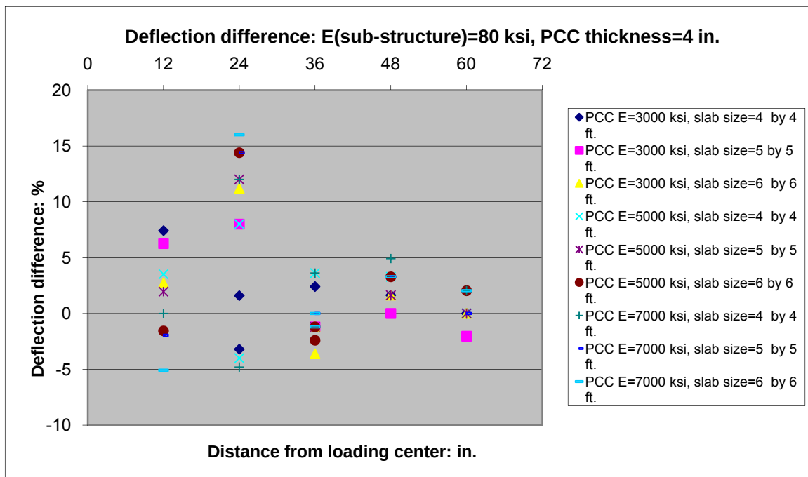
Figure 37. Plots of Deflection Differences for Sub-structure Modulus=80 ksi, PCC thickness=4 in.
