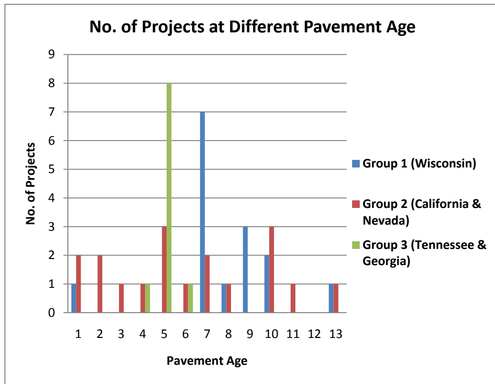
Figure 45. Number of Projects at Different Pavement Age for 3 Groups
