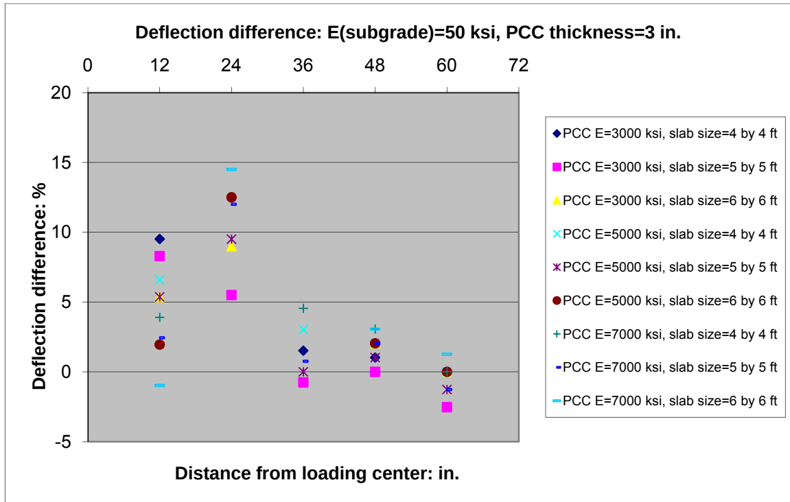
Figure 34. Plots of Deflection Differences for Sub-structure Modulus=50 ksi, PCC thickness=3 in.
