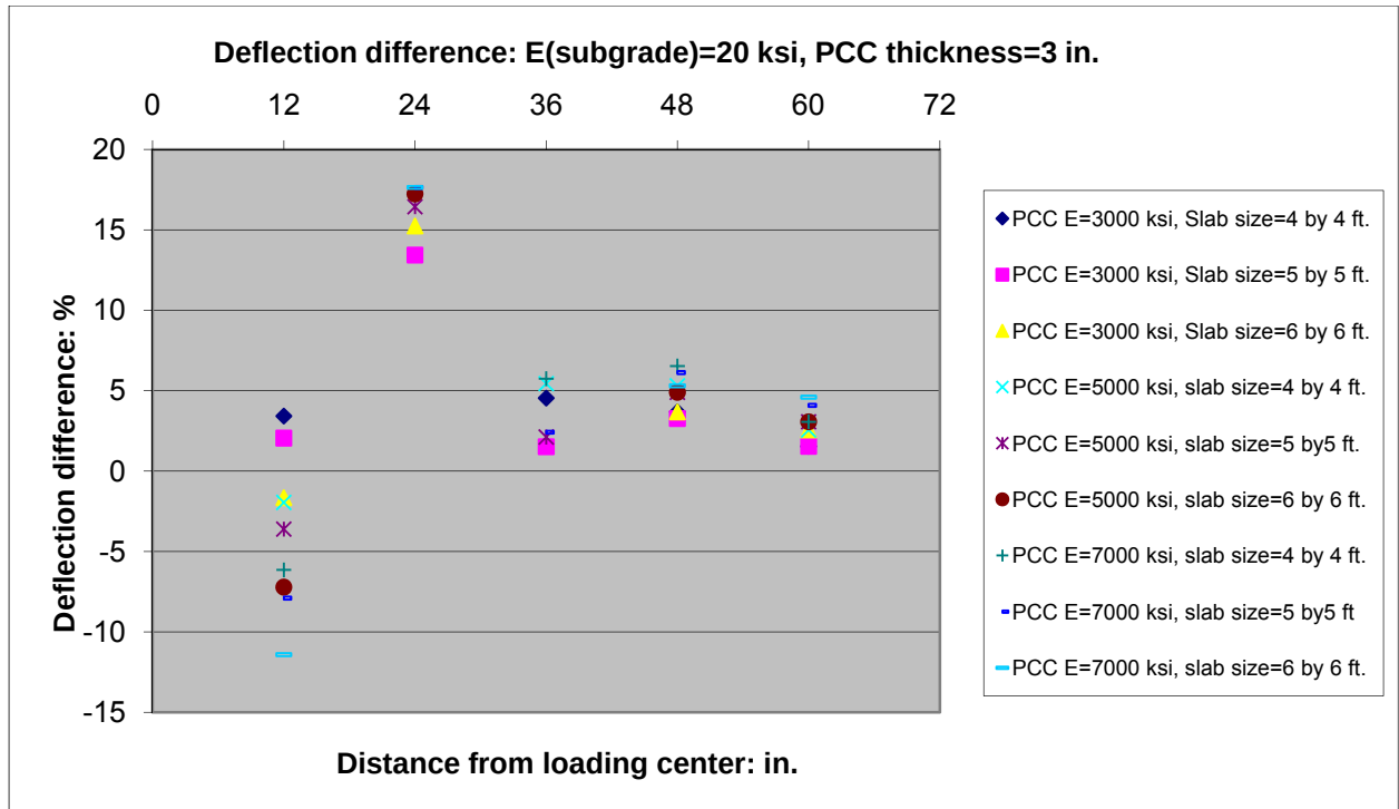
Figure 32. Plots of Deflection Differences for Sub-structure Modulus=20 ksi, PCC Thickness=3 in.
