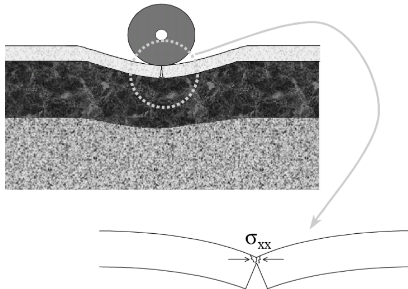
Figure 12. Joint Spalling Mechanisms (Rasmussen et al. 2002)
