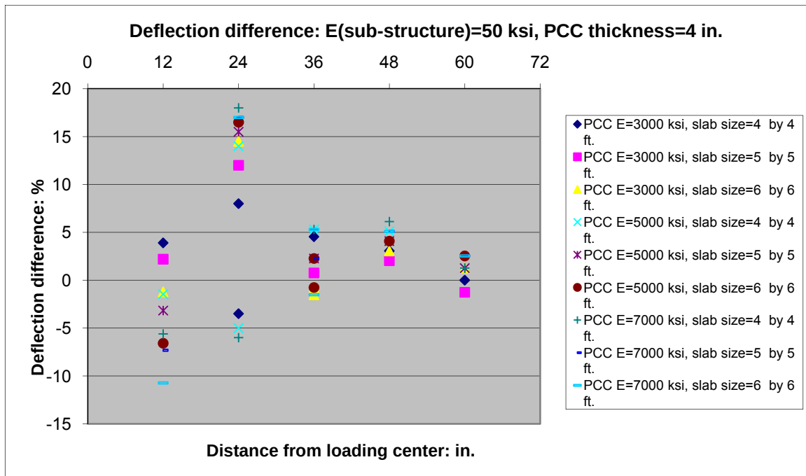
Figure 35. Plots of Deflection Differences for Sub-structure Modulus=50 ksi, PCC thickness=4 in.
