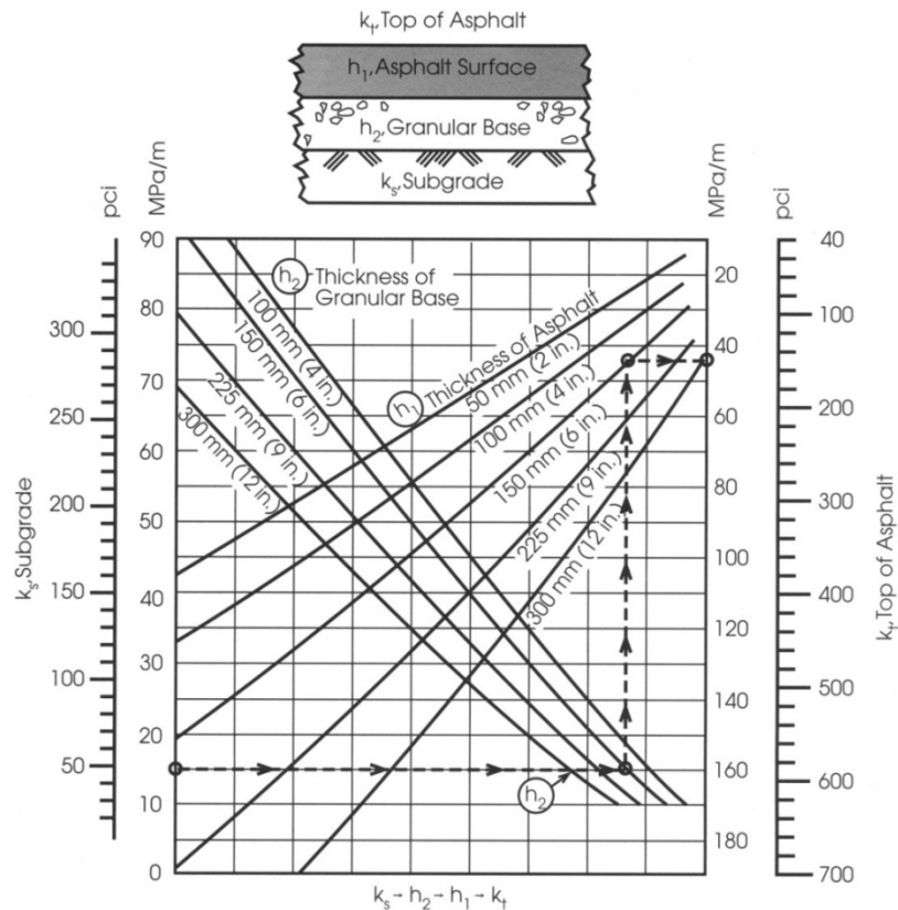
Figure 2. k-value on top of HMA pavement with granular base (ACPA 2002)
