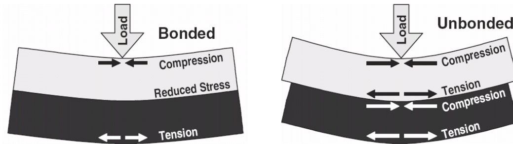
Figure 1. Bonded Vs. Unbonded behavior (Rasmussen et al. 2004)
