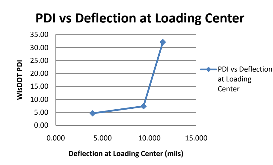
Figure 43. Relationship between WisDOT PDI and FWD Deflection at Loading Center
