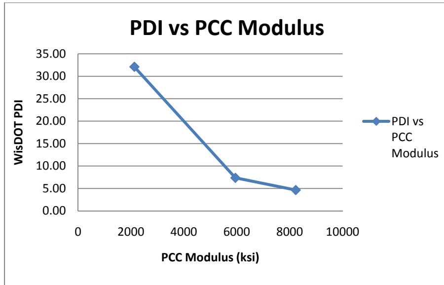
Figure 42. Relationship between WisDOT PDI and PCC Modulus
