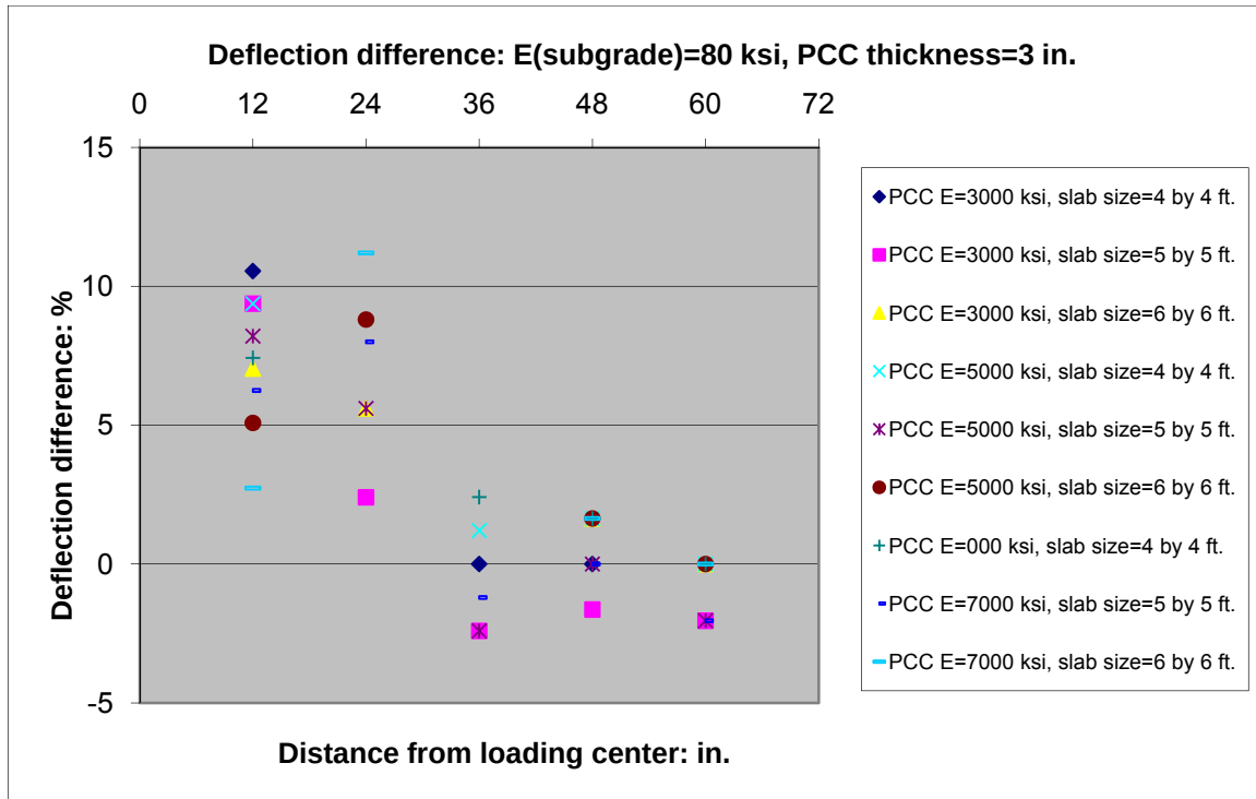
Figure 36. Plots of Deflection Differences for Sub-structure Modulus=80 ksi, PCC thickness=3 in.
