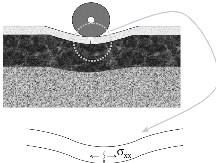
Figure 7. Mid-slab cracking mechanisms (Rasmussen et al. 2002)
