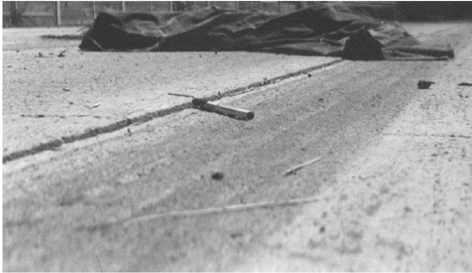
Figure 8. Longitudinal Faulting (Rasmussen et al. 2002)
