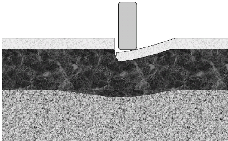
Figure 9. Longitudinal joint faulting mechanisms (Rasmussen et al. 2002)
