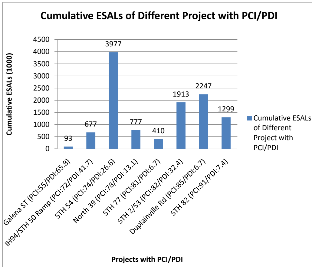
Figure 41. Cumulative ESALs of Different Projects
