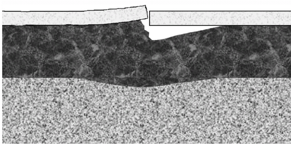
Figure 10. Transverse joint faulting mechanisms (Rasmussen et al. 2002)
