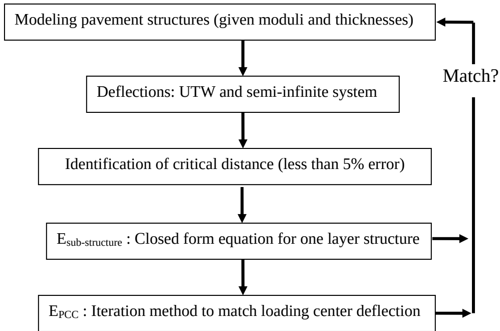
Figure 31. Flow Chart of the Research Procedure
