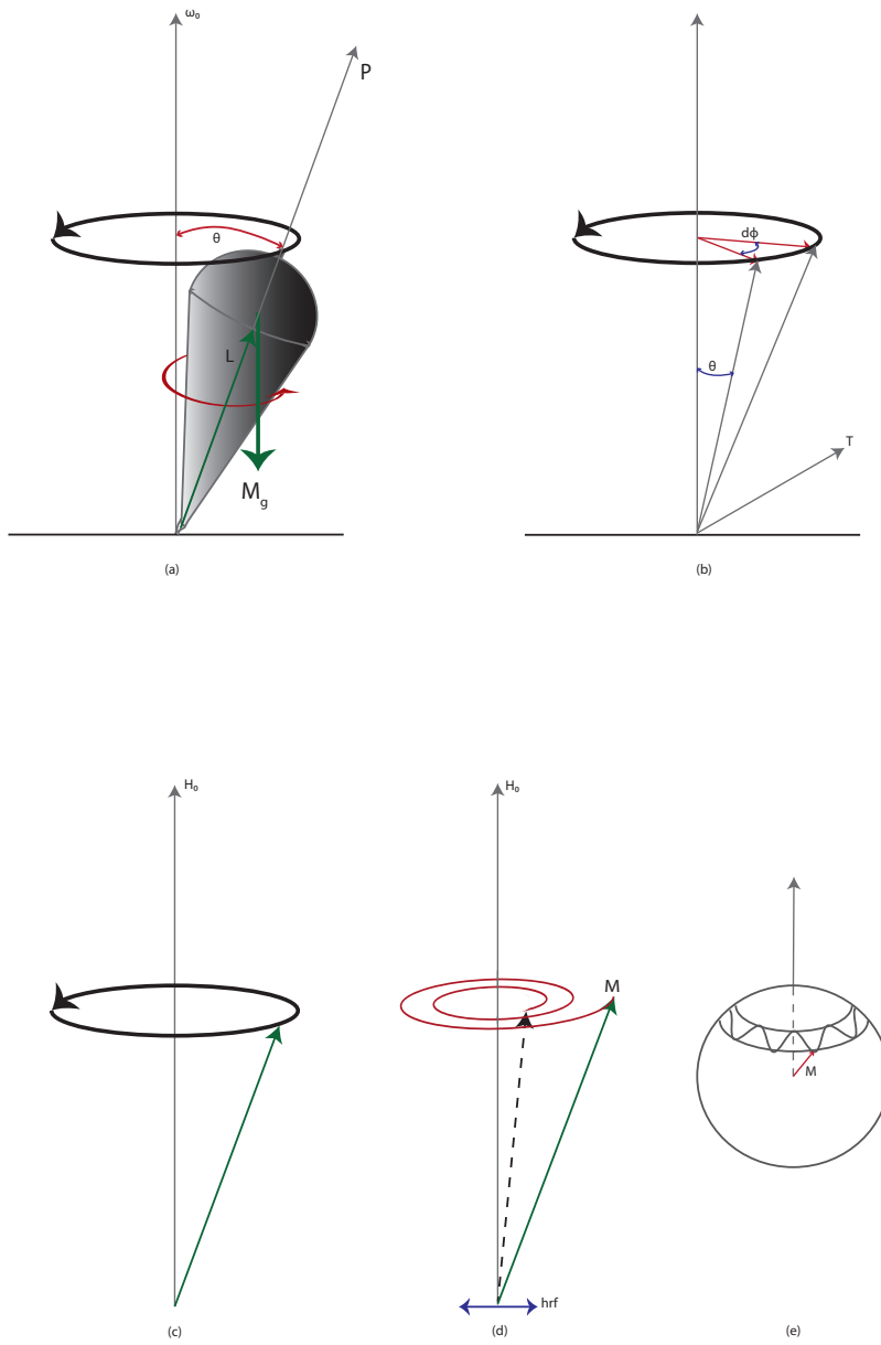
Figure 2-8: (a) Precessional motion of a spinning symmetrical top in a gravitational field (rigid body at frequency \omega_0 ). (b) Angular momentum and torque vectors. (c) Precession of the magnetized vector in a constant magnetic field. (d) Precession of the magnetization vector in an alternating magnetic field when \omega \neq \omega_0 . (e) The magnitude of a magnetization vector is constant so that oscillation takes place on the surface of the radius |M| .
