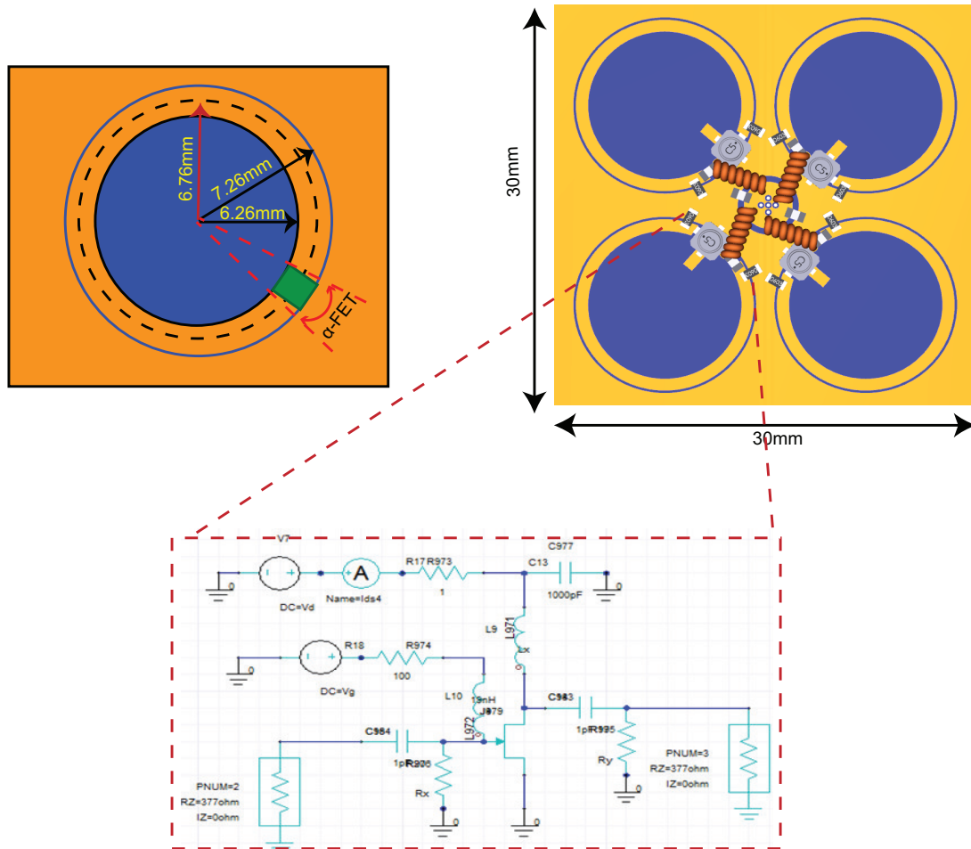
Figure 3-5: Unit super-cell consisting of 4 rings in a 90^\circ -symmetric configuration. Dimensions of the ring resonator and loaded circuit configuration for each ring slot.
