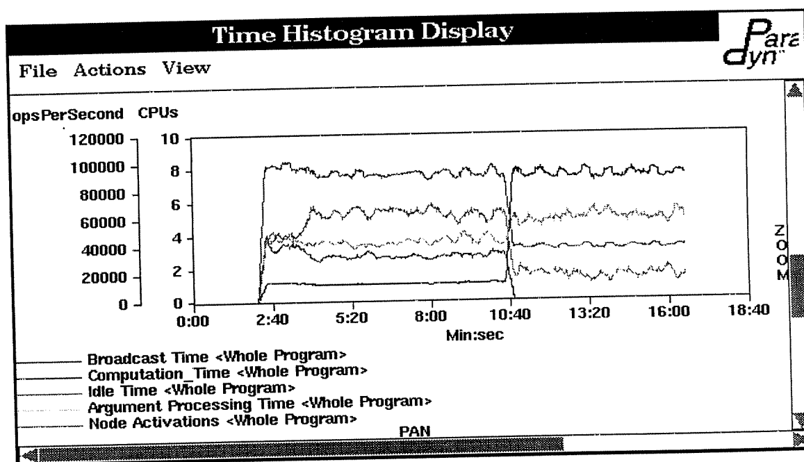
Figure 32: Node-level View of Performance for Peace
