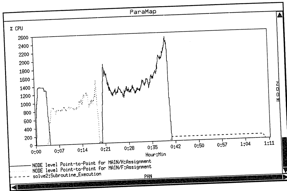
Figure 17: Time plot of CPU Time for the entire initial parallel DRBEM application. The display shows three primary runtime contributors: Point-to-Point communications that map to arrays MAIN/H and MAIN/F , and sequential execution in the routine solve2
