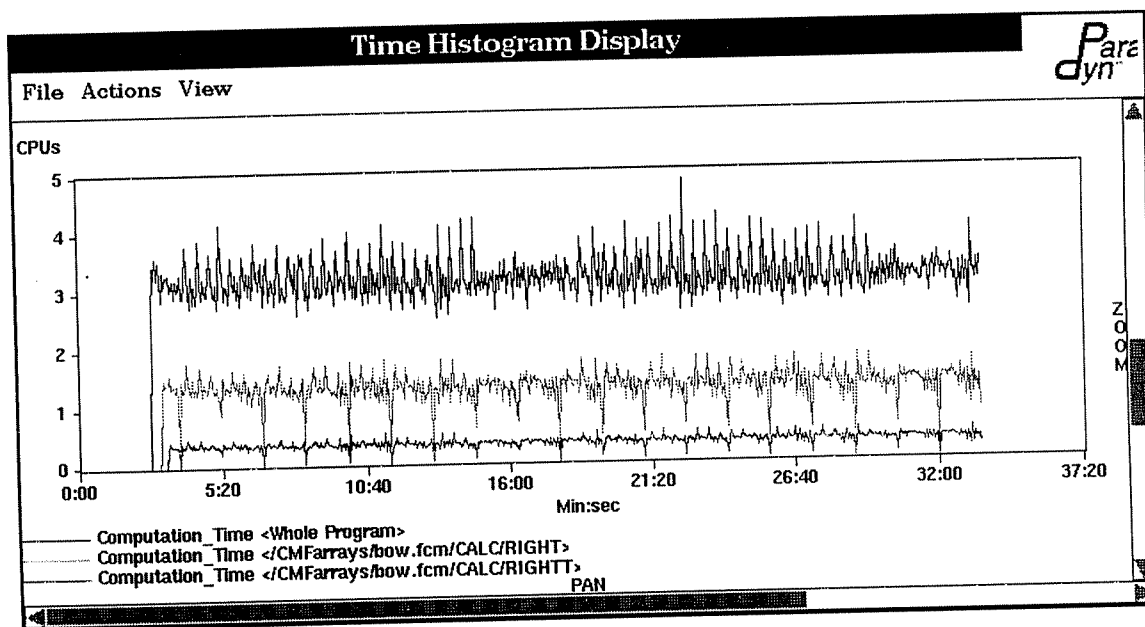
Figure 25: Performance for Righthand Convolution Matrices.
