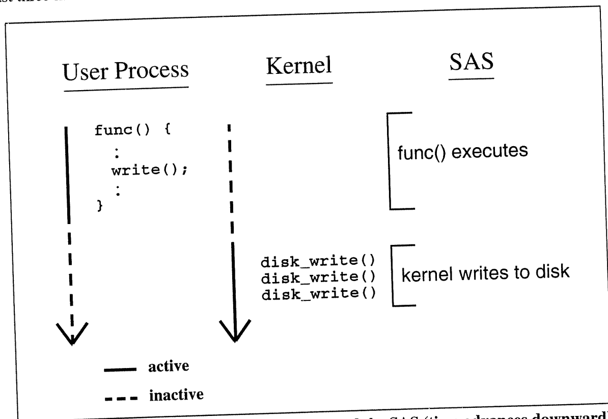
Figure 9: Asynchronous sentence activations and the SAS (time advances downward)
