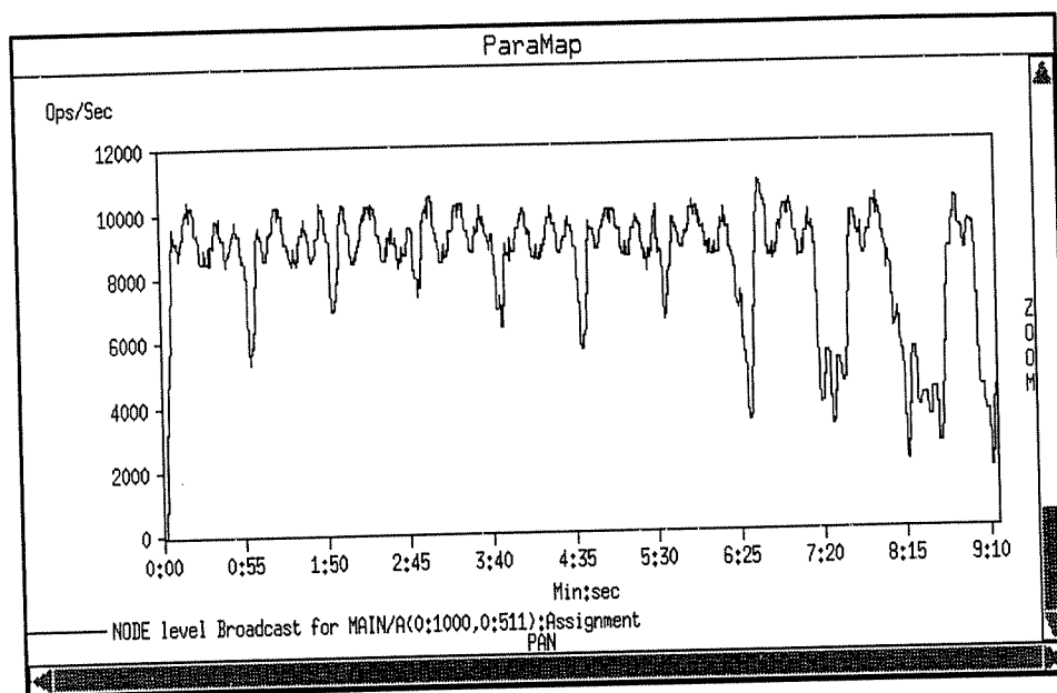
Figure 12: Time plot of Broadcasts that map to an array sub-region. Only events from the nodes that map to the selected sub-region are shown.
