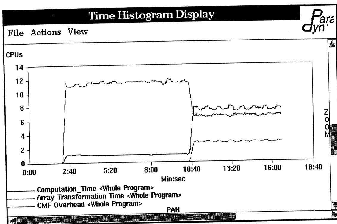
Figure 31: CMF-level Performance for Peace
