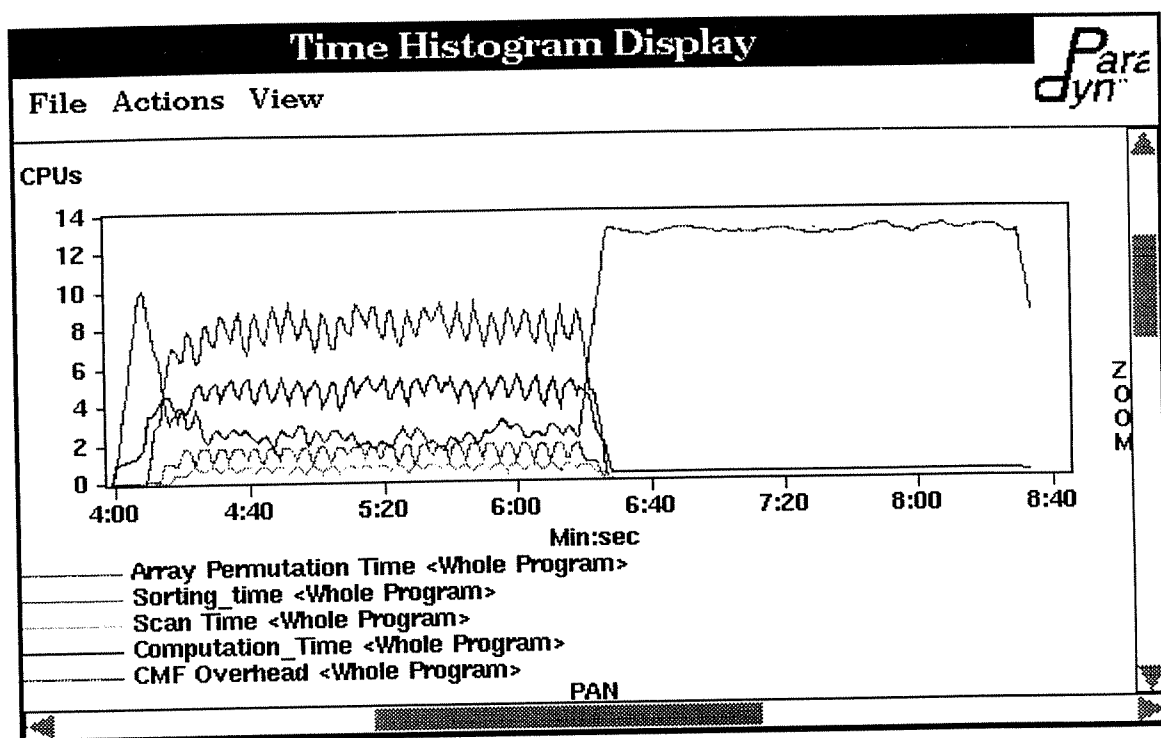
Figure 36: CMF-level Performance for PSICM
