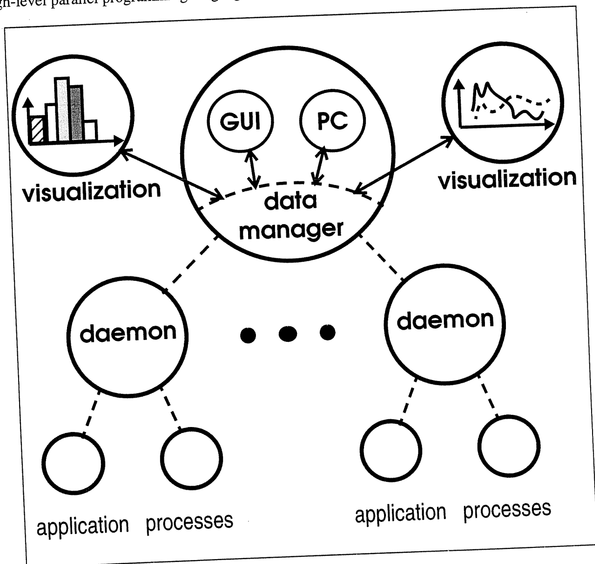
Figure 19: Basic structure of Paradyn
