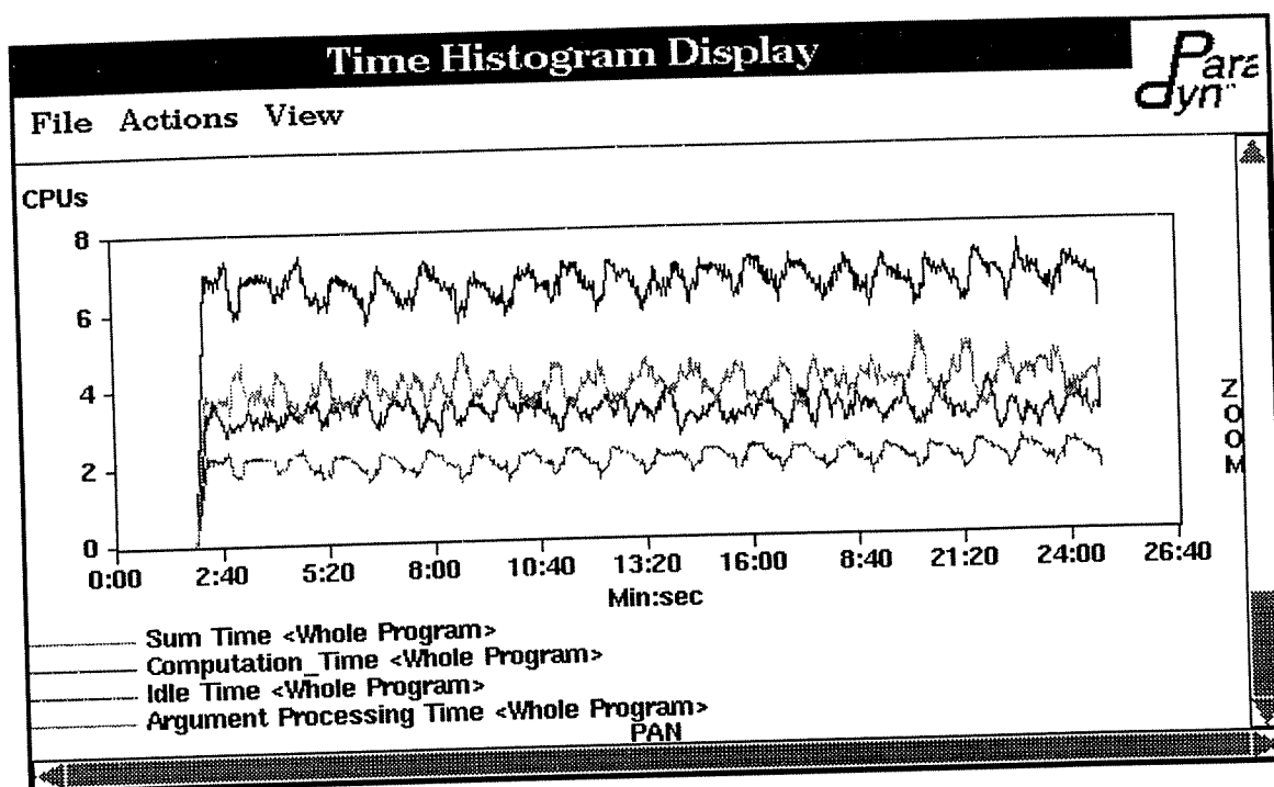
Figure 29: Paradyn Display of Improved Bow
