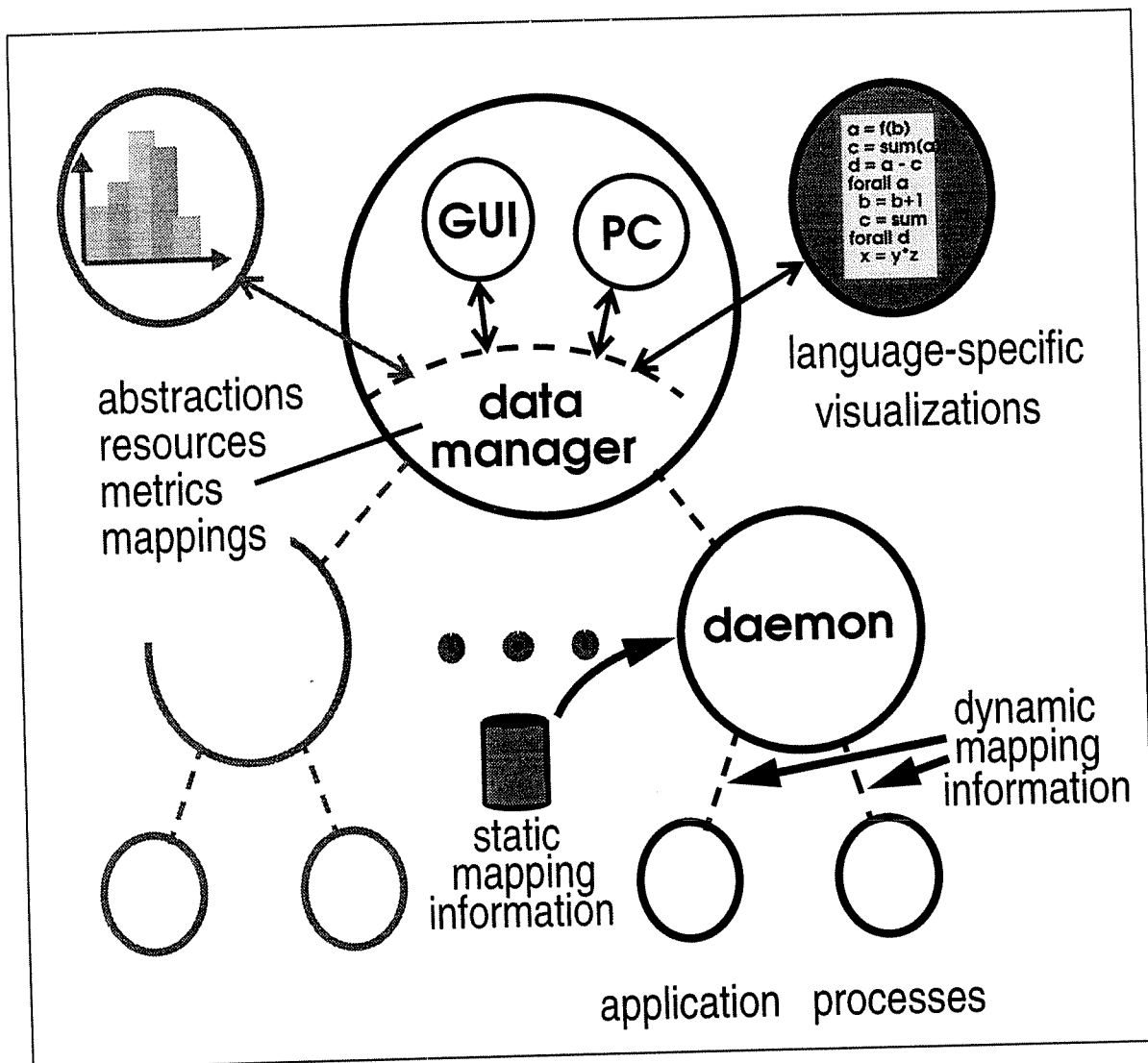
Figure 20: Updated Paradyn structure.
