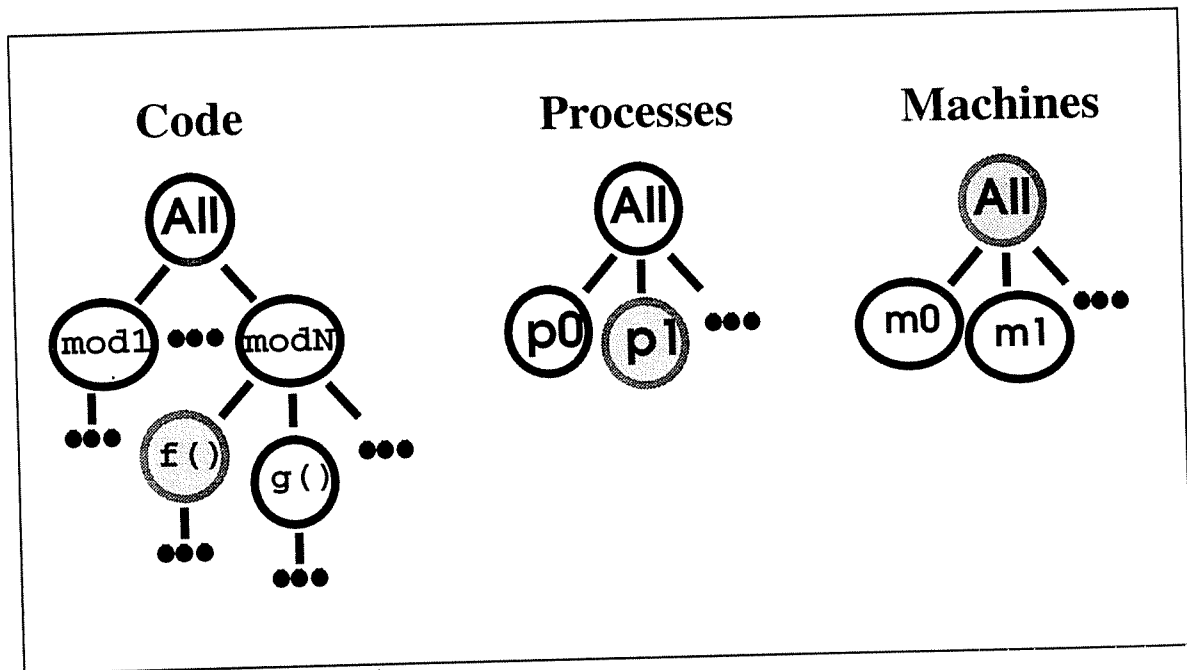
Figure 18: Example Resource Hierarchies and Focus Selection
