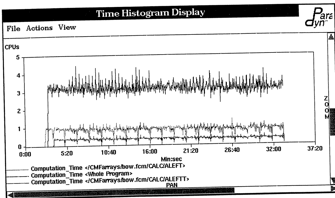
Figure 26: Performance for Lefthand Convolution Matrices
