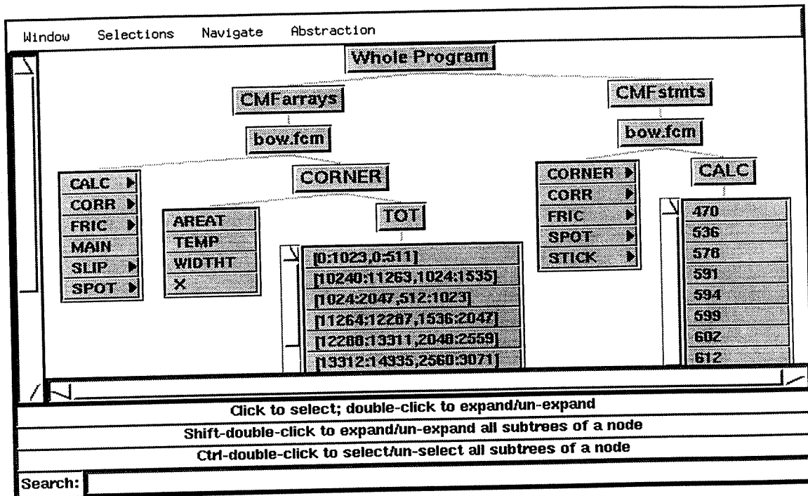
Figure 21: CMF-Level Where Axis
