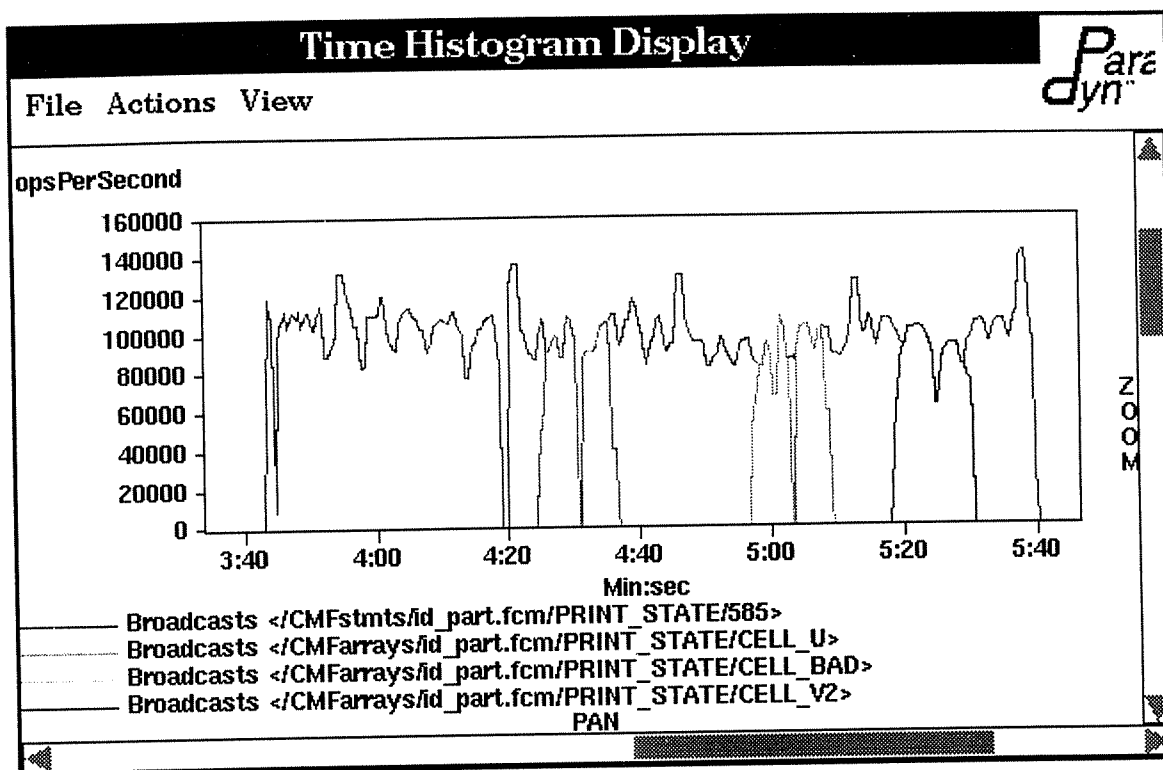
Figure 38: Code and Data Views of Performance for Second Phase of PSICM (note that both code and data views are visible in this figure)
