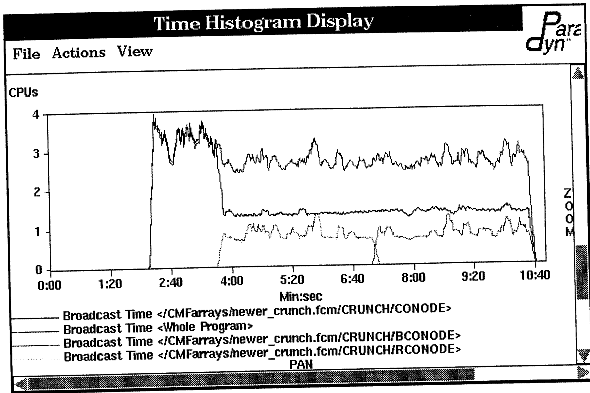
Figure 33: Node-level Broadcasts Constrained by CMF-level Arrays
