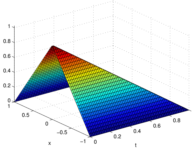
Figure 2.2.: \min(1-t, 1-|x|)
