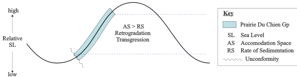
Figure 93. Model of the sea level driven accommodation space and sedimentation rate relationship that drove retrogradation during deposition of the Prairie du Chien.
