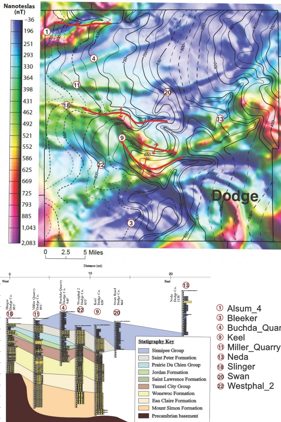
Figure 102. Sinnipee Group elevation contours and folds superimposed on aeromagnetic anomalies showing strong correlation (modified from Stewart, 2021). Vertically exaggerated cross section of Dodge County cores show Cambrian and Ordovician strata’s relationship to Precambrian surface (dark red).
