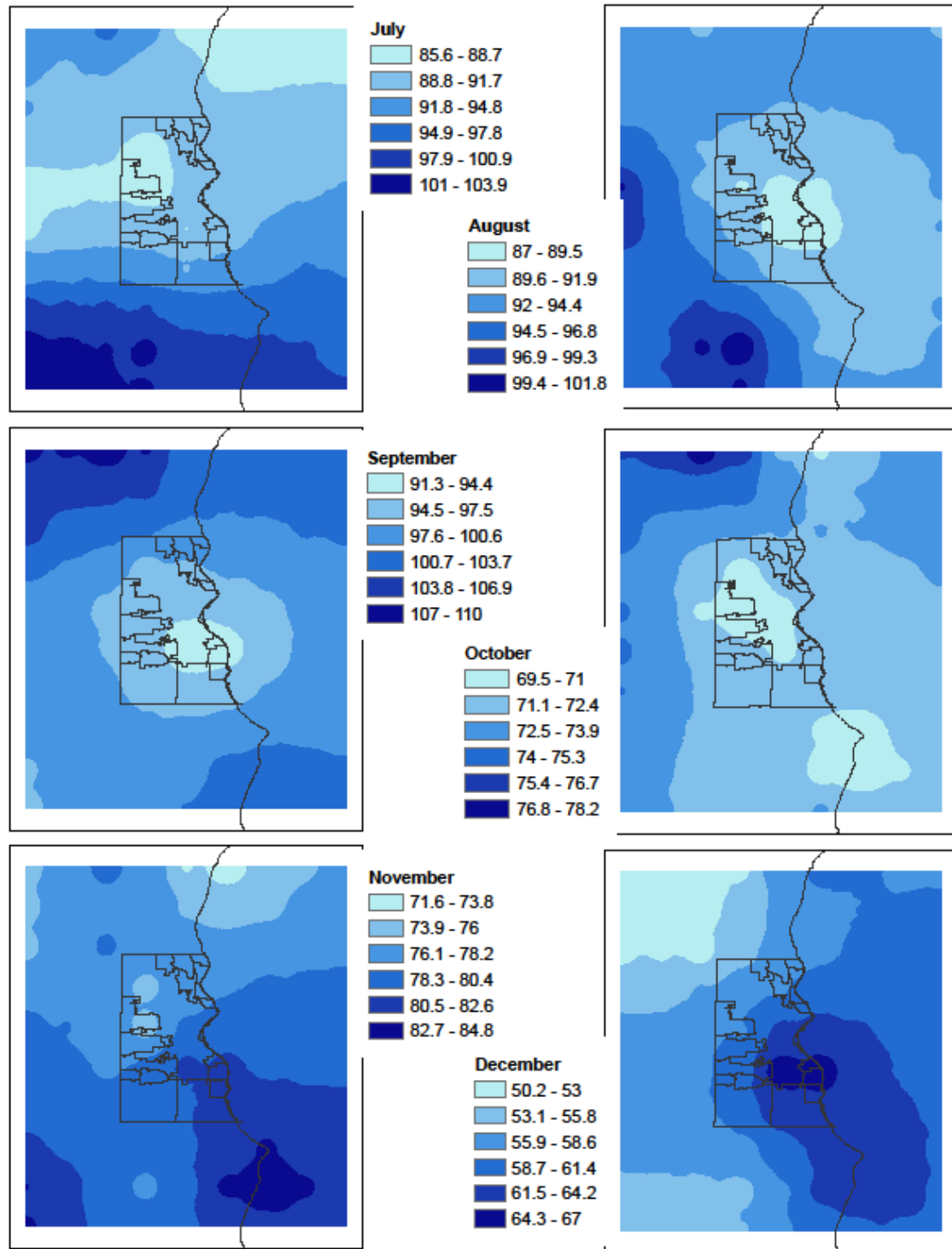
Fig. 22f: Spatial variation of projected mean monthly precipitation (mm) for the B1 emission scenario for the 2080s for July to December
