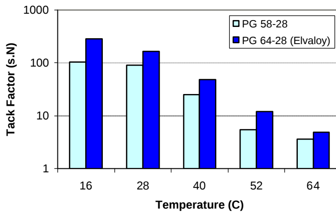
Figure 3.21 Effect of Temperature on Tack Factor
