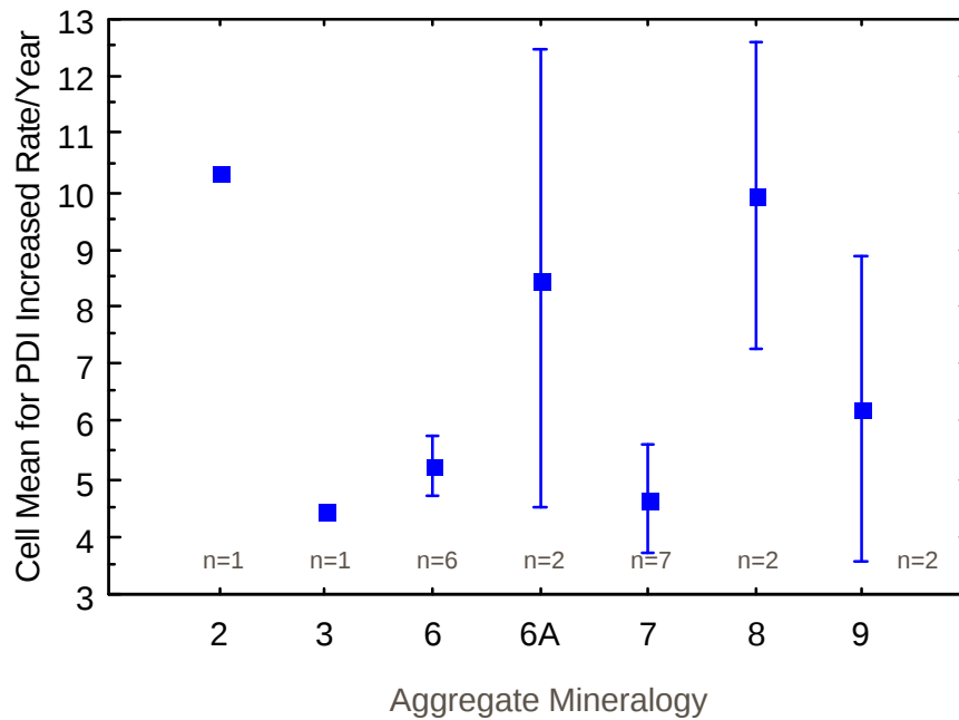
Figure 2.5 Effect of Aggregate Mineralogy on DPDI/Year
