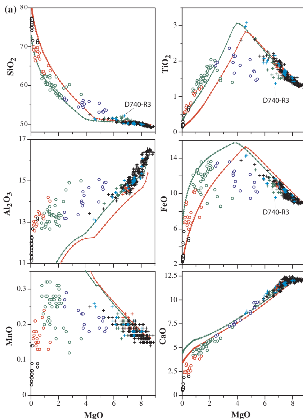
Figure 16. MgO variation diagrams of AR lavas for (a) \text{SiO}_2 , \text{TiO}_2 , \text{Al}_2\text{O}_3 , \text{FeO} , \text{MnO} , and \text{CaO} and (b) \text{Na}_2\text{O} , \text{K}_2\text{O} , \text{P}_2\text{O}_5 , \text{S} , and \text{Cl} subdivided by lithology and location. Basalt sample D740-R3 and E-MORB D746-R12 are labeled where their compositions are distinctive and discussed in the text. Most, but not all basalts, andesites, dacites, and rhyolites follow crystal fractionation trends that highlight that titanomagnetite begins to crystallize at \text{MgO} = \sim 4.5 wt % and apatite at \text{MgO} = \sim 2 wt %. Most basaltic andesites, some andesites, and basalt D740-R3 are hybrid lavas formed by mixtures of basalts with 7.5–8.0 wt % \text{MgO} and silicic lavas with \text{MgO} < \sim 1\% . Most hybrid lavas are located north of the rhyolite dome. Two RhyoliteMELTS models are shown using sample D395-R11 (supporting information Table S1) as the starting composition with 0.20 wt % \text{H}_2\text{O} , and pressure of 0.2 or 1 kbar and oxidation state of QFM or QFM-1 for the model. See text for discussion of the models and their implications.
