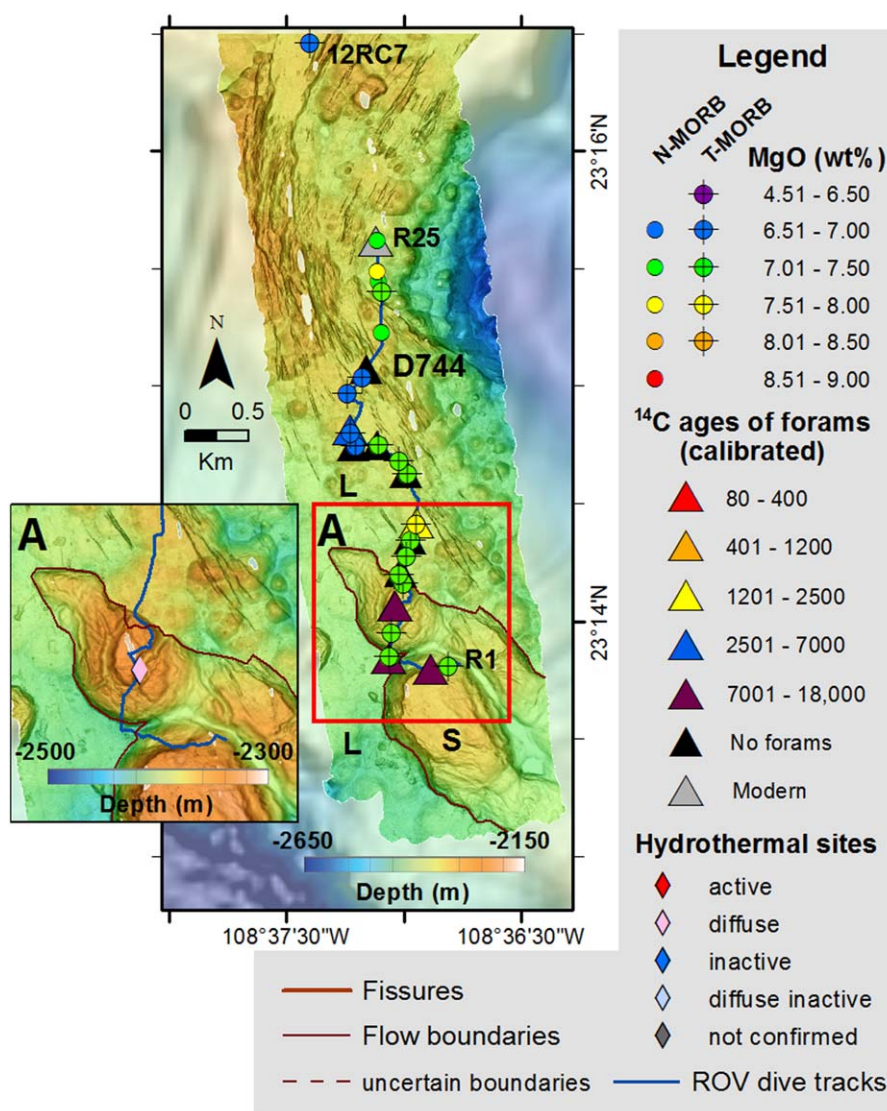
Figure 3. TT map with ROV dive D744 track, lava samples from dive (with first and last rock samples labeled as R1 and R25) and wax-tip rock core 12RC7 color coded by MgO content and with different symbols for N-MORB and T-MORB. Push cores are color coded by radiocarbon age of basal slice. The legend defines symbols used in all subsequent maps except Figures 10 and 19, which also divide the lavas by lithology. Inset A, indicated by red box, shows the location of a low-temperature hydrothermal seep site on a sediment hill. This hydrothermal site was not identified in the AUV bathymetry. Lava flows (L) cover the seafloor west and north of the flow boundary line whereas thick sediment (S) characterizes the seafloor in the southeast portion of the map.
