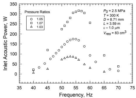
Figure 7. Inlet acoustic power vs. frequency for a reservoir volume of 83 cm 3
