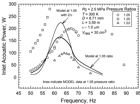
Figure 6. Inlet acoustic power vs. frequency for a reservoir volume of 30 cm 3
