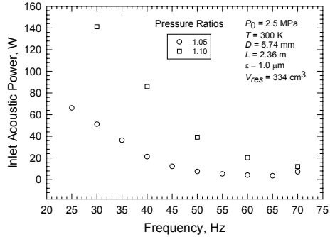
Figure 5. Inlet acoustic power vs. frequency for a reservoir volume of 334 cm 3
