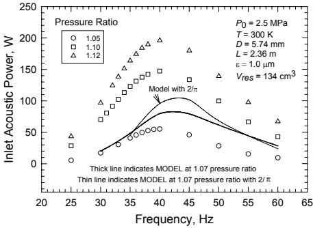
Figure 4. Inlet acoustic power vs. frequency for a reservoir volume of 134 cm 3
