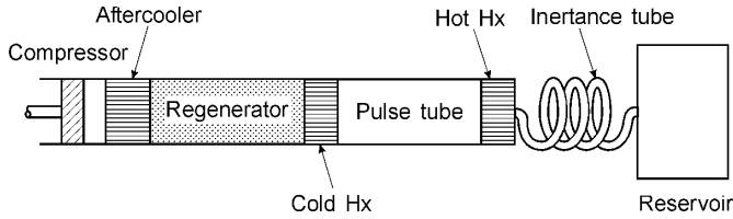
Figure 1. Schematic of pulse tube cryocooler with inductance tube.
