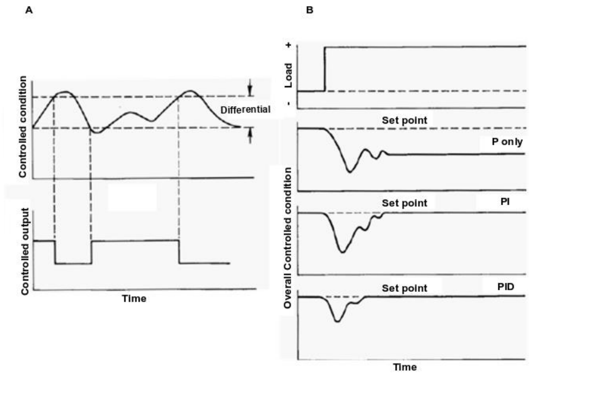
Figure 2.1. Simple schematic of A) On/Off controller and B) P, PI, and PID controller [25].
