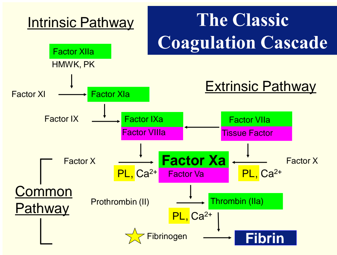
Figure 2: The classic coagulation cascade. In green are serine proteases, magenta are cofactors. PL represents negatively charged phospholipids and Ca 2+ represents calcium, both of which are required for assembling complexes containing \gamma -carboxyglutamic acid (GLA)-domain proteins on the membrane. Star indicates terminal glycoprotein fibrinogen that polymerizes to insoluble fibrin once cleaved by thrombin.
