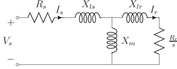
Figure 2.1 Single-Cage Induction Machine Steady State Equivalent Circuit
