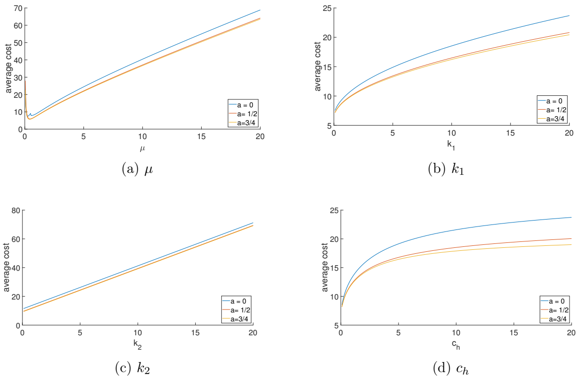
Figure 3.2.: Sensitivity analysis of the average cost in a drifted Brownian motion inventory model with uniformly distributed supply for different model parameters ( \mu = 3 , \sigma = 1 , k_1 = 8 , k_2 = 2 , c_h = 3 , c_b = 4 , if not variable)
