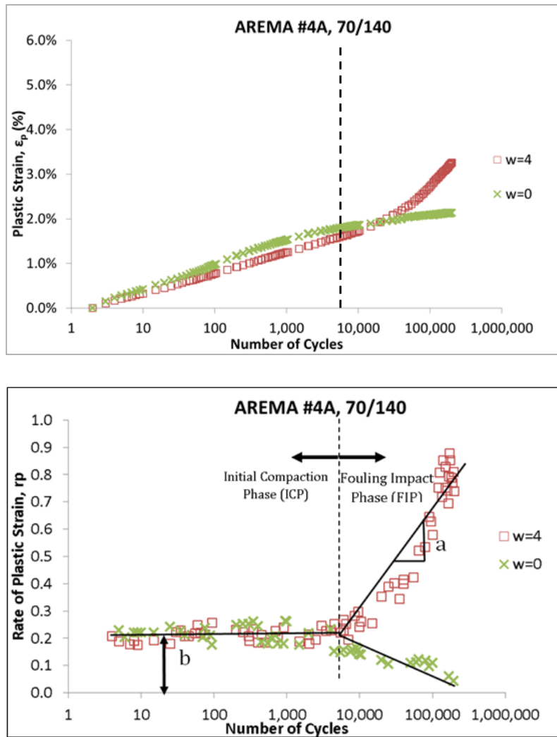
Figure 5.1.14 WiscRail model parameters 'a' and 'b' for sample data. These parameters will vary for changing ballast type, fouling type, fouling content, and moisture content.
