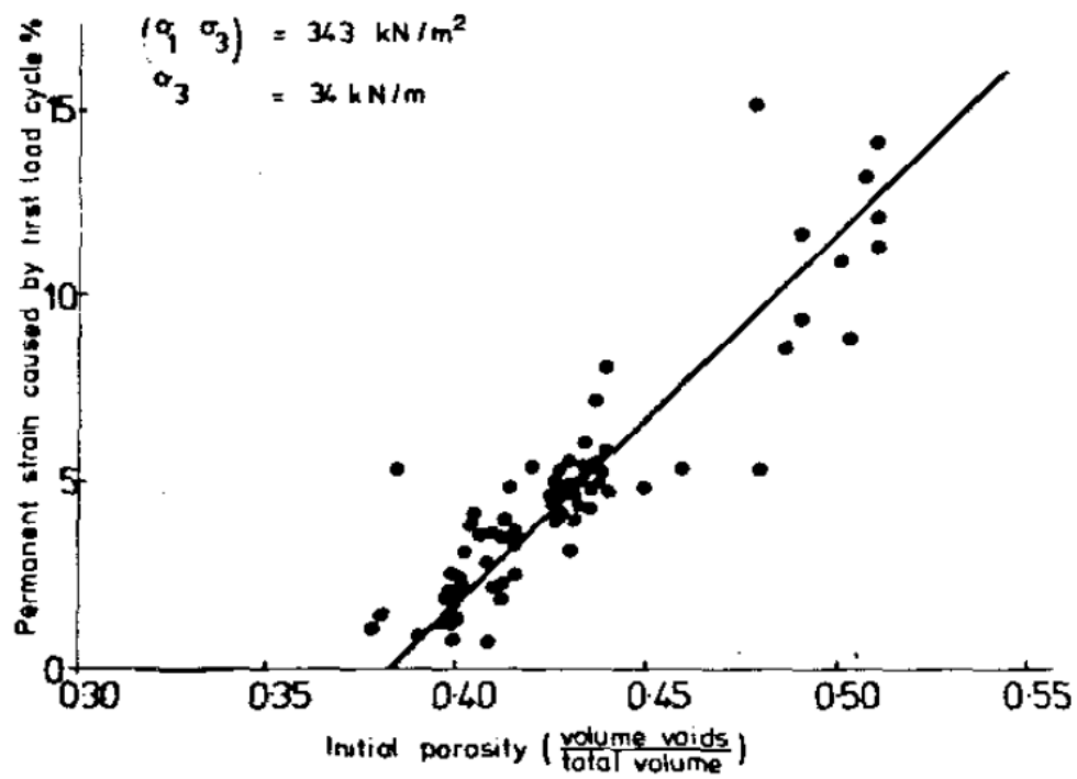
Figure 2.16 Diagram showing first cycle plastic strain variation as a function of porosity (Shenton 1975).
