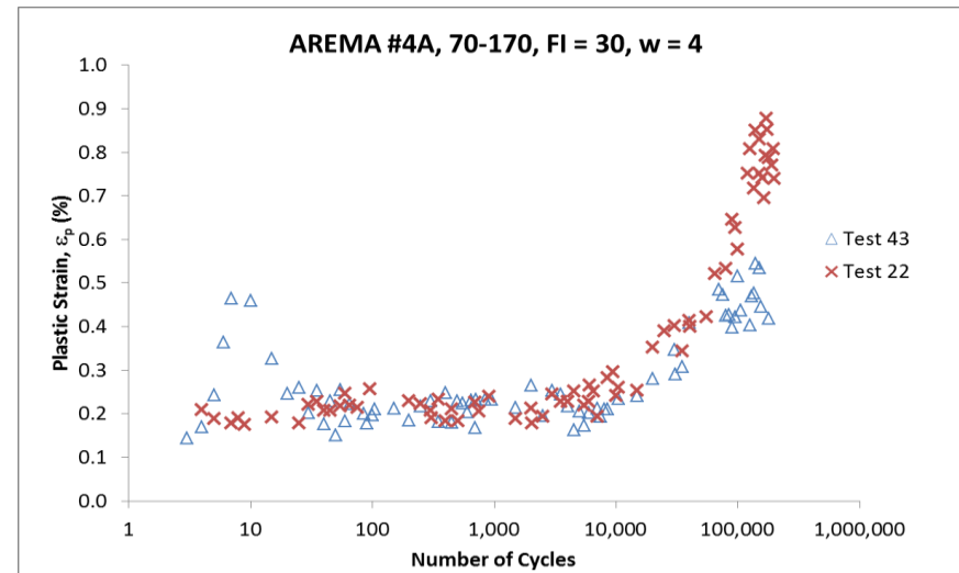
Figure 0.6 Accumulation of plastic strain and rate of plastic strain for repeated tests #43 & #22, under 2 \times 10^5 loading cycles.
