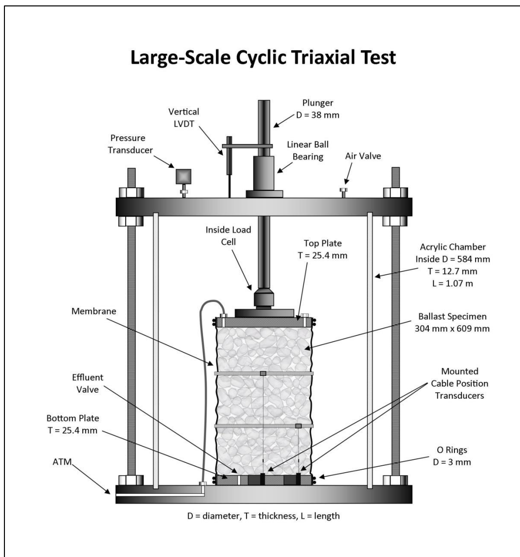
Figure 0.1 Large-Scale Cyclic Triaxial (LSCT) Setup Diagram.
