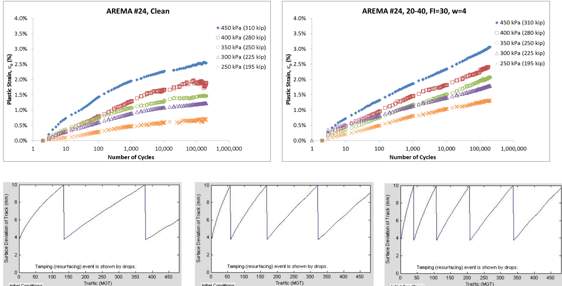
Figure 5.1.17 WiscRail™ model results for HAL with 225, 280, and 310 kip graphs represented.
