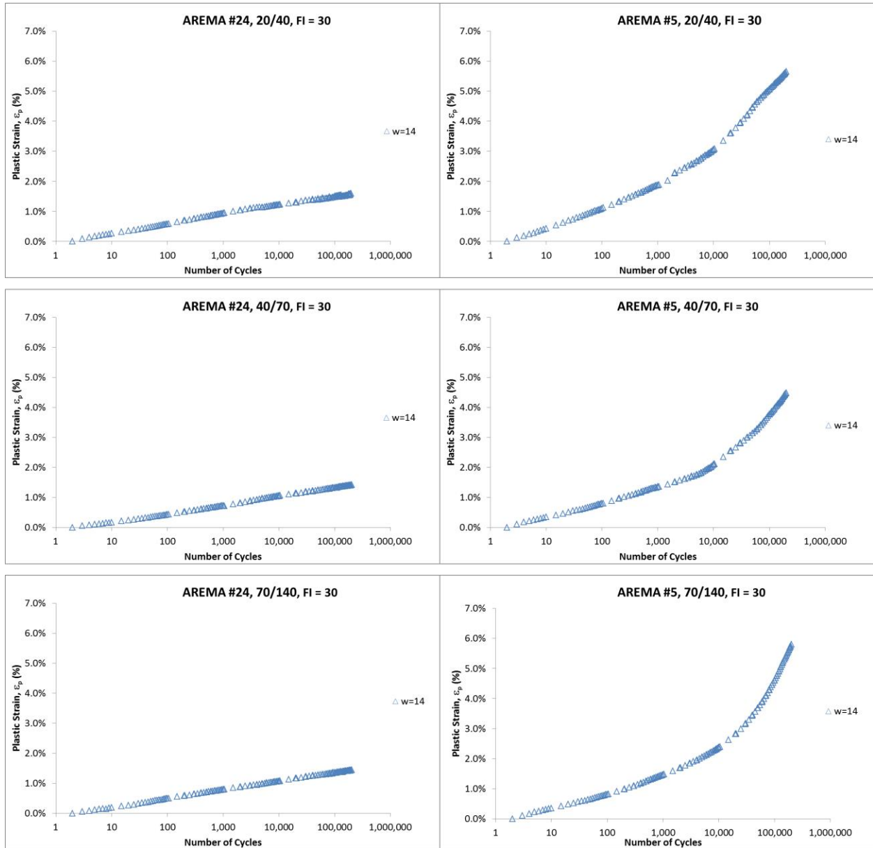
Figure 5.1.6 Cumulative plastic strain, comparison of sand gradation from 20/40 to 70/140 (top to bottom) in AREMA #24 and AREMA #5 ballast (left to right).
