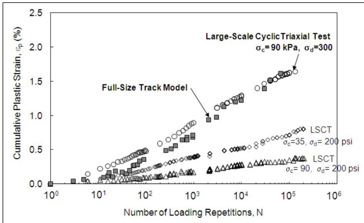
Figure 2.3 Full-Scale Track Model and Large-Scale Cyclic Triaxial Model comparison used by Ebrahimi (2011).
