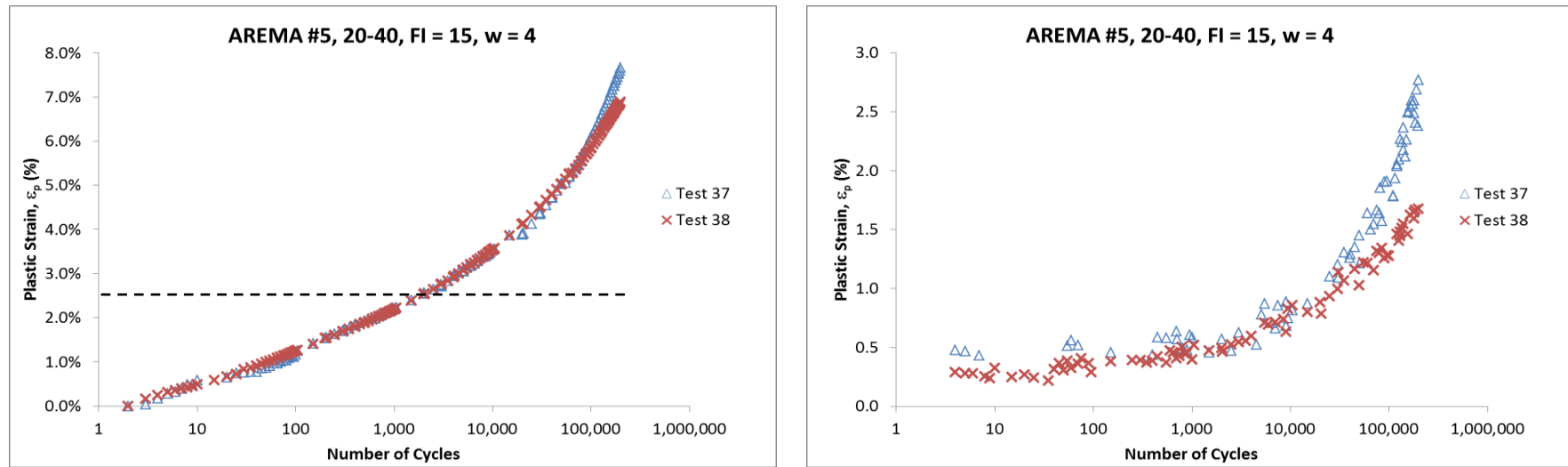
Figure 0.7 Accumulation of plastic strain and rate of plastic strain for repeated tests #37 & #38, under 2 \times 10^5 loading cycles.
