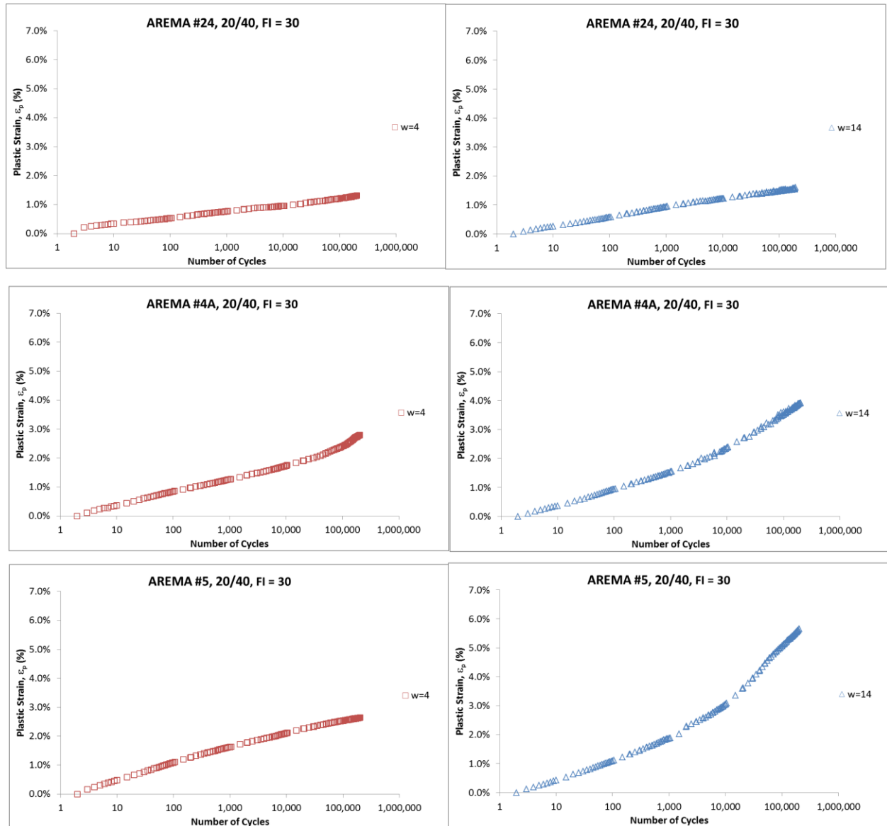
Figure 5.1.1 Cumulative plastic strain, comparison of water content for the same ballast and frac sand at w = 4, 14 (left to right).
