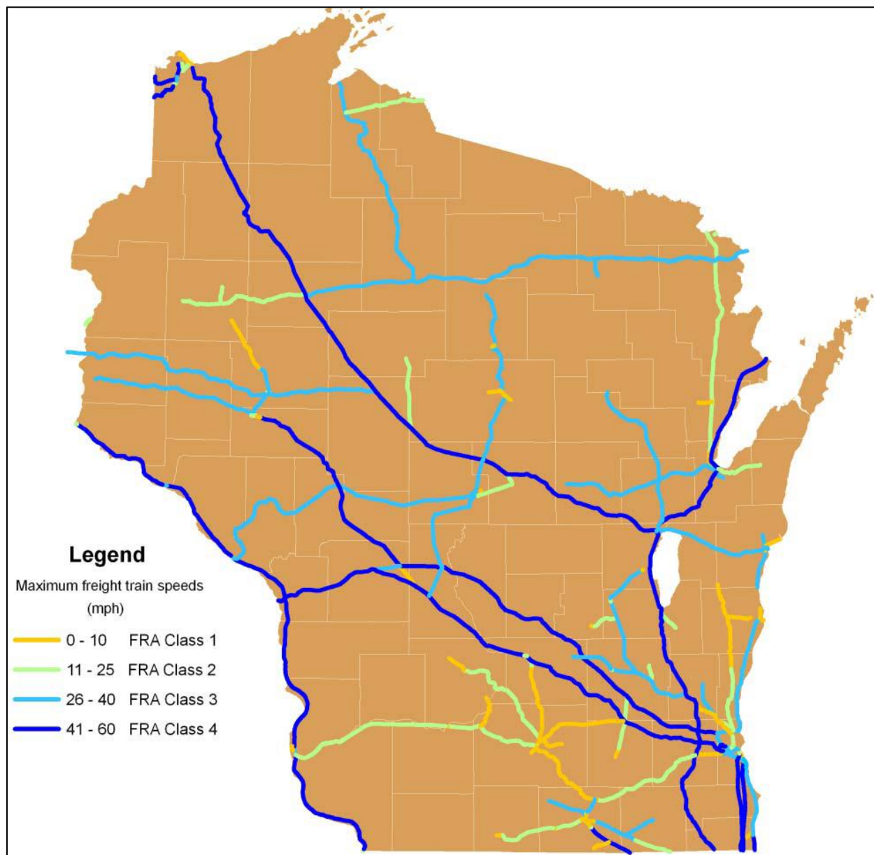
Figure 0.3 Maximum allowable train speeds on Wisconsin Railways (Wisconsin DOT 2010).
