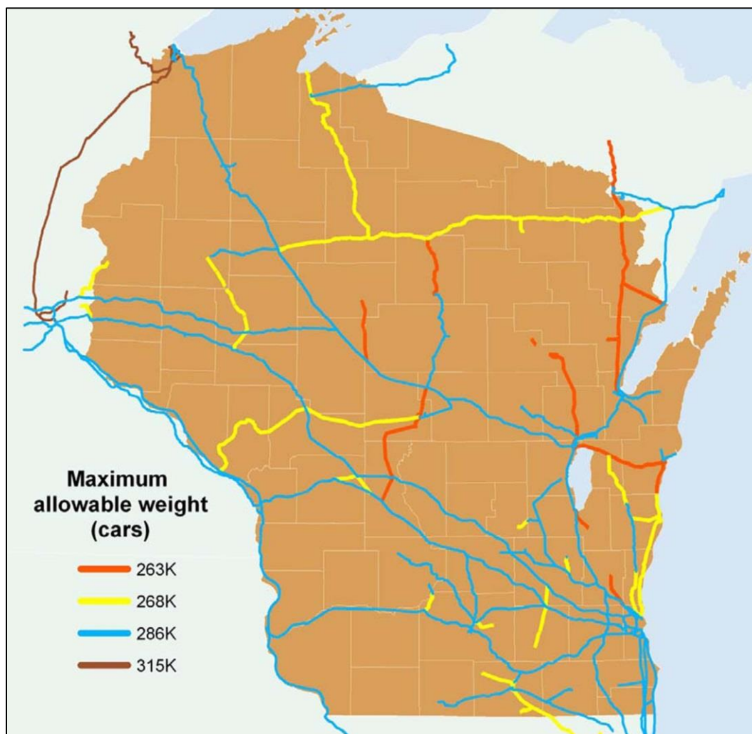
Figure 2.9 Wisconsin's maximum allowable weight (in thousands of pounds) for freight rail cars (Wisconsin DOT 2010).
