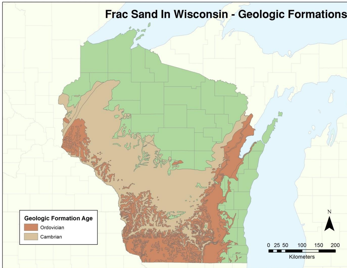
Figure 1.2 Wisconsin Geologic Formations.
