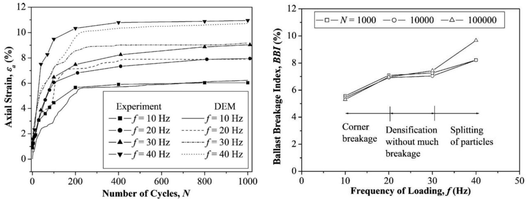
Figure 2.14 Effect of frequency on ballast deformation and ballast breakage (Indraratna et al. 2010).
