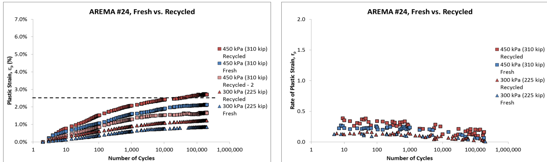
Figure 5.1.11 Comparison of fresh versus recycled for AREMA #24 ballast, FI = 0, w = 0, and \sigma_d = 300 kPa, 450 kPa
