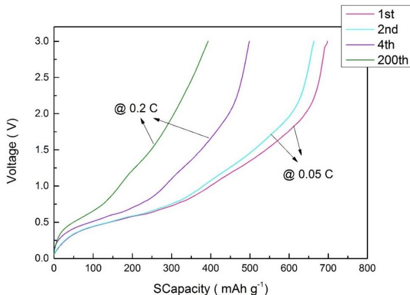
Figure 25 Charge Curve of the 1 st , 2 nd , 4 th and 200 th cycles.
