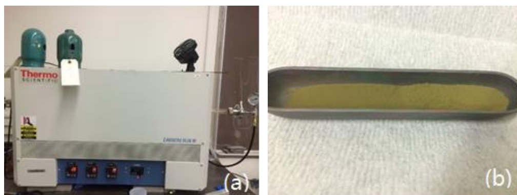
Figure 9(a). Vacuum tube oven. (b). Earthy yellow powder obtained after reduction.
