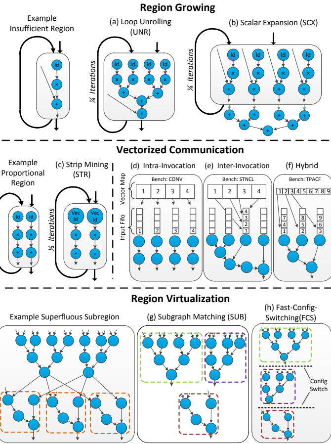
Figure 3: Overview of Hardware and Software Transformations for Parallelism Specialization
