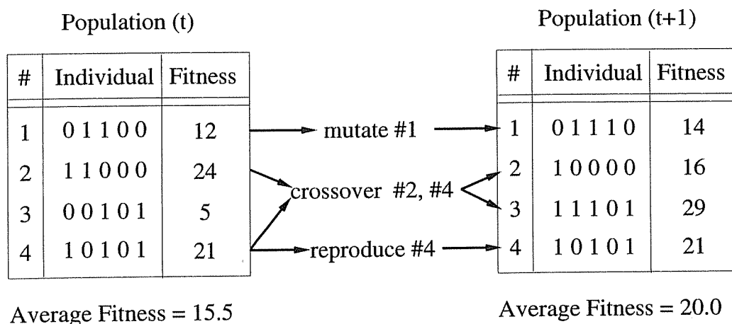
Figure 16: An example of one generation in a standard GA. A population of four individuals is reproduced, through fitness-proportional reproduction, to create another population of four individuals.
