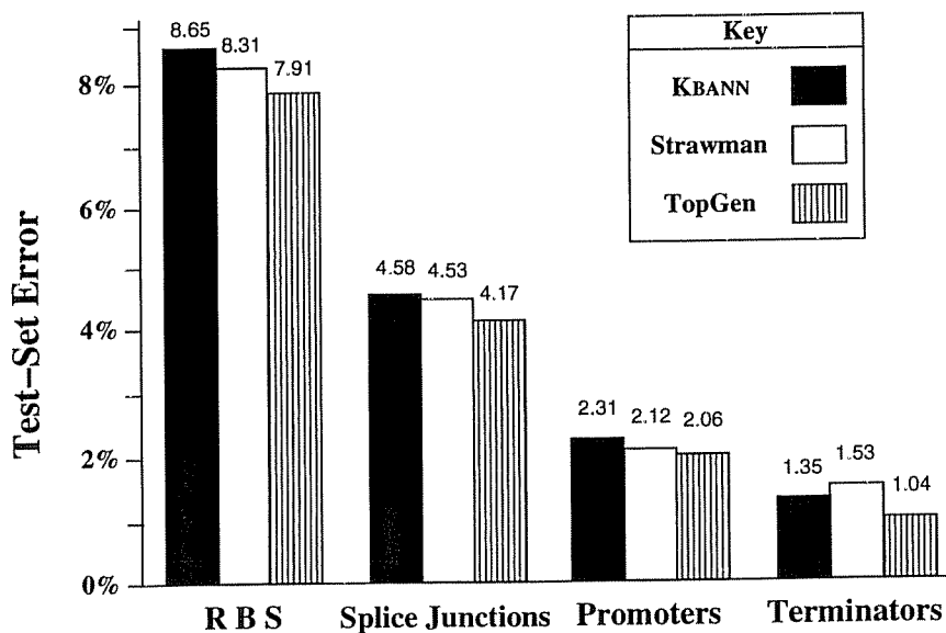
Figure 14: Error rates on four Human Genome problems.
