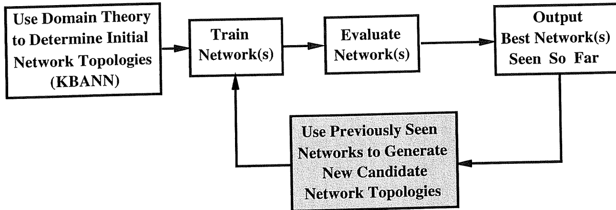
Figure 2: Framework for the learning algorithms I introduce in this thesis.
