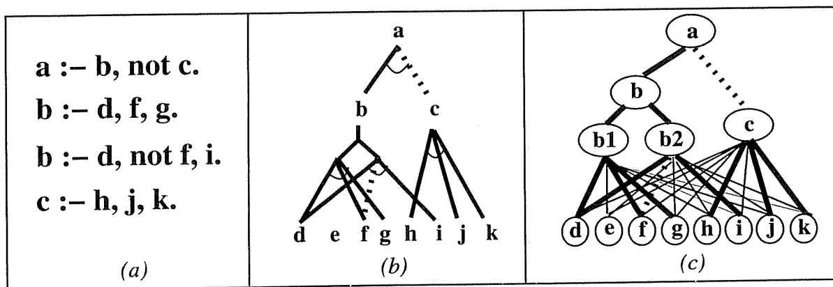
Figure 10: KBANN's translation of a knowledge base into a neural network. Panel (a) shows a sample propositional rule domain theory in Prolog (Clocksin & Mellish, 1987) notation, panel (b) illustrates this rule set's corresponding dependency tree, and panel (c) shows the resulting network created from KBANN's translation. (This is a repeat of Figure 6 in Section 2.2.1.)
