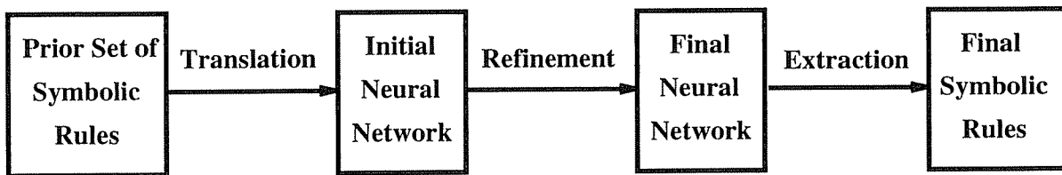
Figure 5: One approach for combining symbolic and neural learning.
