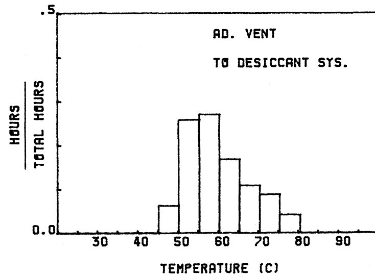
Figure 6.4.3 Distribution of temperatures sent to the solar system and returned to the desiccant system for the cooled Dunkle and adiabatic vent cycles.
