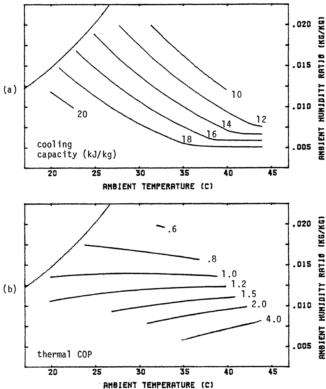
Figure B.3 Adiabatic Dunkle cycle system performance maps.
