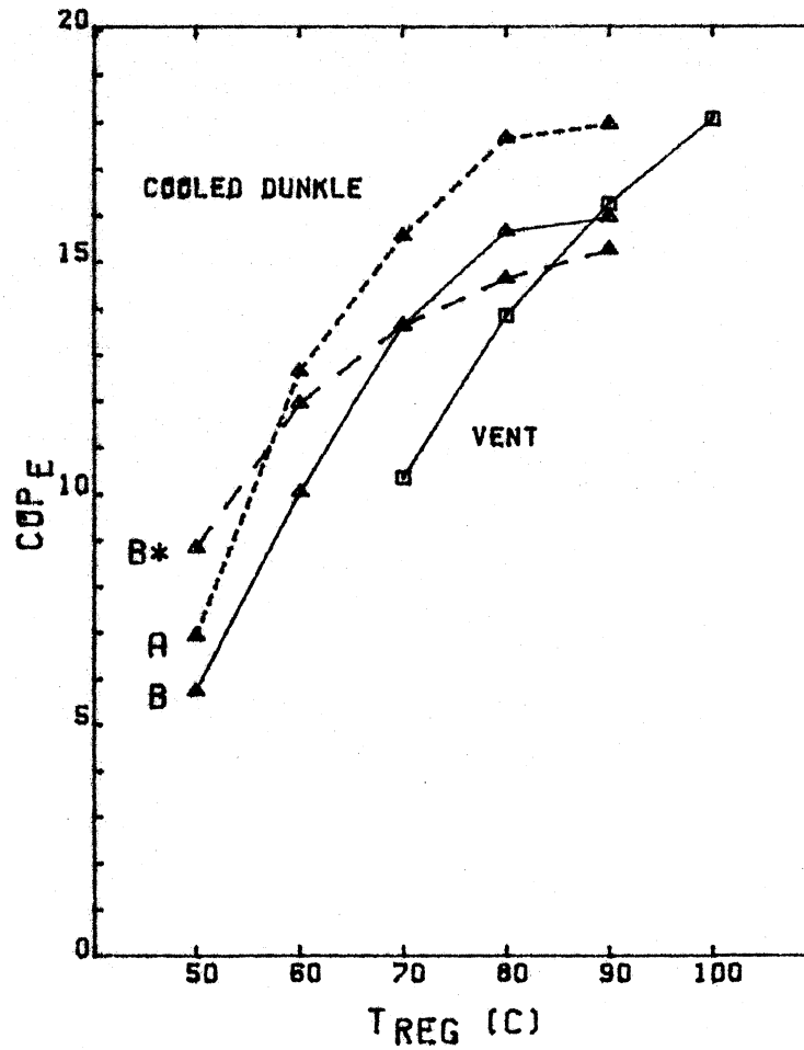
Figure 6.4.1 Performance of the gas-fired cooled Dunkle cycle in Miami, FL, for the months of June, July, and August. (a) thermal COP. (b) electric COP.
