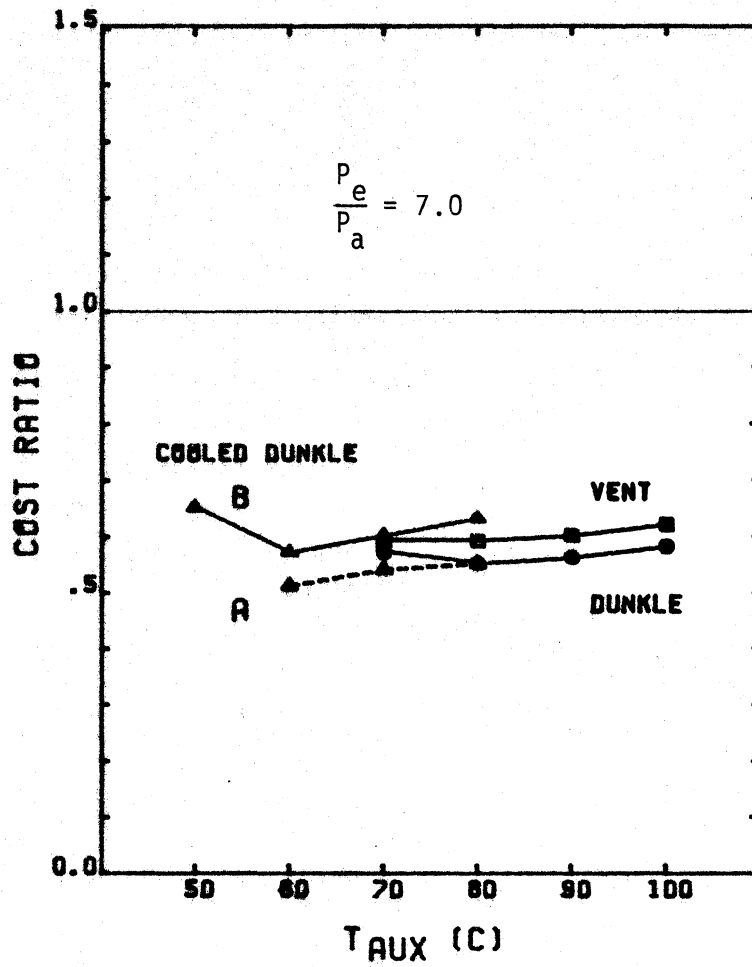
Figure 6.4.5 (cont) Phoenix, solar-fired. (e) & (f) cost ratios.
