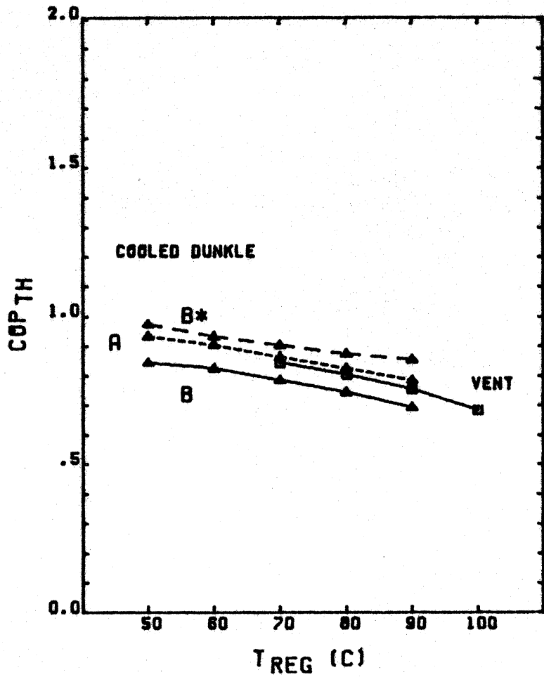
Figure 6.4.6 Performance of gas-fired cooled Dunkle cycle in Columbia, MO, for the months of June, July, and August. (a) thermal COP. (b) electric COP.
