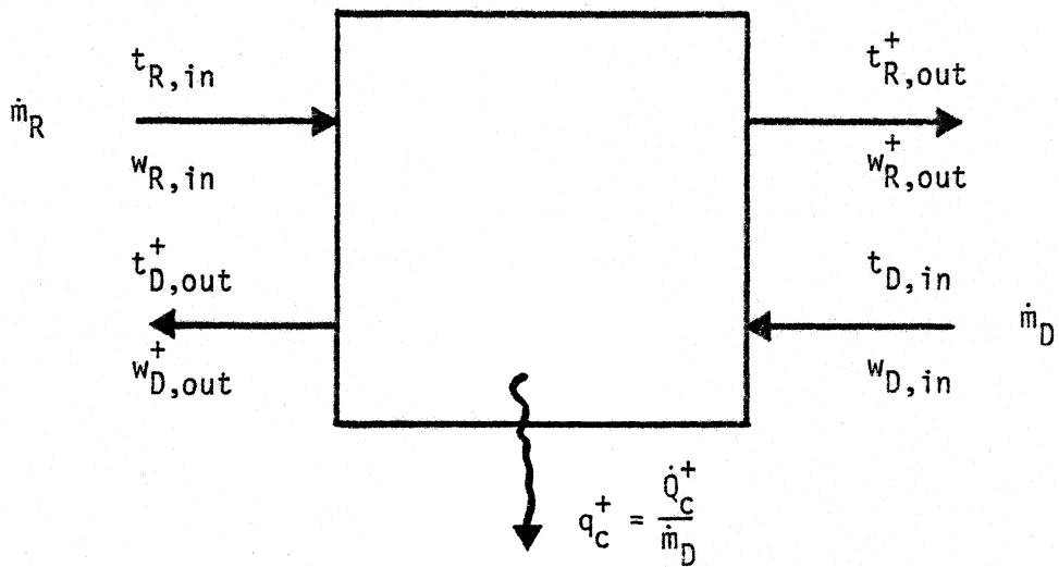
Figure 4.2.9 Wave diagram and control volume for idealized cooled dehumidifier cycle with a flow ratio greater than (\dot{m}_R/\dot{m}_D)^* .
