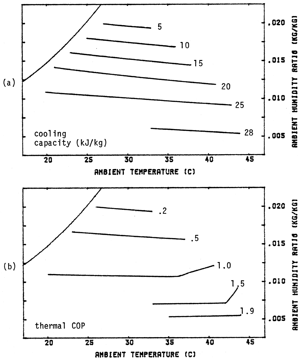
Figure B.2 Cooled ventilation cycle system performance maps.
