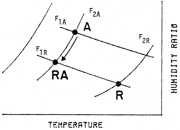
Figure 4.2.3 Wave diagram and psychrometric representation of idealized (adiabatic) dehumidification process in cooled dehumidifier cycle.
