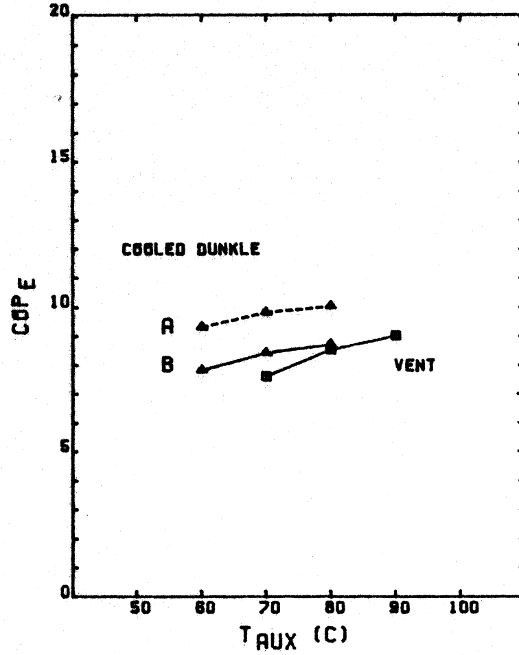
Figure 6.4.7 (cont) Columbia, solar-fired. (c) purchased thermal energy COP. (d) electric COP.
