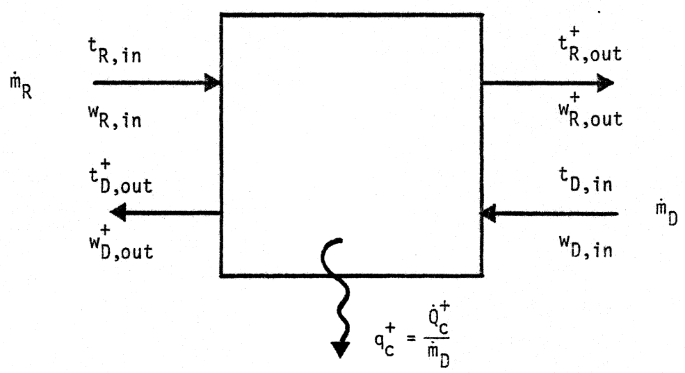
Figure 4.2.10 Wave diagram and control volume for idealized cooled dehumidifier cycle with a flow ratio less than (\dot{m}_R/\dot{m}_D)^* .
