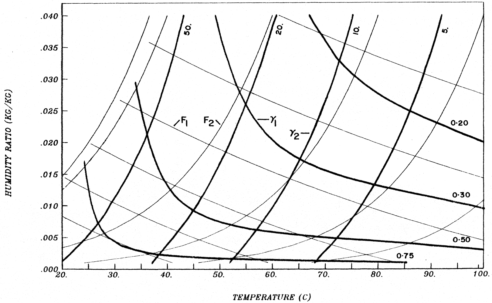
Figure 3.1.3 \gamma_1 and \gamma_2 superimposed on F_1 and F_2 for moist air-silica gel (from ref[7]).
