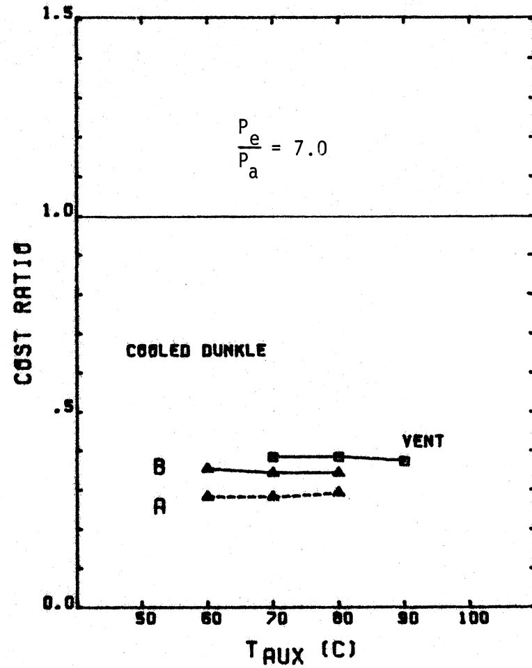
Figure 6.4.7 (cont) Columbia, solar-fired. (e) & (f) cost ratios.
