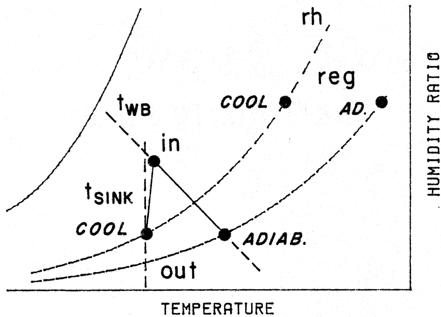
Figure 2.3.3 Regeneration temperatures required to obtain same outlet humidity ratio from cooled and adiabatic dehumidifiers.
