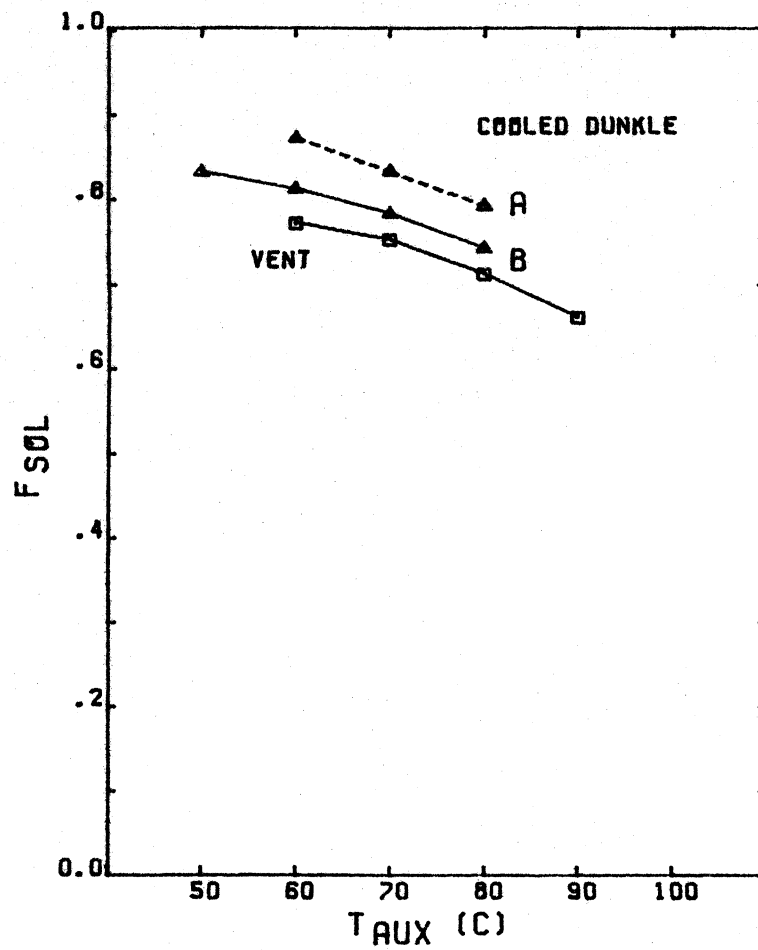
Figure 6.4.2 Performance of solar-fired cooled Dunkle cycle in Miami, FL for month of July. (a) thermal COP. (b) fraction of thermal energy supplied by solar.
