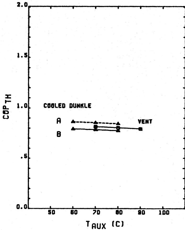
Figure 6.4.7 Performance of solar-fired cooled Dunkle cycle in Columbia, MO, for the month of July. (a) thermal COP. (b) fraction of thermal energy supplied by solar.
