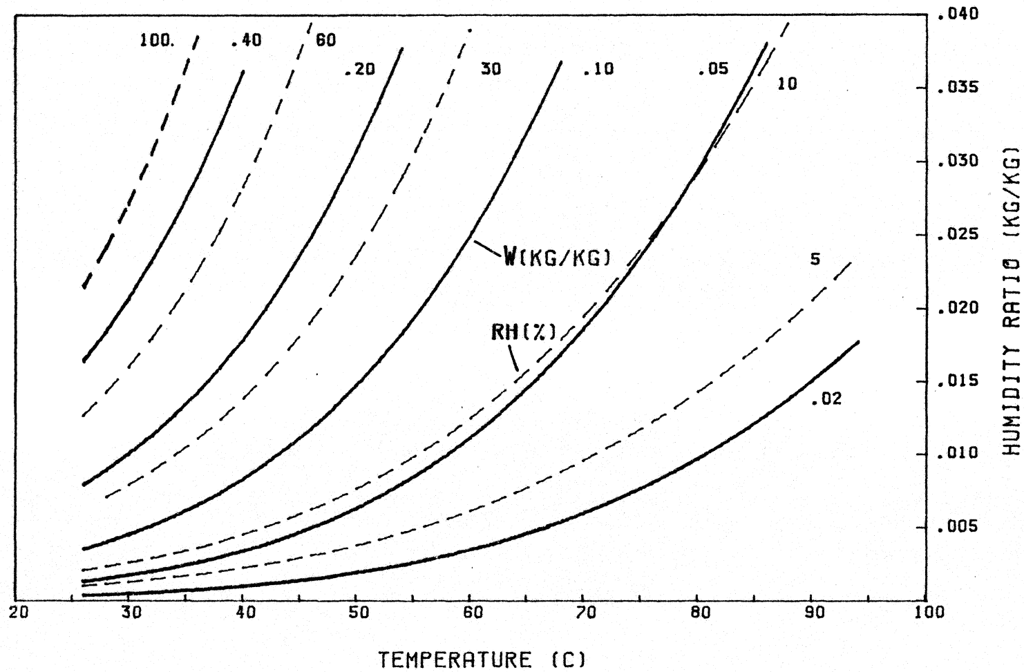
Figure 2.6.1 Psychrometric diagram of silica gel water content and relative humidity.
