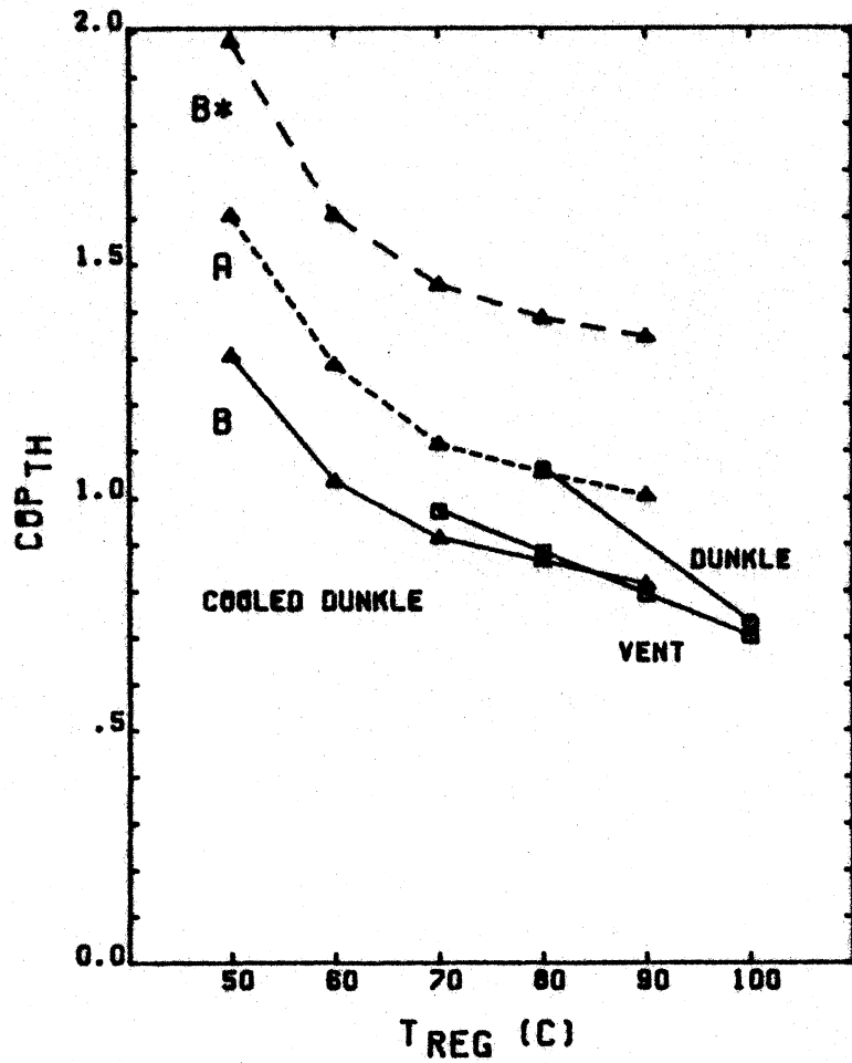
Figure 6.4.4 Performance of gas-fired cooled Dunkle cycle in Phoenix, AZ, for the months of June, July, and August. (a) thermal COP. (b) electric COP.
