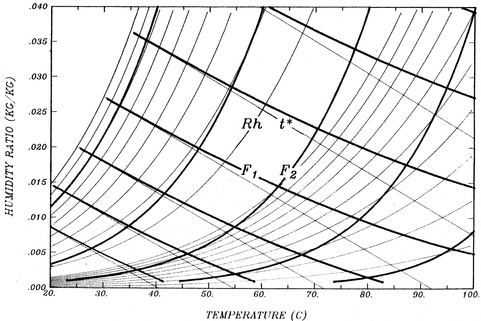
Figure 3.1.2 Characteristic potentials F_1 and F_2 for moist air-silica gel superimposed on wet bulb temperature ( t^* ) and relative humidity lines ( Rh ) (from ref [7]).
