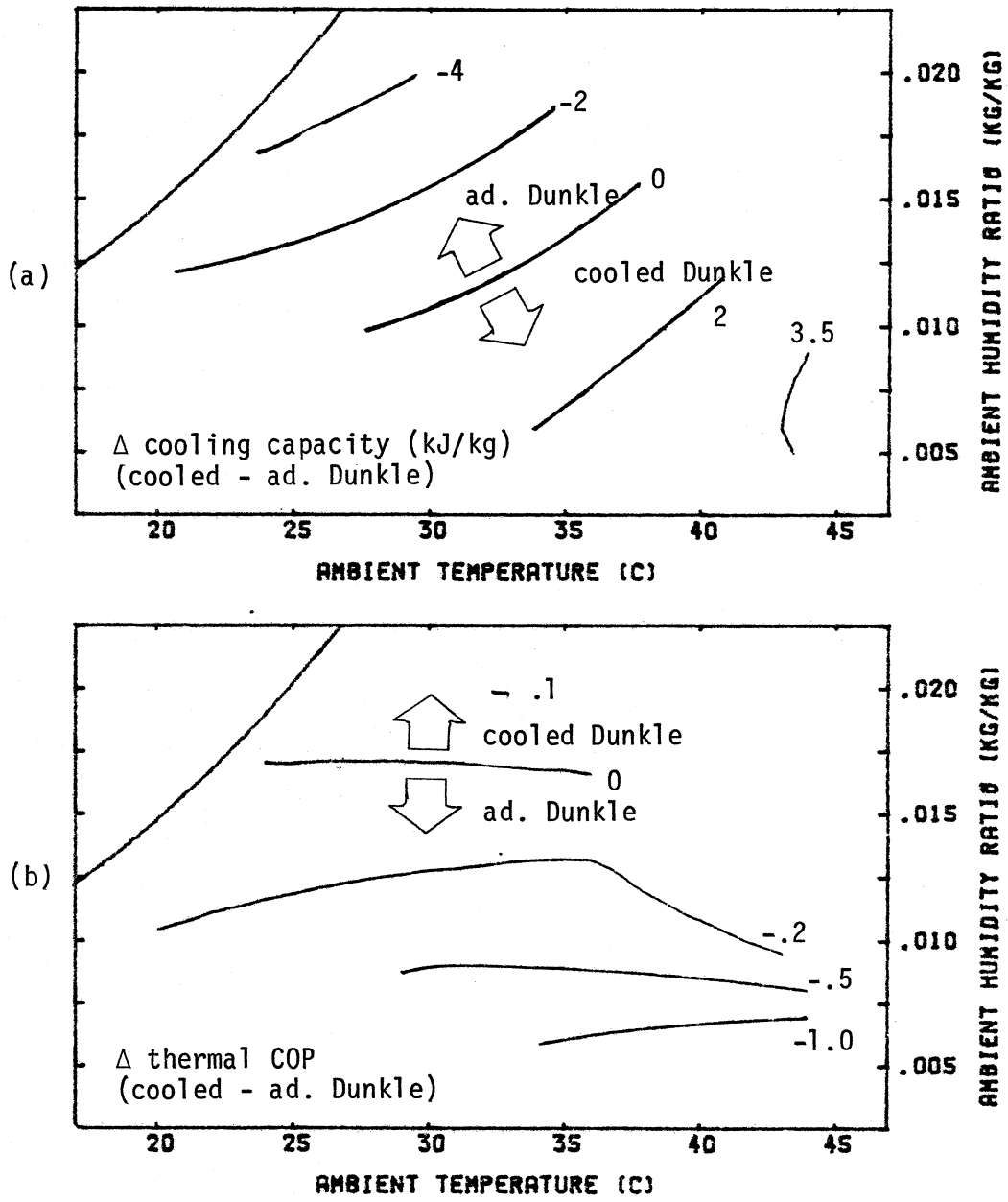
Figure 5.5.1 Difference between performance of cooled Dunkle ( T_{REG} = 55^{\circ}C ) and adiabatic Dunkle ( T_{REG} = 70^{\circ}C ) cycles. (a) cooling capacity. (b) thermal COP.
