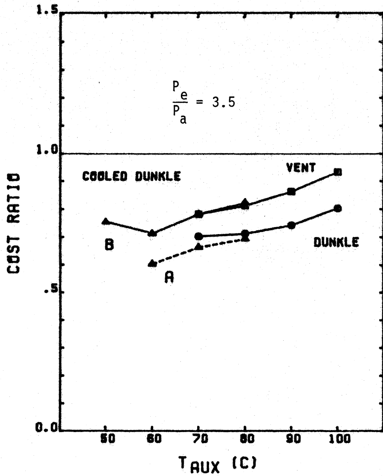
Figure 6.4.5 (cont) Phoenix, solar-fired. (e) & (f) cost ratios.
