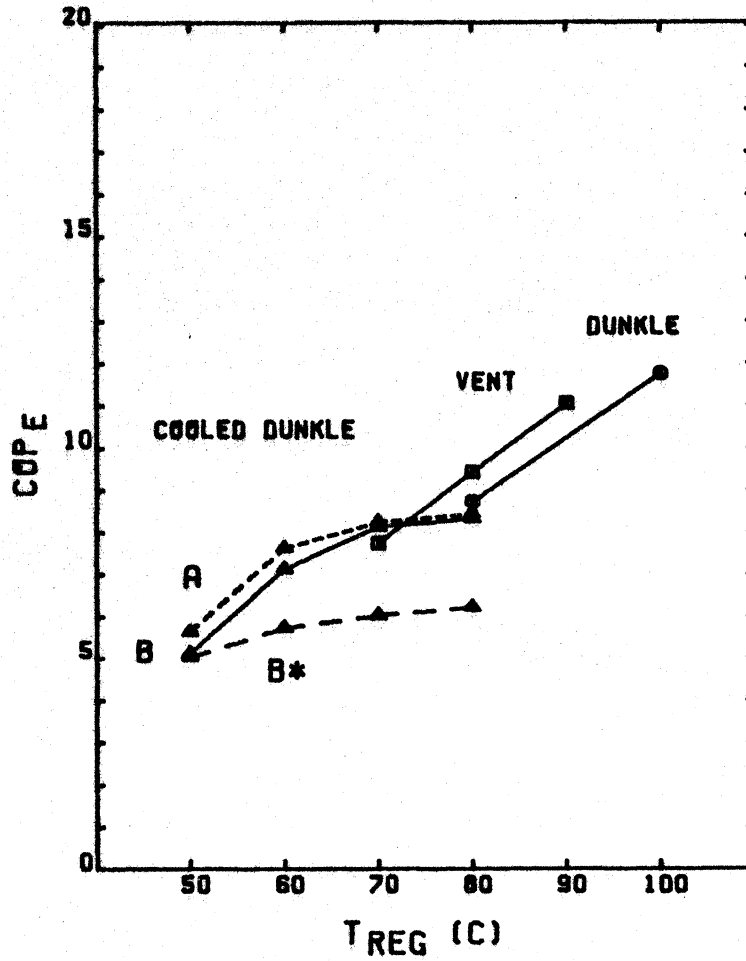
Figure 6.4.4 Performance of gas-fired cooled Dunkle cycle in Phoenix, AZ, for the months of June, July, and August. (a) thermal COP. (b) electric COP.
