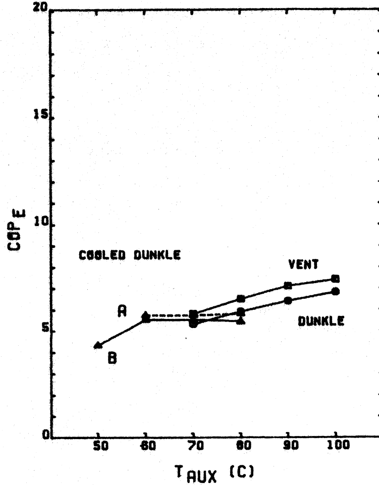
Figure 6.4.5 (cont) Phoenix, solar-fired. (c) purchased thermal energy COP. (d) electric COP.
