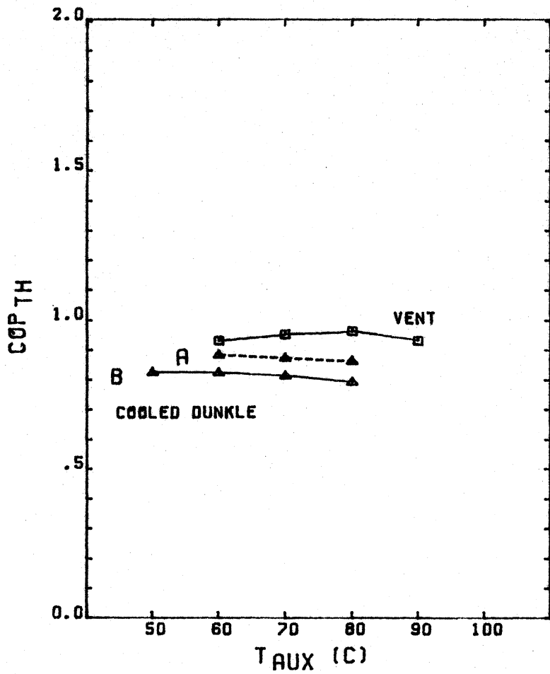
Figure 6.4.2 Performance of solar-fired cooled Dunkle cycle in Miami, FL for month of July. (a) thermal COP. (b) fraction of thermal energy supplied by solar.
