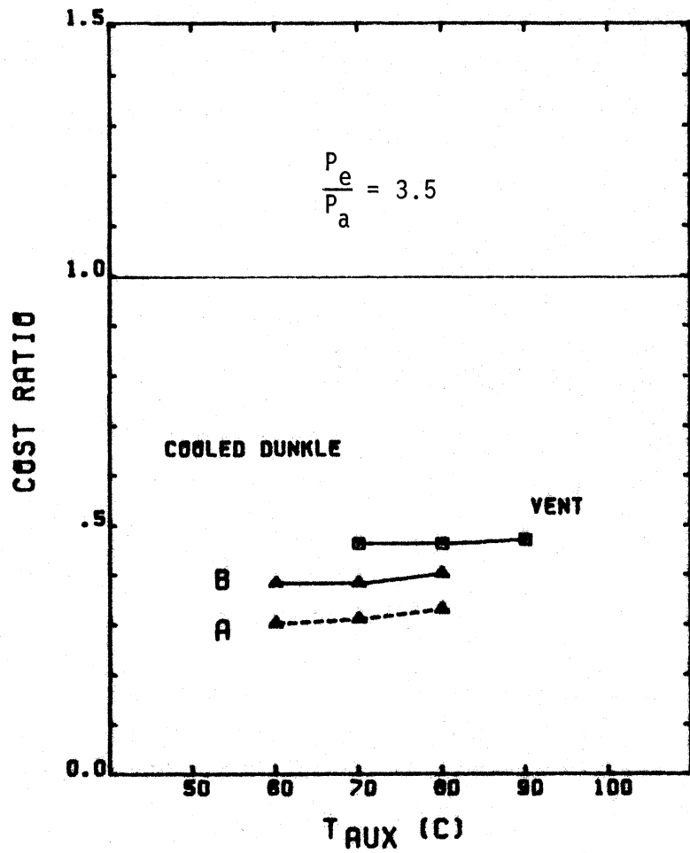
Figure 6.4.7 (cont) Columbia, solar-fired. (e) & (f) cost ratios.
