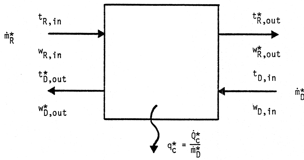
Figure 4.2.7 Control volume and air states for idealized cooled dehumidifier with flowrates set for maximum dehumidification and regeneration.
