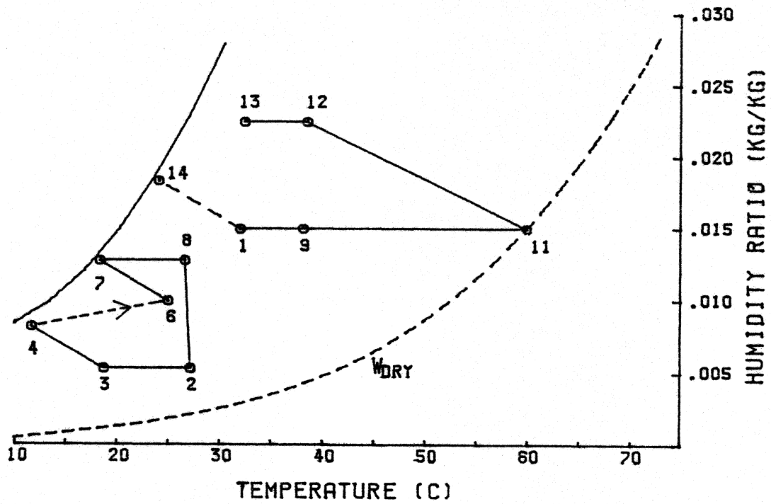
Figure 2.4.1 Cooled Dunkle cycle cooling system.
