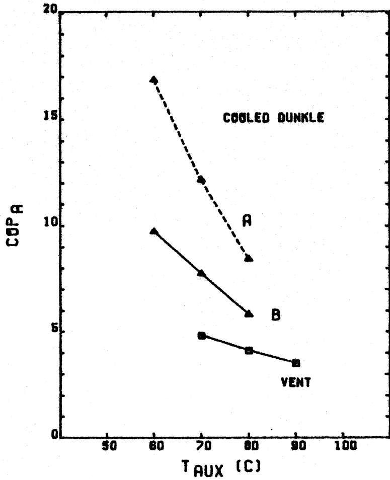
Figure 6.4.7 (cont) Columbia, solar-fired. (c) purchased thermal energy COP. (d) electric COP.
