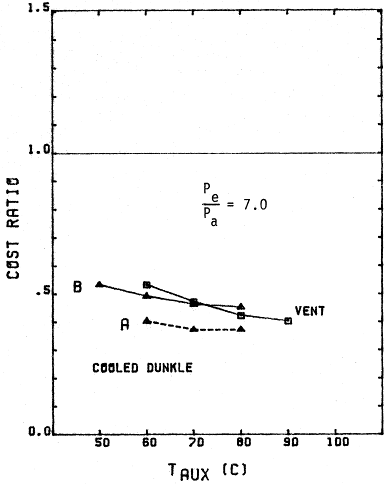
Figure 6.4.2 (cont) Miami, solar-fired. (e) & (f) cost ratios.
