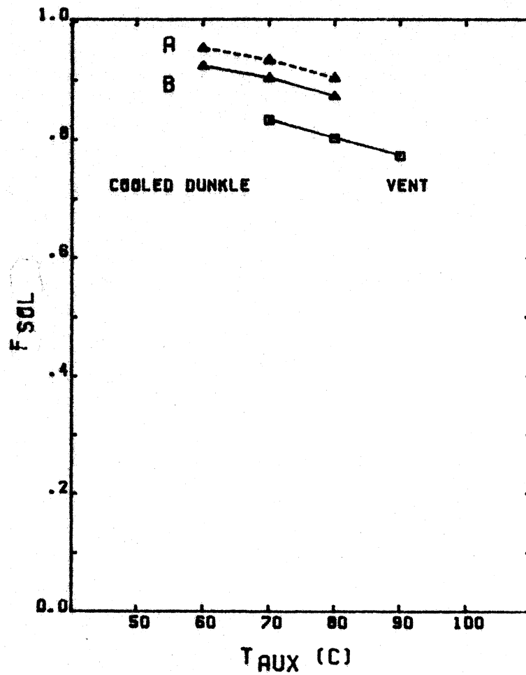
Figure 6.4.7 Performance of solar-fired cooled Dunkle cycle in Columbia, MO, for the month of July. (a) thermal COP. (b) fraction of thermal energy supplied by solar.
