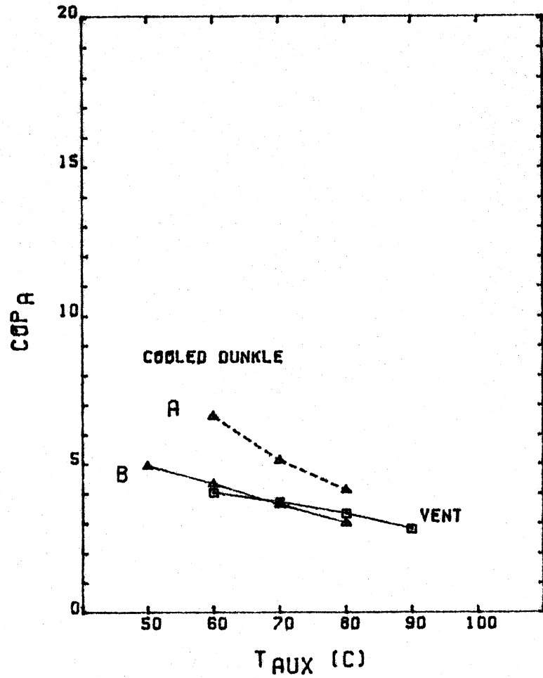
Figure 6.4.2 (cont) Miami, solar-fired. (c) purchased thermal energy COP. (d) electric COP.
