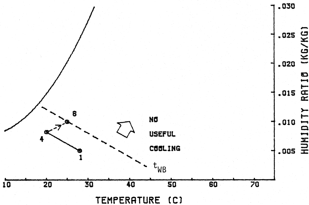
Figure 2.1.1 Simple evaporative cooling system.
