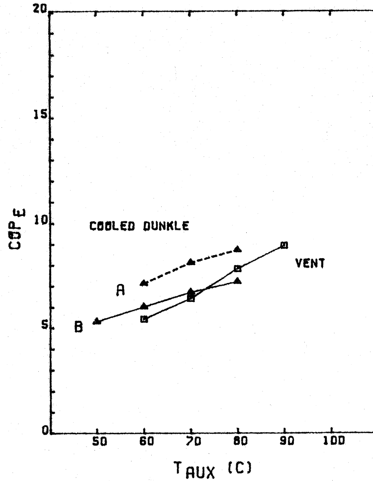
Figure 6.4.2 (cont) Miami, solar-fired. (c) purchased thermal energy COP. (d) electric COP.
