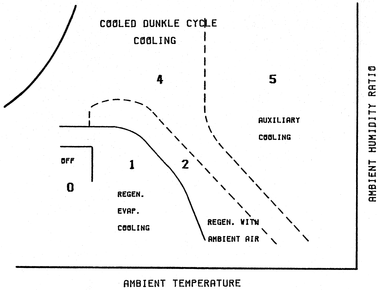
Figure 6.1.2 Effects of ambient condition on mode of operation of the cooled Dunkle cycle.
