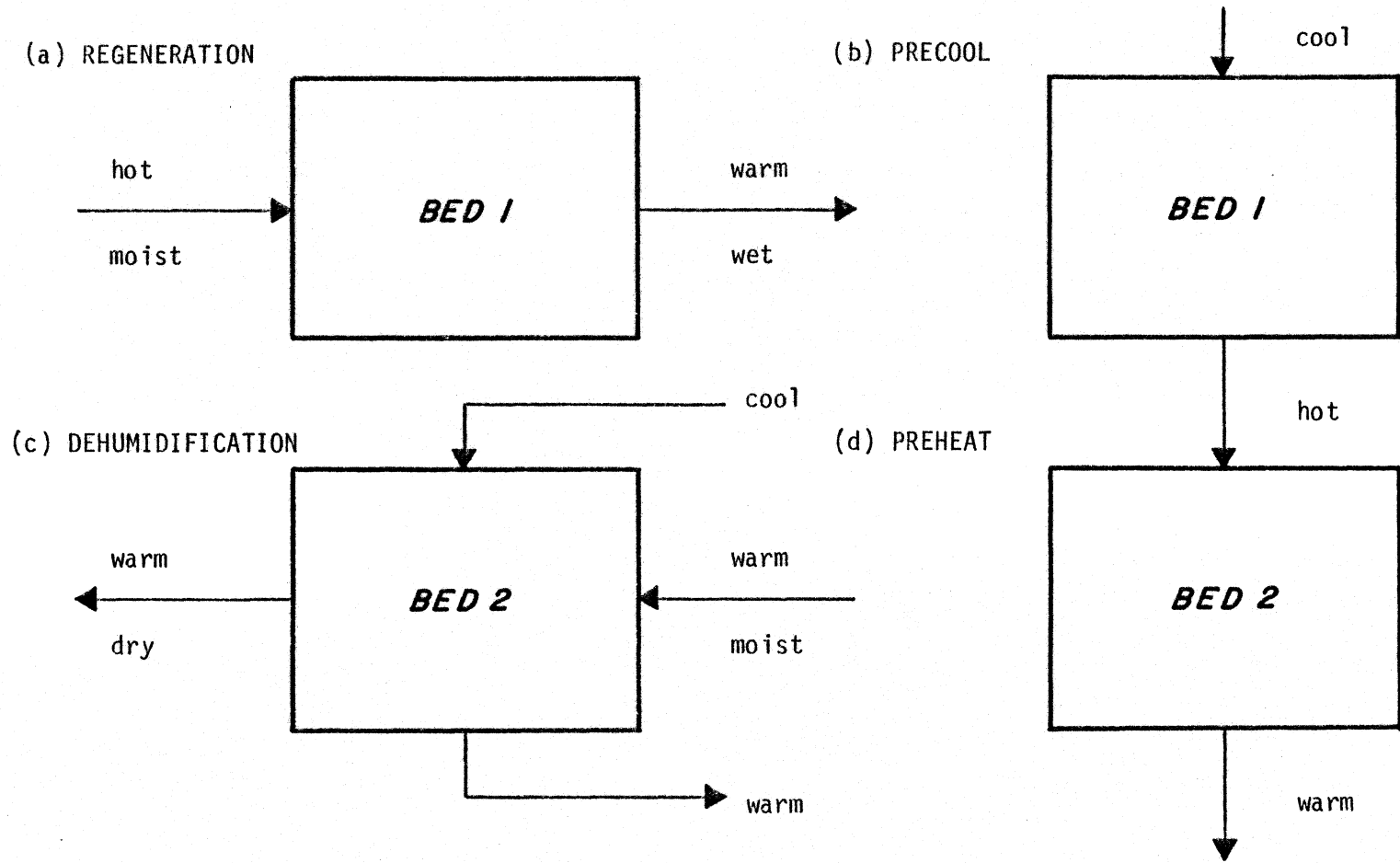
Figure 4.1.2 Cooled dehumidifier cycle.
