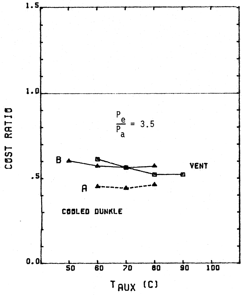
Figure 6.4.2 (cont) Miami, solar-fired. (e) & (f) cost ratios.
