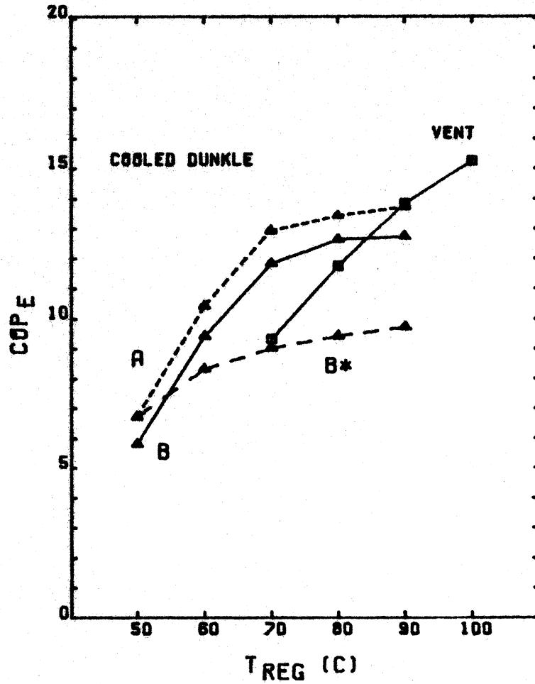
Figure 6.4.6 Performance of gas-fired cooled Dunkle cycle in Columbia, MO, for the months of June, July, and August. (a) thermal COP. (b) electric COP.
