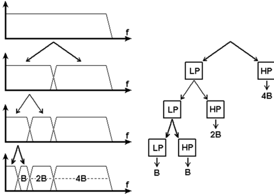
Figure 3-3 Frequency Bands Separation and multi-resolution analysis (MRA)
