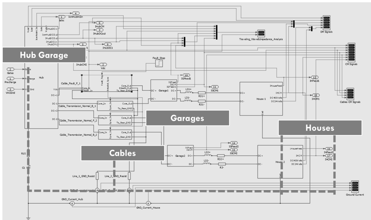
Figure 4-14 The Ground Fault Current Paths in the Model
