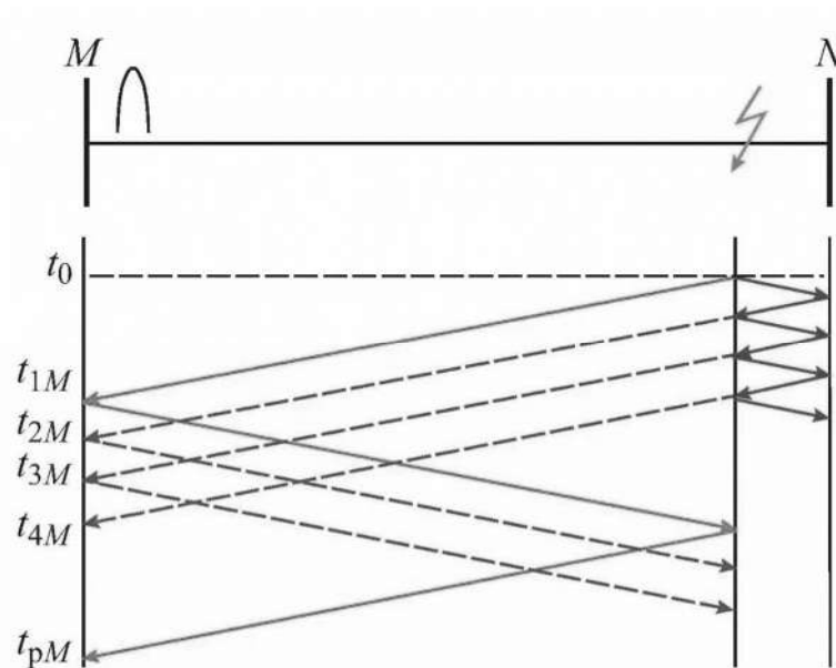
Figure 1-5 The Reflection of Traveling Wave when Fault Happens in Cable
