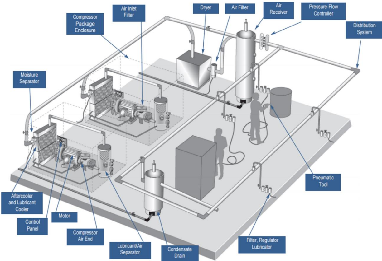
Figure 5 Typical Compressed Air System [25]
