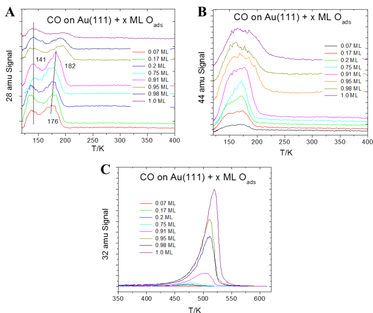
Figure 7.3.2.3: TPD profiles [(A) 28, (B) 44, and (C) 32 amu] of 10L CO adsorbed at 80K on a surface with various coverages of atomic oxygen collected using a heating rate of 3.4 K/s as a function of CO exposure.
