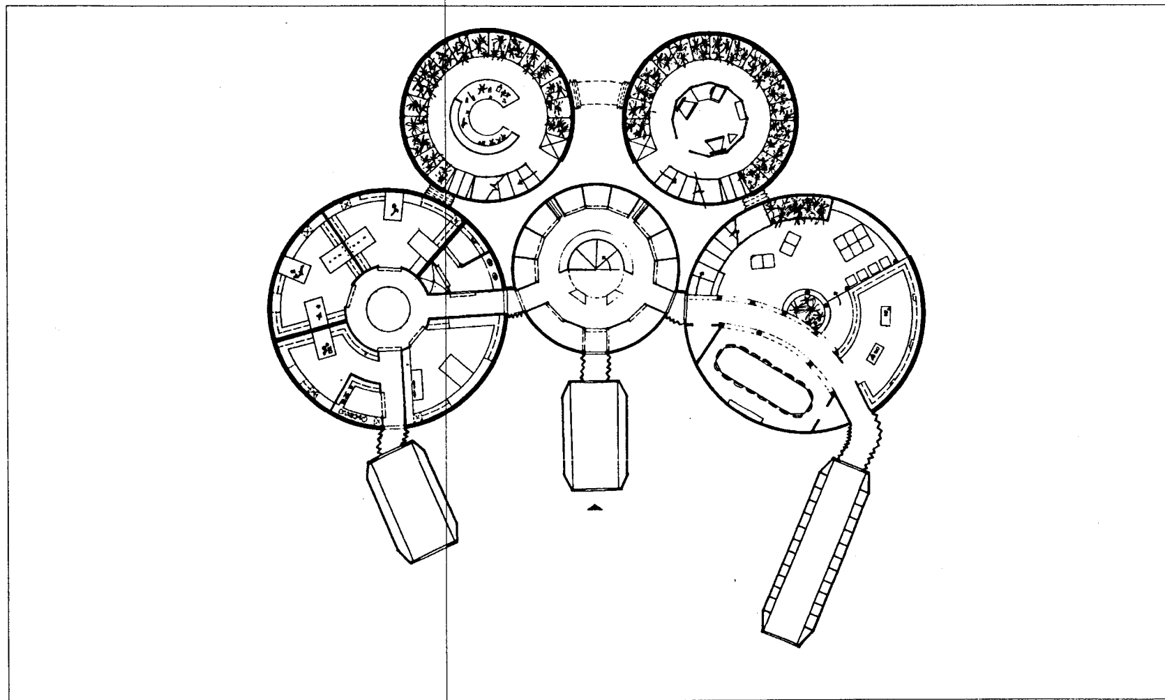
Figure 4.5.1.1-1. Floor plan of the habitat, level one. Three smaller modules contain the entry space and the greenhouse facilities. The two larger modules support the crew and laboratory functions. A logistics module and two airlocks complete the habitat plan.
