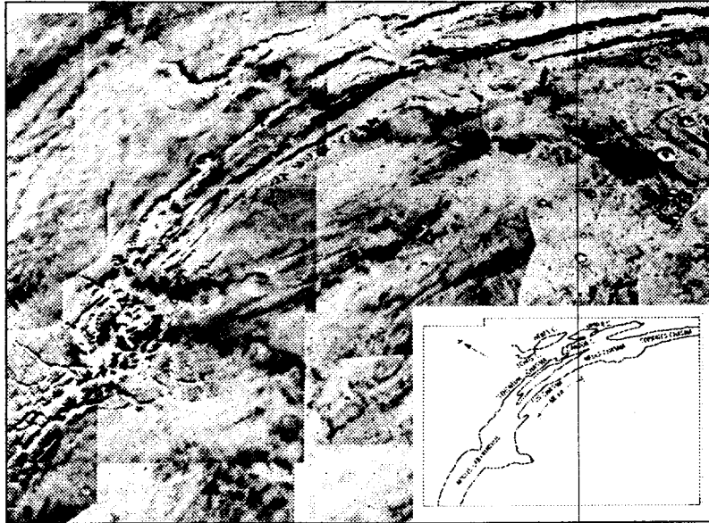
Figure 3.2.1-4. Channel network on Martian surface. (Spitzer, 1980)
