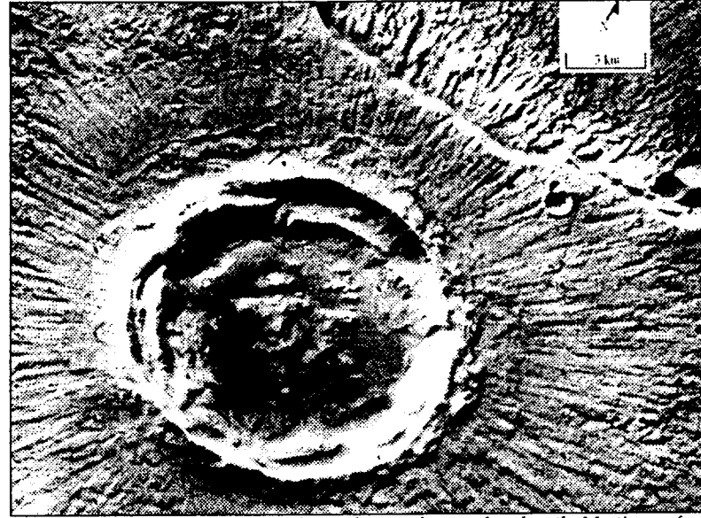
Figure 3.2.1-5. Poona Crater. One of several types of craters found on the Martian surface. (Spitzer, 1980)
