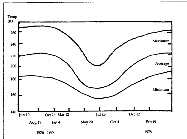
Figure 3.2.1-2. Chart of surface temperatures.
