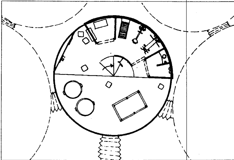
Figure 4.5.1.2-1. Floor plan of the lowest level of the habitat—the active recreation area and exercise facility of the entry module. Note: While each module has two levels, only the entry module is set lower in the Martian surface so that entry is on the second level of this module.
