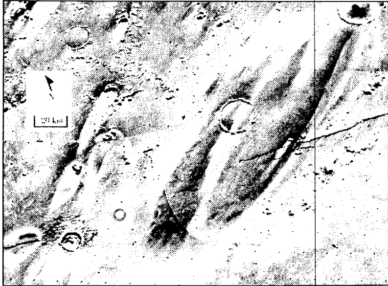
Figure 3.2.1-3. Distinctive streaks: the dark areas represent wind erosion, light centers where bright, fine particles deposit and collect (assumptions based on wind tunnel simulations). (Spitzer, 1980)
