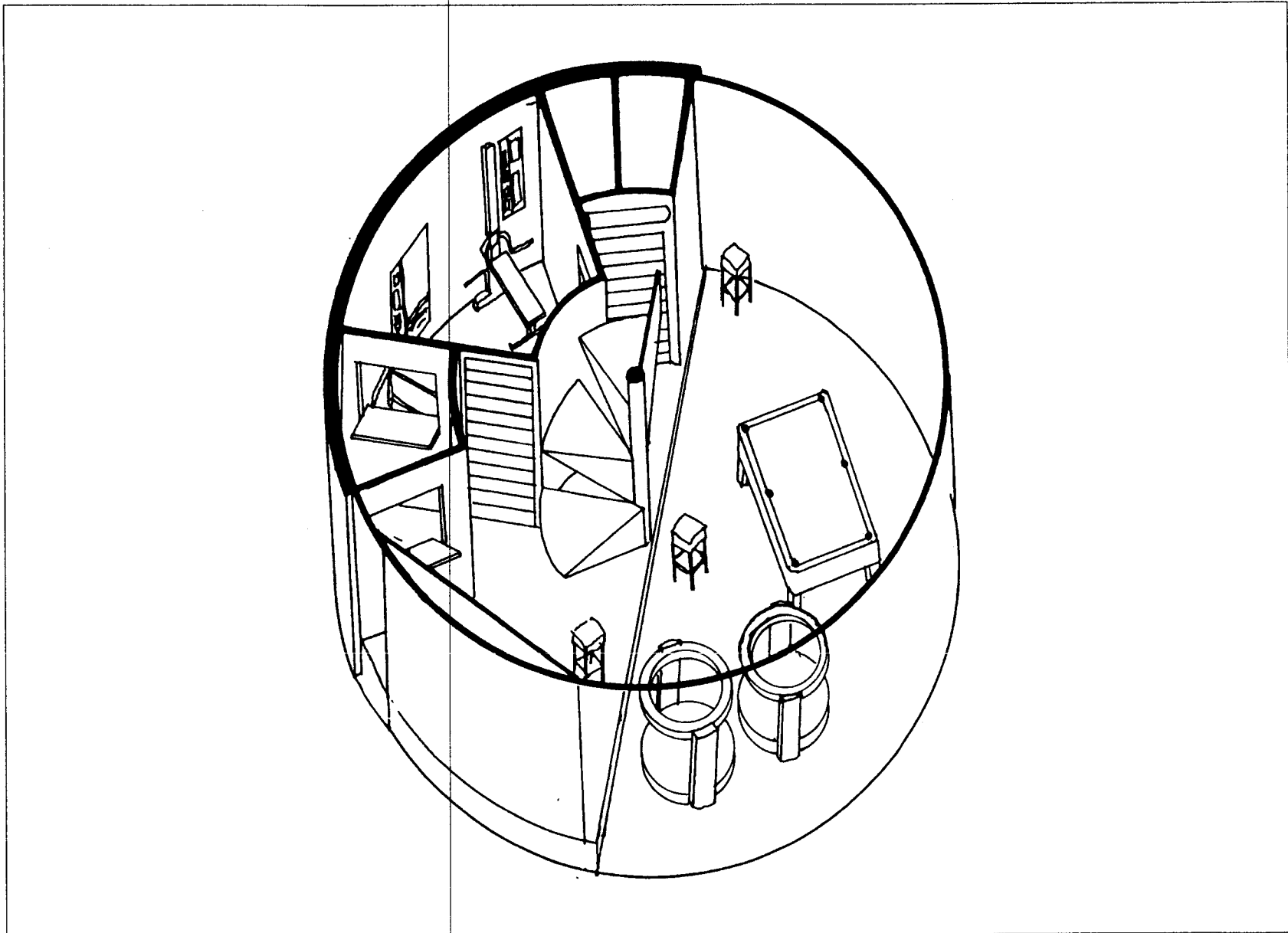
Figure 4.4.1-13. Axonometric of the lower level of the entry module (one level down from the entry level of Figure 4.4.1-11). Contained within is the active group recreation area and exercise facility.
