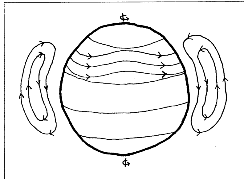
Figure 3.2.1-1. Diagram of Martian wind convections.
