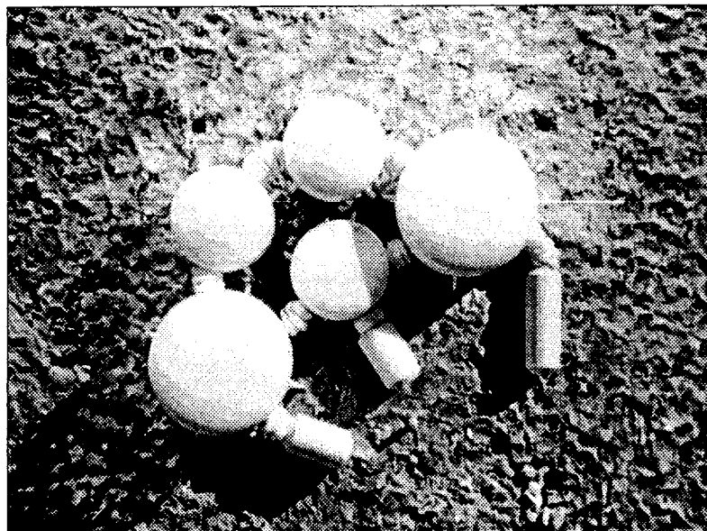
Figure 4.4.1-10. The habitat is comprised of three 9 m hard modules and two 12.6 m inflatables. Each module contains two levels.
