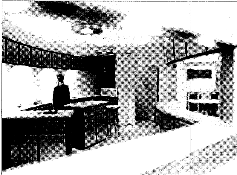
Figure 4.5.3.2-1. The galley is designed for ease of food preparation and maintenance., ample stowage, three separate workstations and mobile islands.
