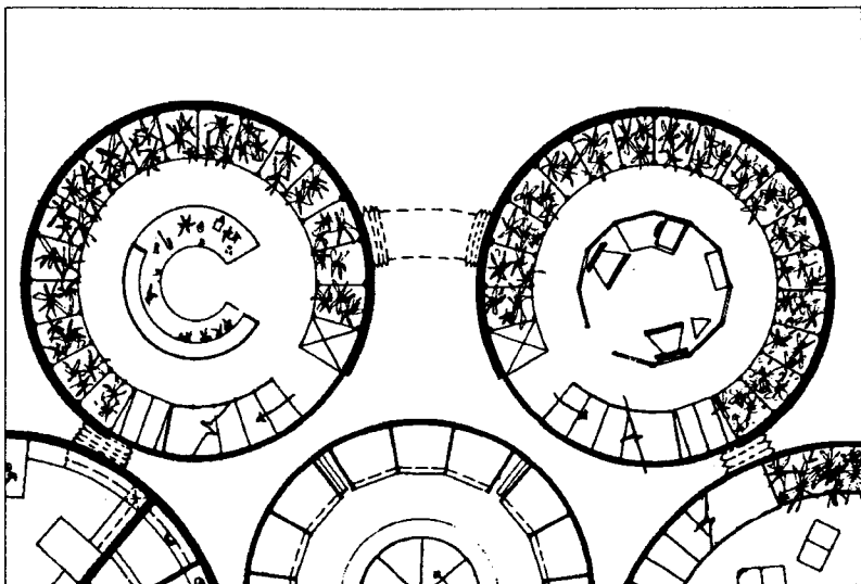
Figure 4.5.4.4-2. Floor plan of the lower floor of the two greenhouse modules, showing the carbon dioxide greenhouse with central work area on the left, and the oxygen greenhouse with central library on the right.
