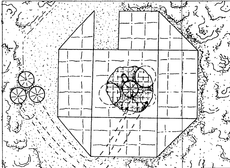
Figure 4.3-5. Rigid entry module is emplaced and the primary entrance airlock for the habitat is attached.
