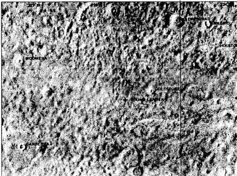
Figure 4.1-1. Viking 2 mission location at 45° north latitude, 251° west longitude.
