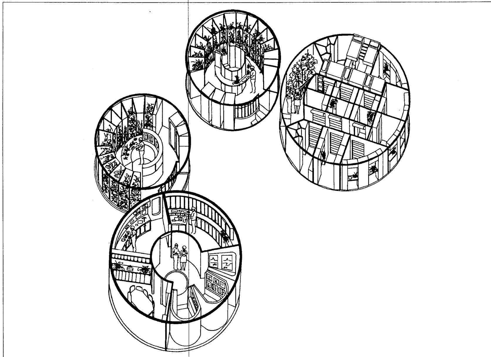
Figure 4.4.1-12. Axonometric drawing of the upper floor of Pax, illustrating the central focus and group interaction space in each module and the creation of a sense of place and homelike environment in all spaces.
