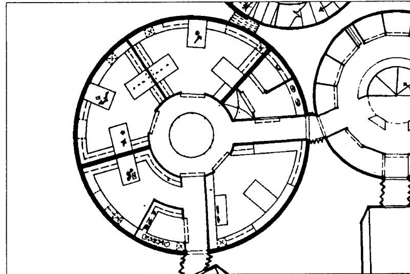
Figure 4.5.2.2-1. Floor plan of the main level of the laboratory module showing (from lower center, clock-wise) the general, chemistry, and biology labs, the HMF, and the microbiology labs.
