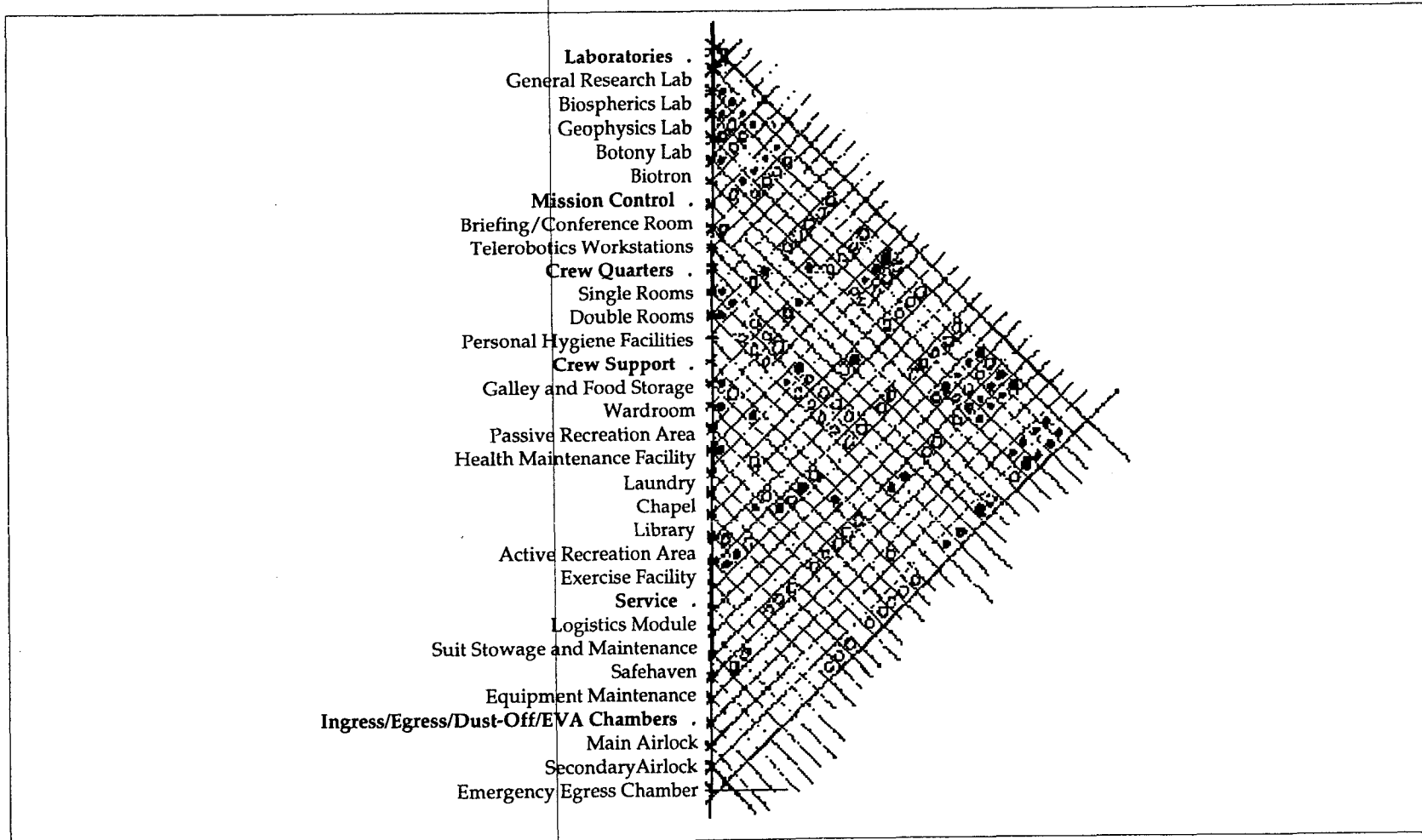
Figure 3.3.7-4. Adjacency matrix for required Martian habitat spaces.
