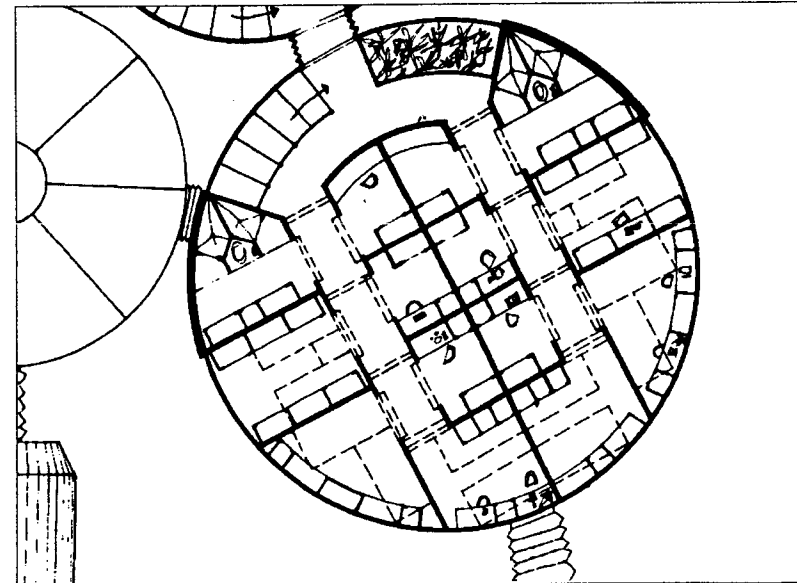
Figure 4.5.3.5-1. Upper level floor plan of the crew support module—the crew quarters and PAFs.
