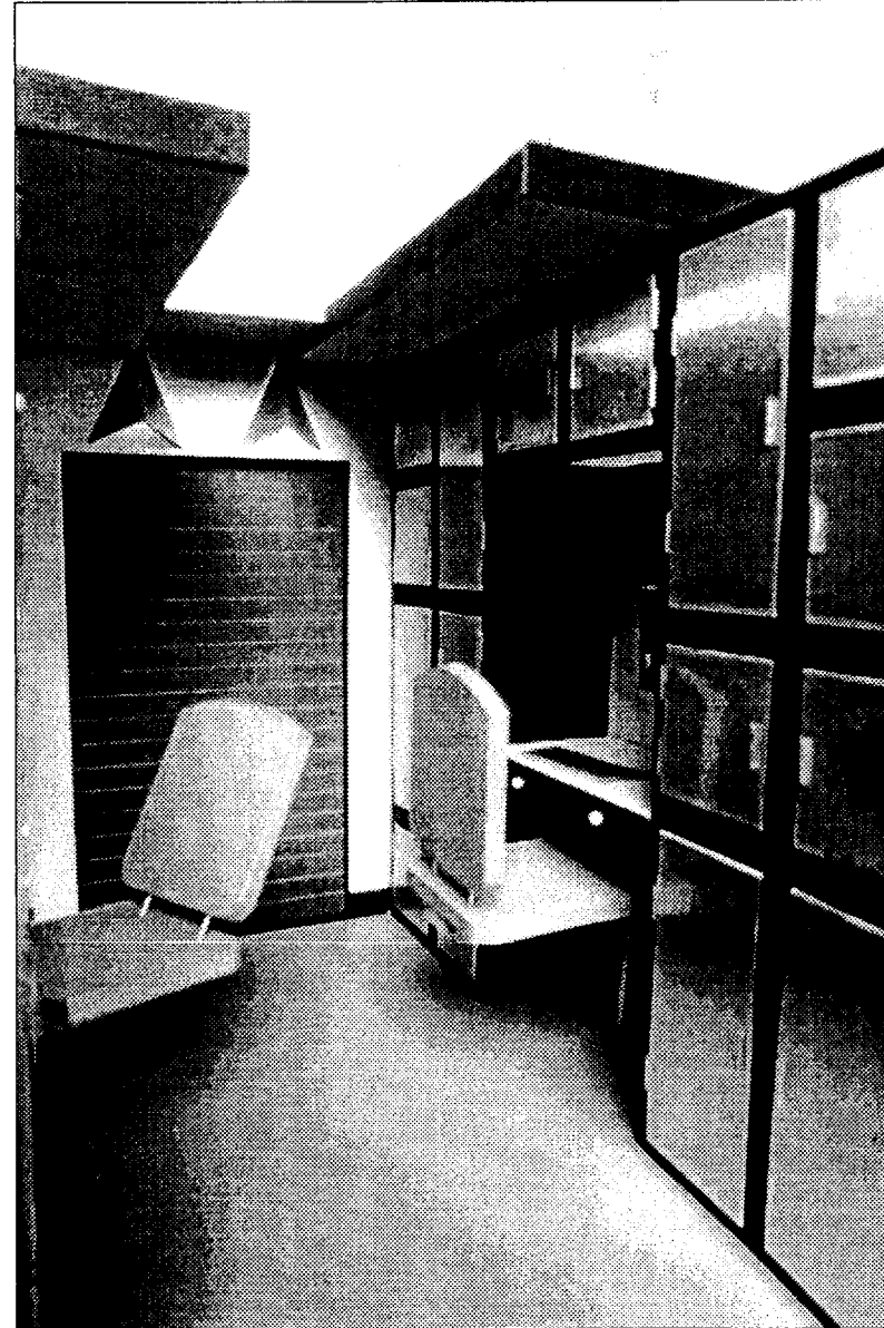
Figure 4.5.2.5-3. A shared crew quarter as viewed from the entrance to the space. Beds are lofted to provide additional floor space. Stowage compartments, on a modular system, are flexible and allow for room rearrangement.
