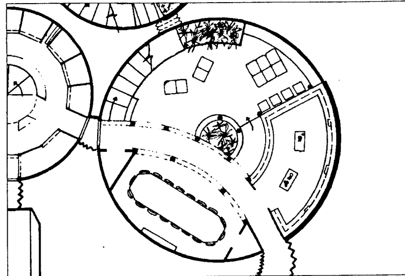
Figure 4.5.3-1. Main level floor plan of the crew support module. This level consists of a wardroom, galley, and group recreation space.
