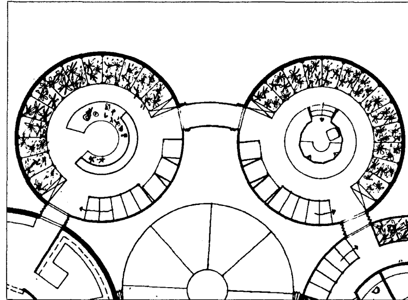
Figure 4.5.4-1. Floor plan of the upper level of the two greenhouse modules. Greenhouse accessibility is from the primary circulation space of the crew support module (upper level) and the botany labs of the laboratory module (upper level).
