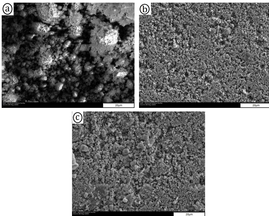
Figure 30: 0.2 wt% Boron Milled for 12 hours at 1000x magnification (a) Before Sintering, (b) Sintered for 1 hour, (c) Sintered for 10 hours
