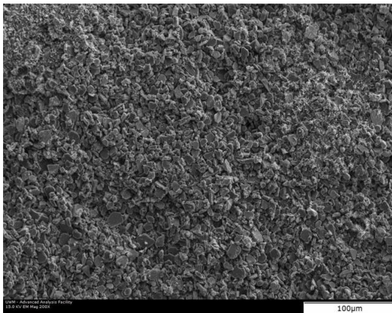
Figure 33: 1.0 wt% boron, hand mixed, sintered for 1 hour at 200x magnification
