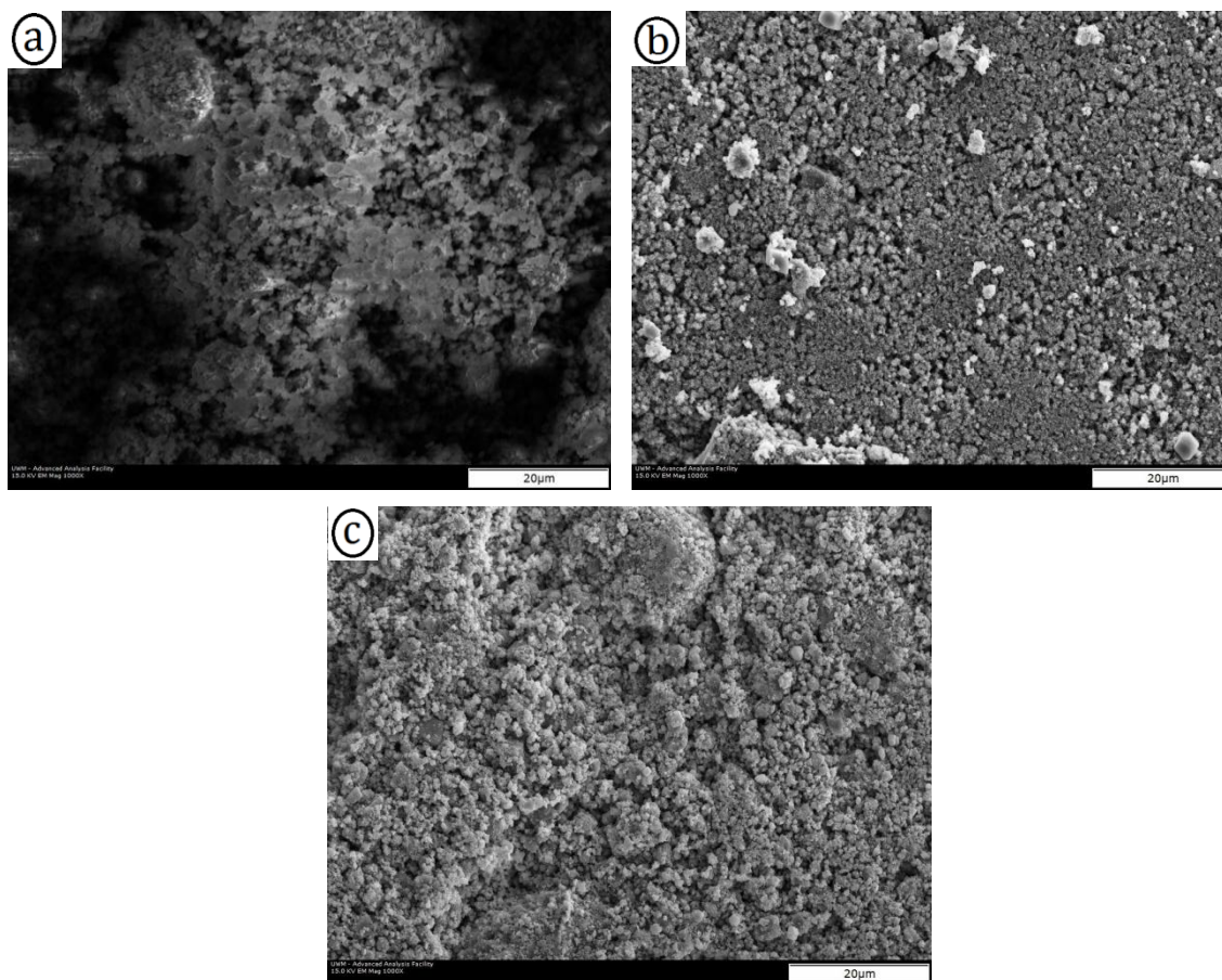
Figure 29: \text{Al}_2\text{O}_3 milled for 12 hours at 1000x magnification (a) Before sintering, (b) Sintered for 1 hour, (c) Sintered for 10 hours
