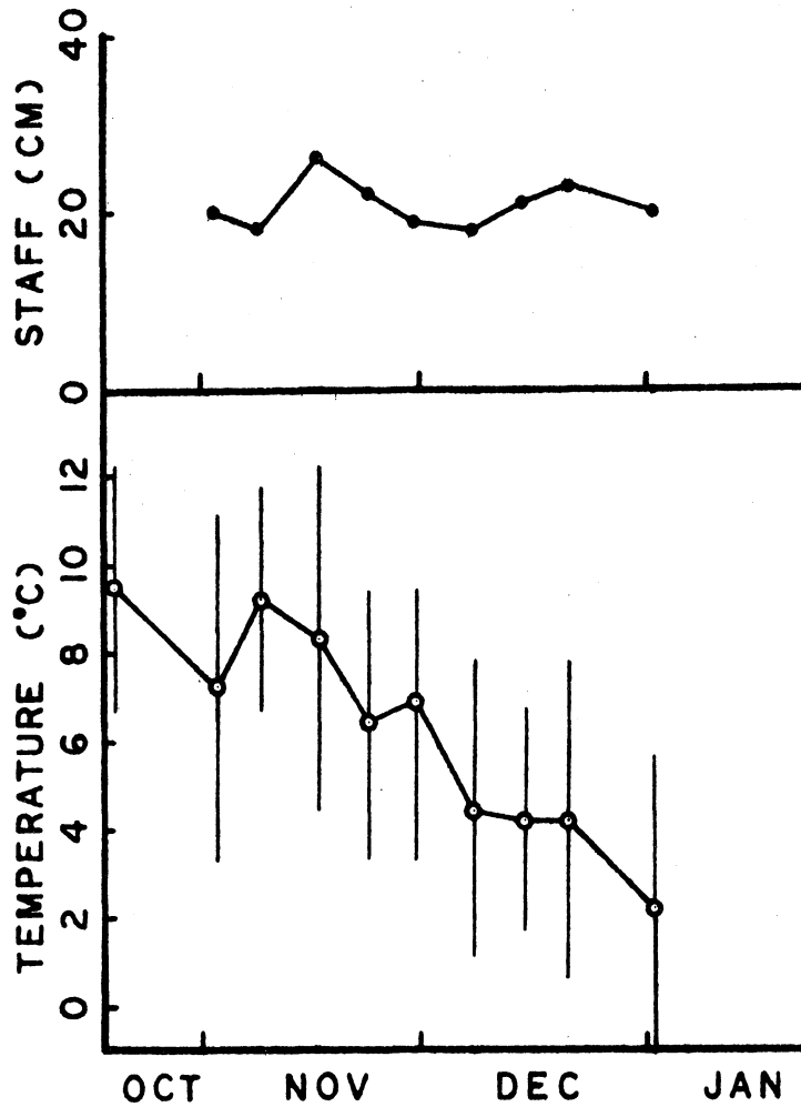
Appendix A. — Staff gauge levels and stream temperatures in Benner Run 1975-1976. Vertical bars denote temperature ranges and open circles denote midpoints of temperature ranges recorded by maximum-minimum thermometer.
