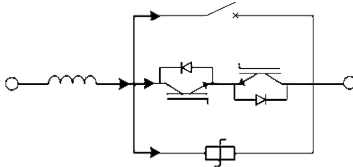
(b) igbt Solid State Circuit semiconductors
