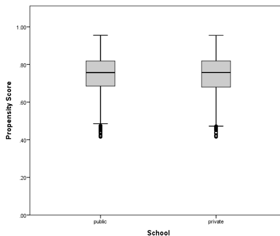
Figure 2: Boxplots
