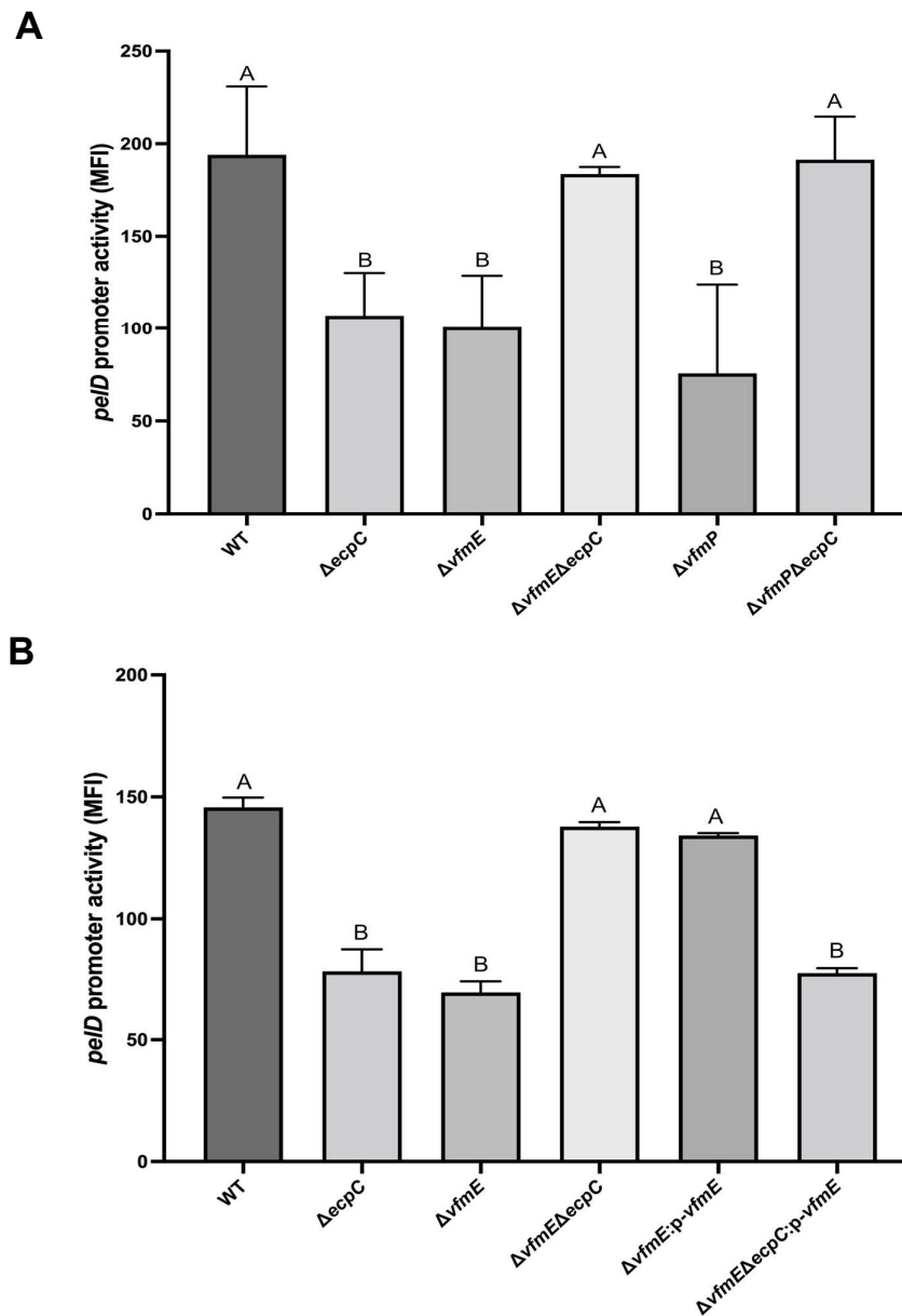
Fig. 2.1. Deletion of vmE and vmP in wild type (WT) decreases pe D promoter activity; on the other hand, deletion of both vmE and vmP under high c-di-GMP background (Δ ecpC ) restores the pe D promoter activity to WT level.
