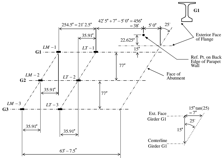
PLAN - Instrumentation Layout: B-20-148
