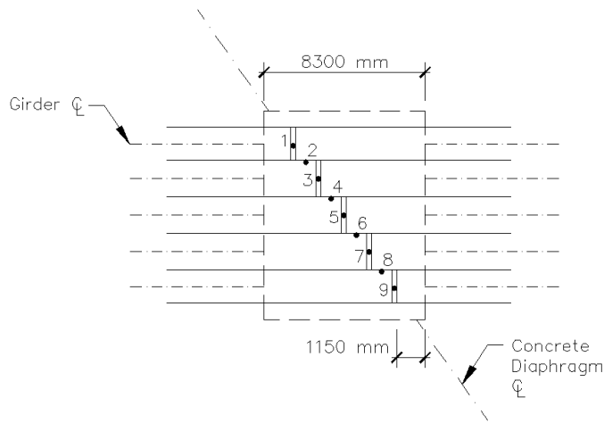
Figure 5.28 Nodal Locations over the Interior Pier (Komp 2009).
