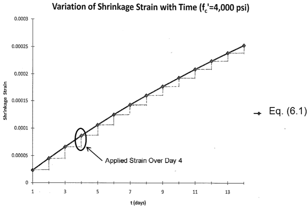
Figure 5.19 Step-Modeling Shrinkage Strain Variation with Time (Komp 2009).
