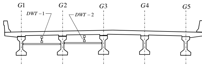
Section Indicating DWT Device Mounting
