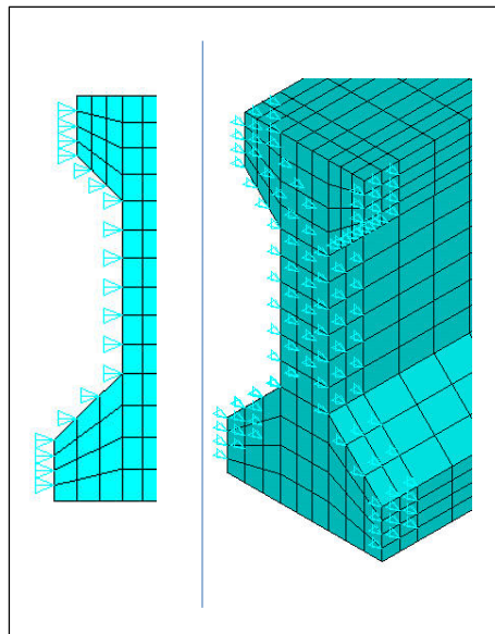
Figure 5.9 End Diaphragm Restraints (Komp 2009).
