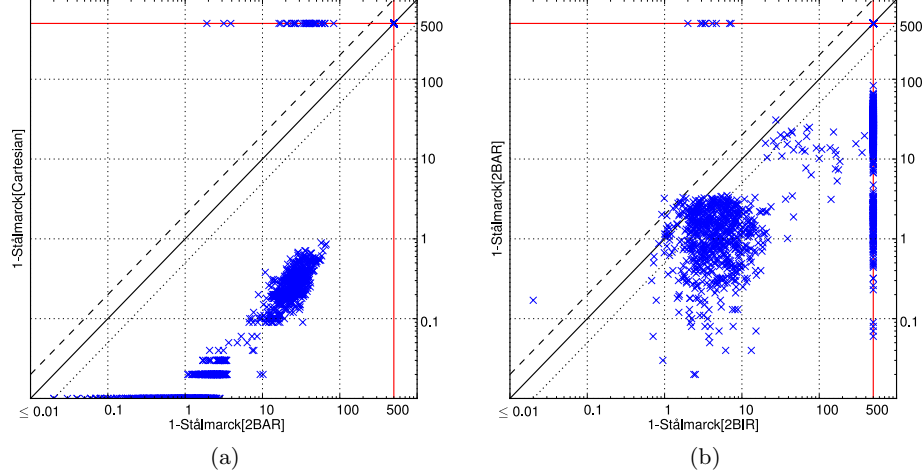
Fig. 15: Log-log scatter plots of the time taken (in seconds) by (a) 1\text{-Stålmarck}[2\text{-BAR}] versus 1\text{-Stålmarck}[\text{Cartesian}] , and (b) 1\text{-Stålmarck}[2\text{-BIR}] versus 1\text{-Stålmarck}[2\text{-BAR}] .
