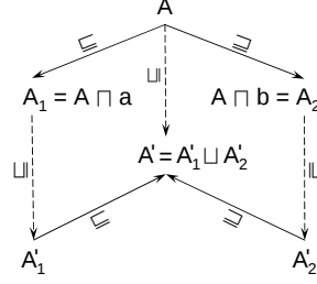
Fig. 10: Generalized Dilemma Rule.
