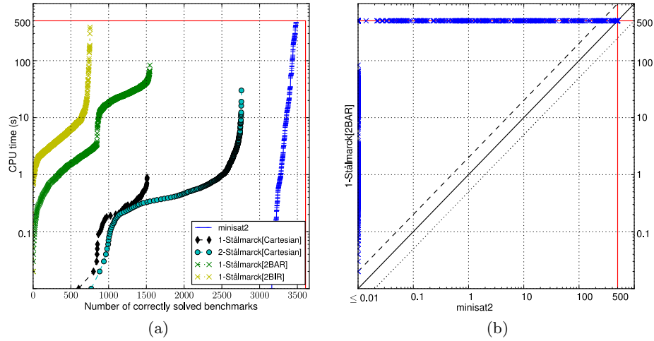
Fig. 14: (a) Semi-log plot showing the number of benchmarks that were each solved correctly in no more than t seconds. (b) Log-log scatter plot of the time taken (in seconds) by MiniSat versus 1 -Stålmarck[2-BAR].
