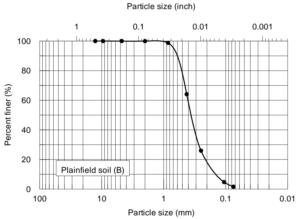
Figure A.25: Particle size distribution curve for Plainfield soil
