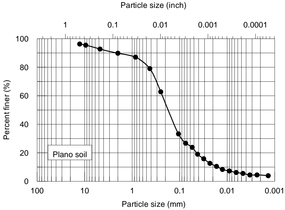
Figure 4.5: Particle size distribution curve of Plano soil
