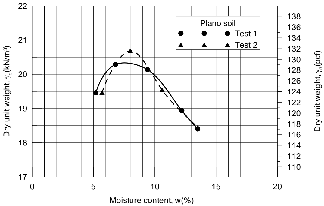
Figure 4.6: Results of Standard Proctor test for Plano soil
