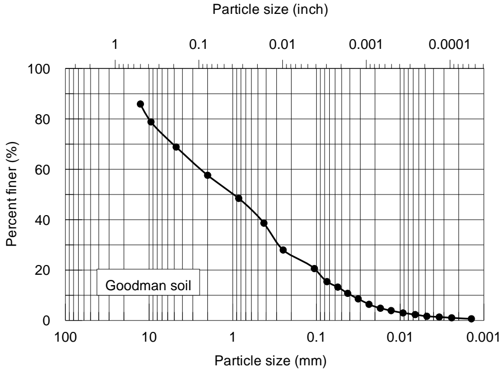
Figure A.5: Particle size distribution curve for Goodman soil
