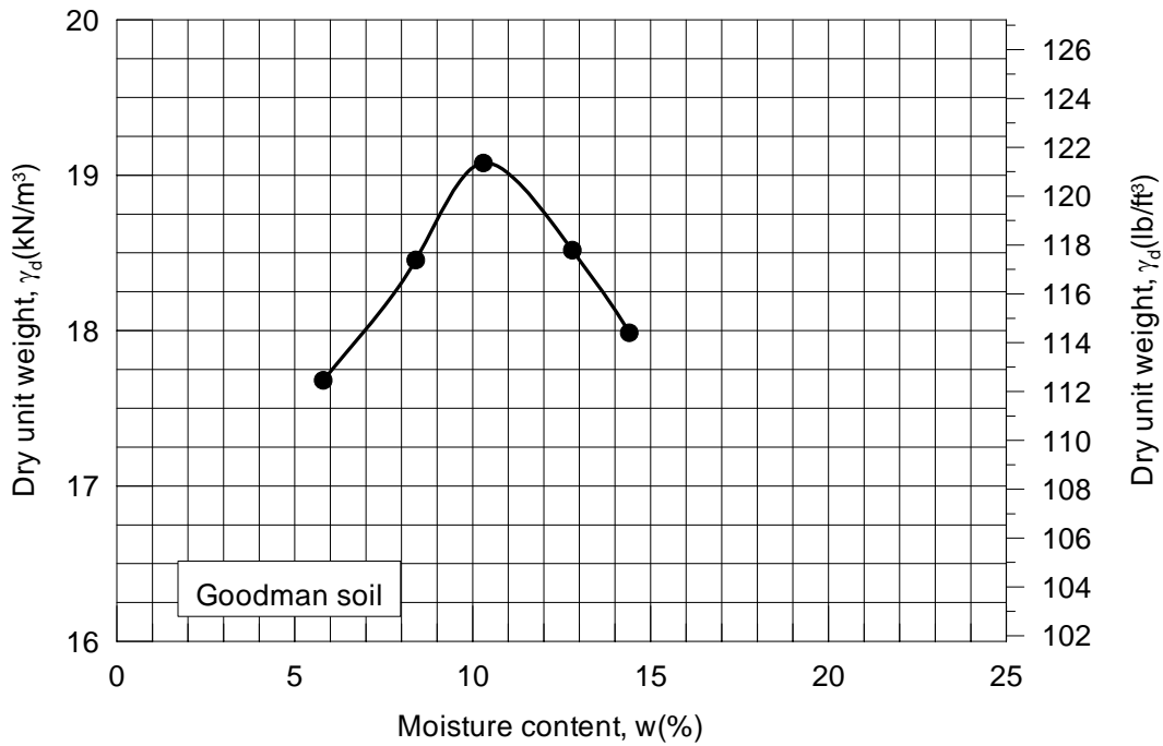
Figure A.6: Results of Standard Proctor test for Goodman soil
