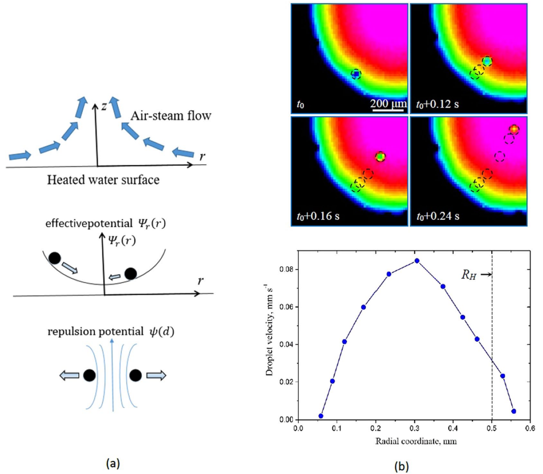
Figure 4. (a) The air-steam flow over the heated water surface creates pressure gradient causing droplets to levitate. The r -component of the drag force can be approximated with an effective potential and is minimal at the center. The repulsion force between the droplets can be presented as a repulsion potential. Together, dragging droplets to the center combined with the repulsion results in the observed packing of the droplets minimizing the total potential \Psi_{total} and thus leading to the self-assembly as evidenced by Voronoi entropy decrease. (b) Experimental observation of the velocity dependence on the distance from the center for a single droplet.
