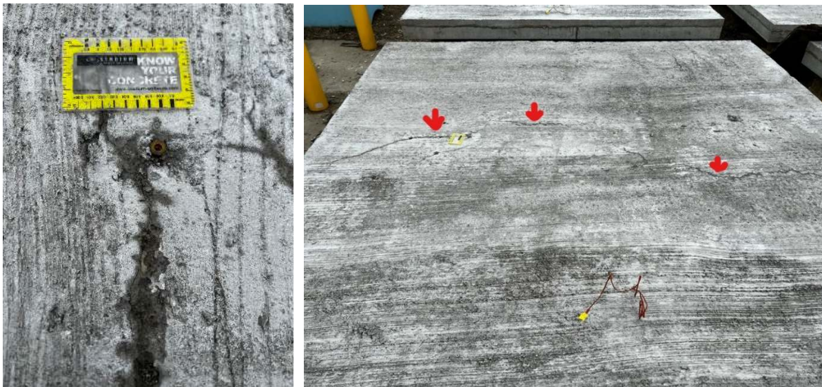
Figure 20 Cracks on Overlay Slab 7 (NC-I)
