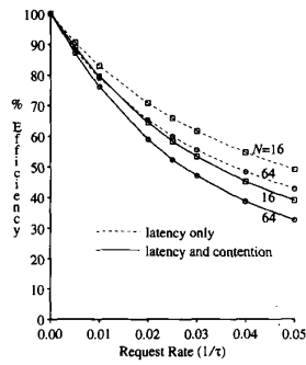
Fig. 5. Efficiency of baseline system. Bidirectional torus, single flit buffers, uniform traffic, N_{out} = 1 .
