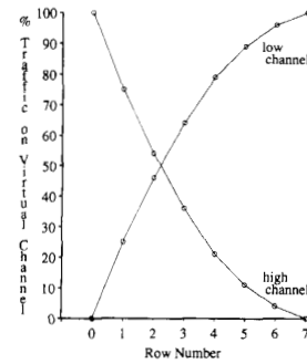
Fig. 4. Traffic on the high and low virtual channels along a column. Unidirectional 8 \times 8 torus. Uniform traffic distribution.
