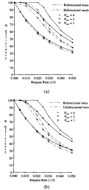
Fig. 9. Comparison of network topologies: 8 \times 8 system, uniform traffic, single-flit buffers. (a) Bidirectional torus vs. mesh. (b) Bidirectional torus vs. unidirectional torus.
