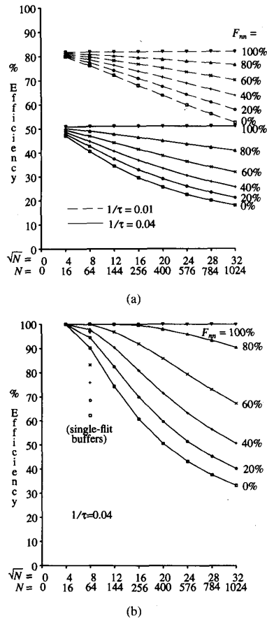
Fig. 10. Effect of communication locality. Bidirectional torus, infinite buffers except single points in (b). (a) N_{out} = 1 . (b) N_{out} = 4 .
