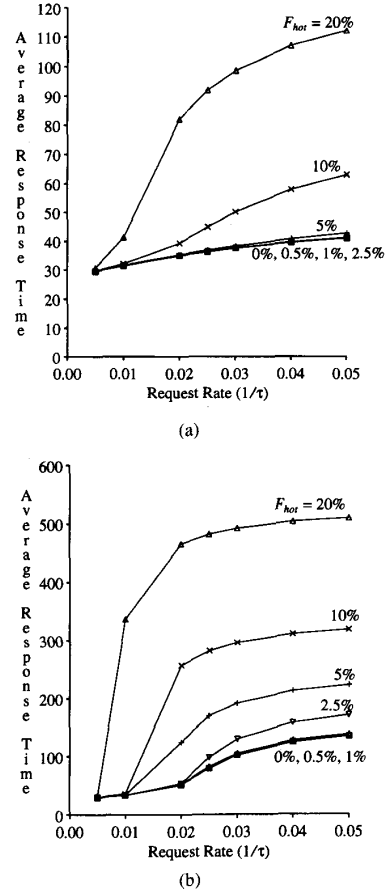
Fig. 11. The effect of hot-spots on overall mean response times. Bidirectional 8 \times 8 torus, single-flit buffers. (a) N_{out} = 1 . (b) N_{out} = 4 .
