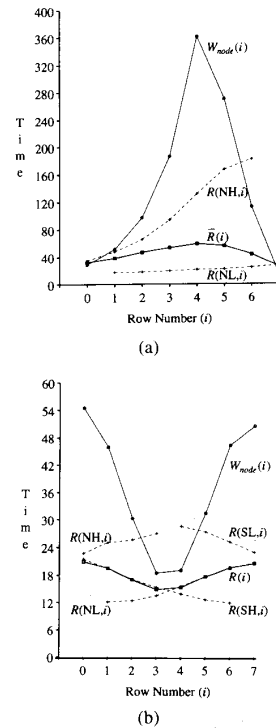
Fig. 16. Residence time on first virtual channel. Nodes on column 3; single-flit buffers, uniform traffic.
