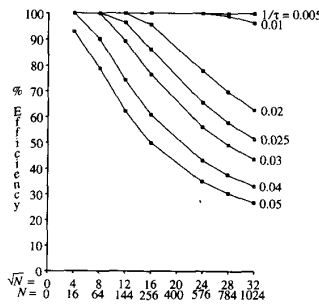
Fig. 8. Scalability with four outstanding requests. Bidirectional torus, uniform traffic, infinite buffers.
