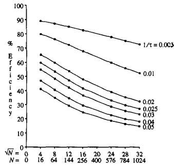
Fig. 6. Scalability of baseline system. Bidirectional torus, infinite buffers, uniform traffic, N_{out} = 1 .
