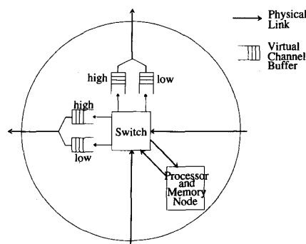
Fig. 2. A node in a unidirectional networks.
