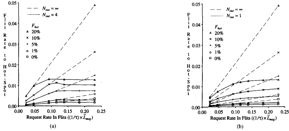
Fig. 14. Effective flit rate to hot node with blocking and nonblocking processors. Bidirectional 8 \times 8 torus, single-flit buffers, multiple node-to-switch links.
