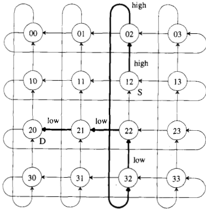
Fig. 3. Example for deadlock-free routing algorithm. Unidirectional 4 \times 4 torus. Channels on path from S = 12 to D = 20 .
