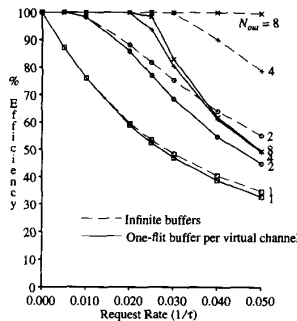
Fig. 7. Efficiency with multiple outstanding requests. Bidirectional torus, uniform traffic, N = 64 .
