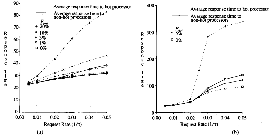
Fig. 13. The effect of hot-spots on mean response times to non-hot processors. Bidirectional 8 \times 8 torus, single-flit buffers, multiple node-to-switch links.
