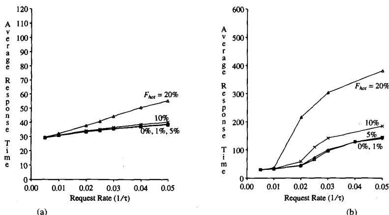
Fig. 12. Overall mean response times under hot-spot traffic with multiple node-to-switch links. Bidirectional 8 \times 8 torus, single-flit buffers. (a) N_{out} = 1 . (b) N_{out} = 4 .
