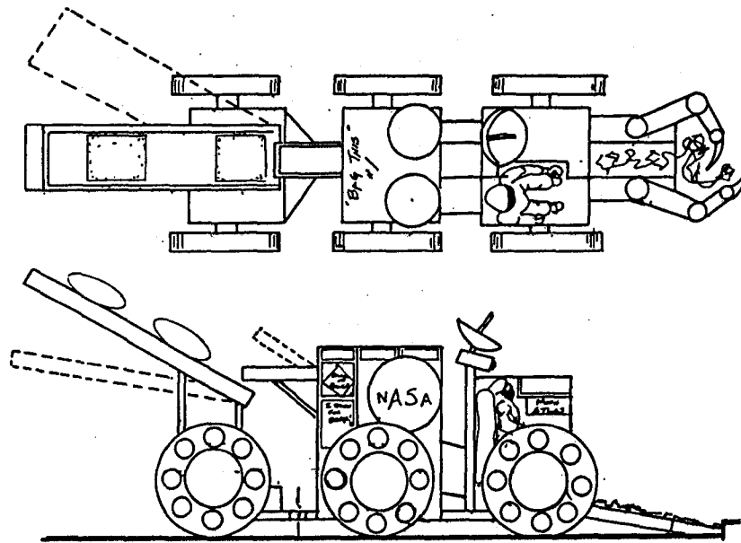
Figure 7.2.4-1. Concept drawing for a multiply-functioning regolith collecting and bagging machine.
