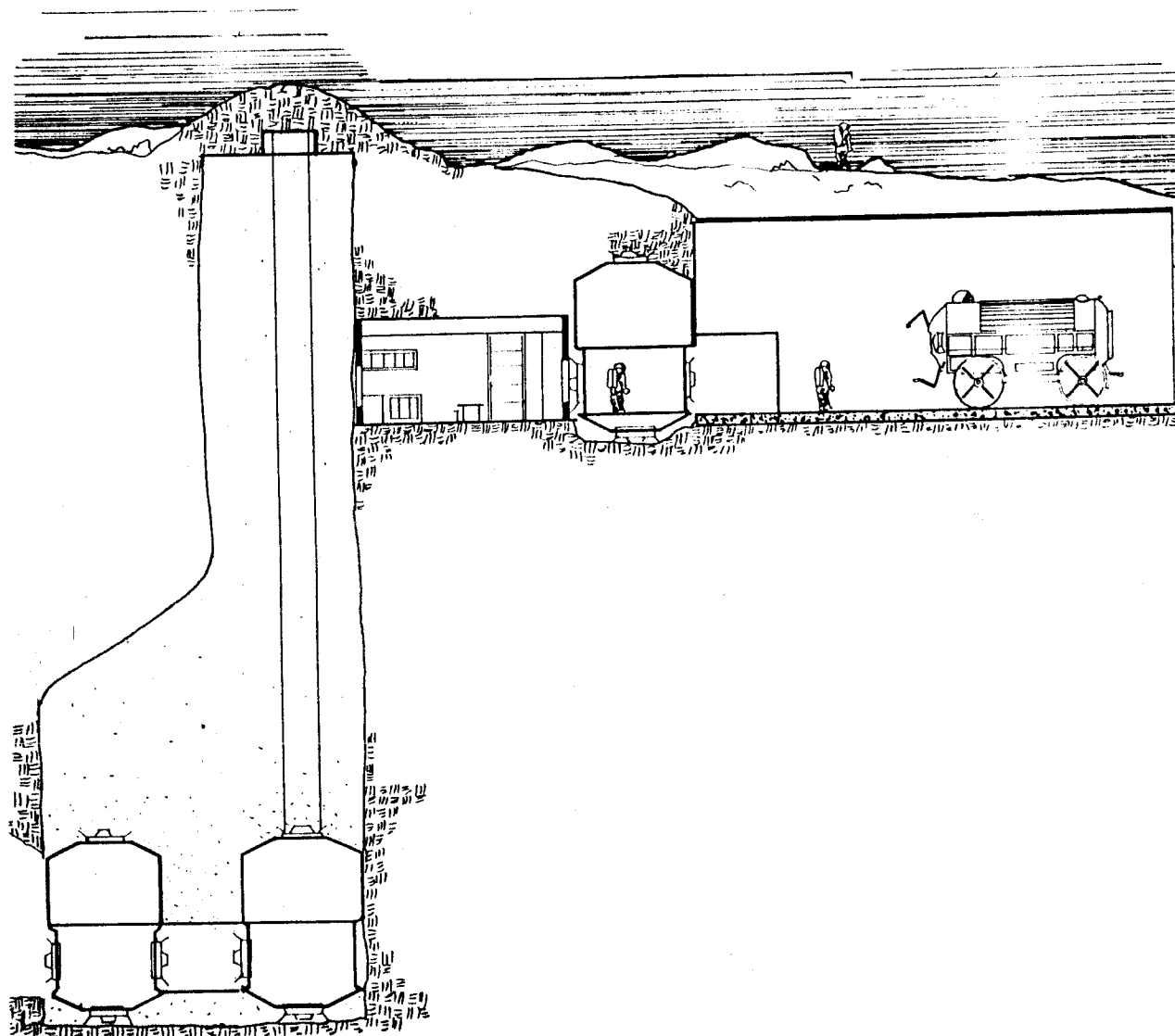
Figure 7.1.2-2. The other entrance/exit to the lava tube showing the logistics/storage area.
