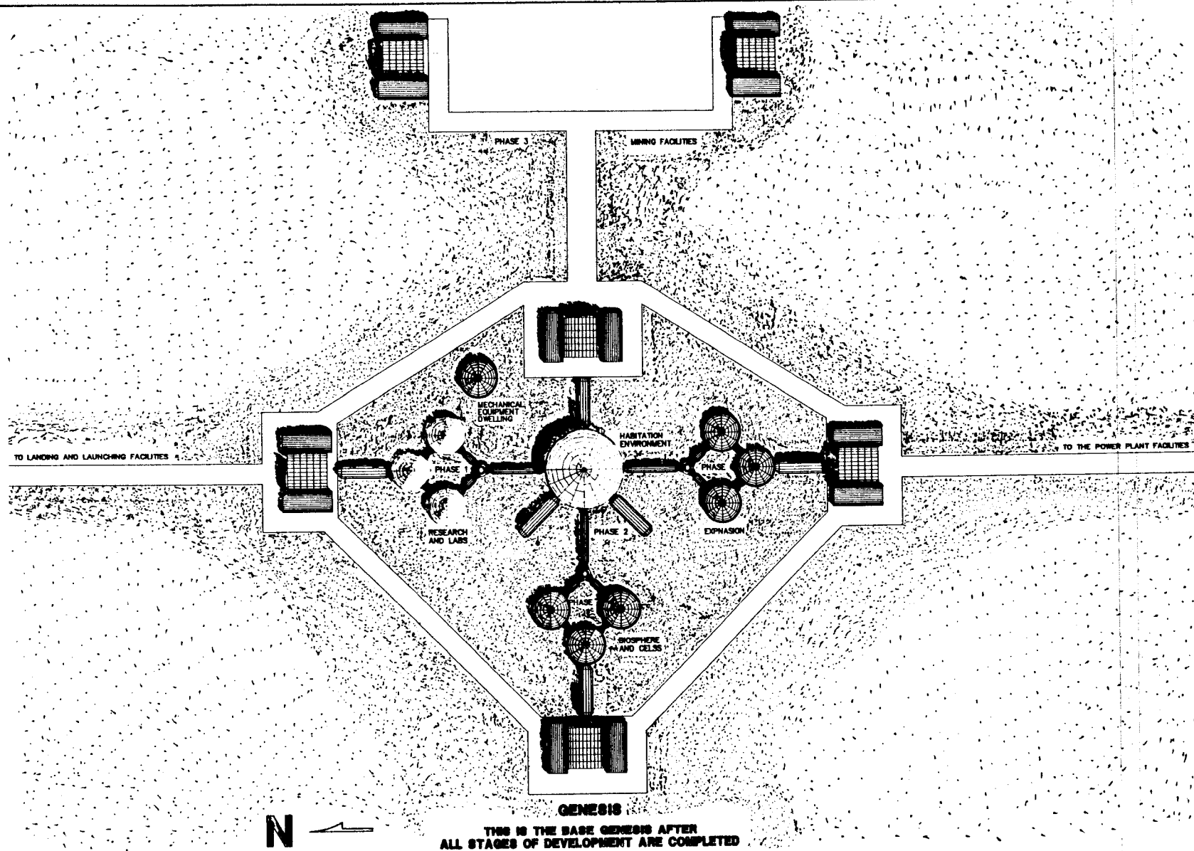
Figure 7.1.3-1. Site configuration of the inflatable lunar outpost. Note that North is to the left.
