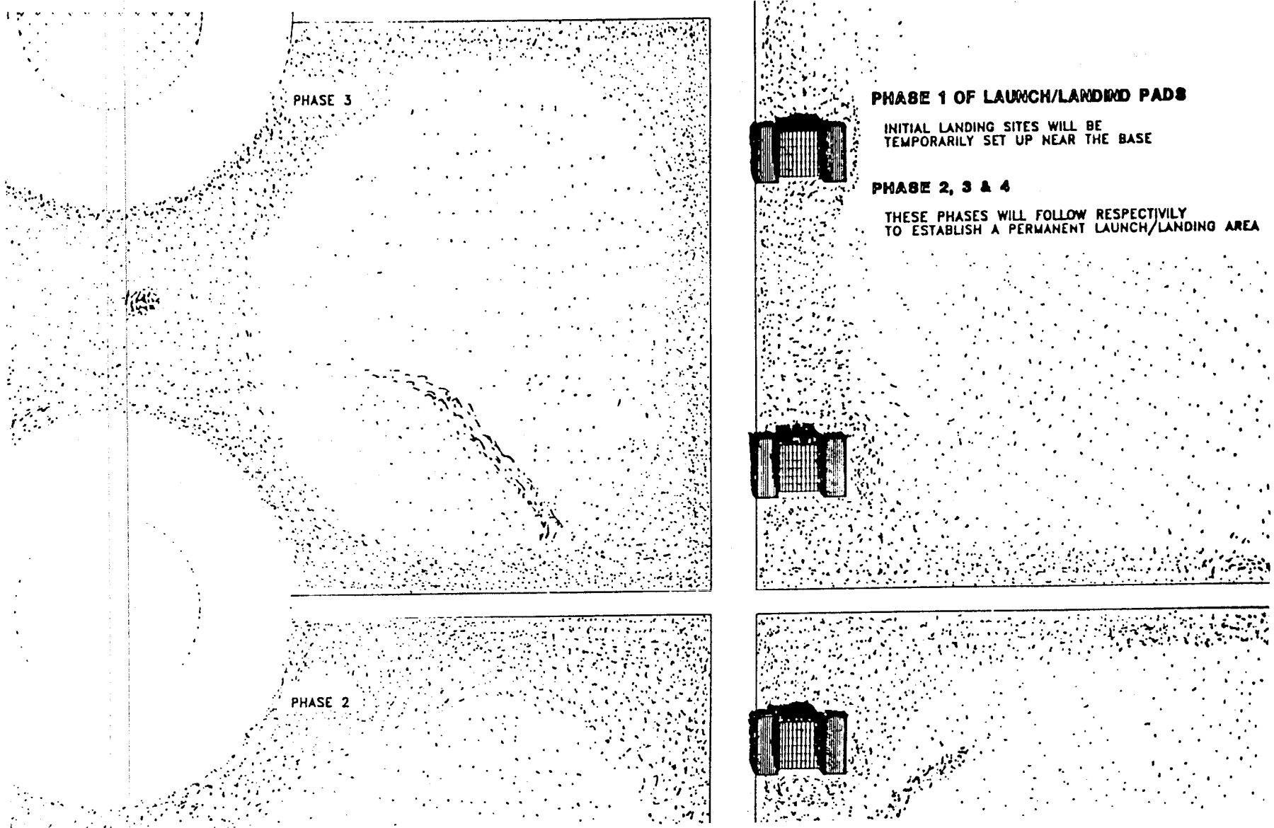
Figure 7.1.3-2. North end (left) of the site showing a portion of the launch/landing pads and growth through Phases 2, 3, and 4.
