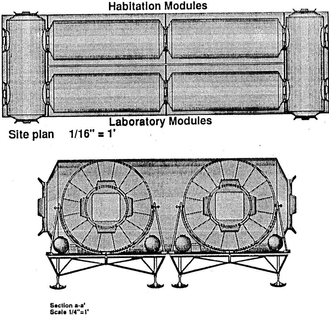
Figure 5.4-3. Module design.
