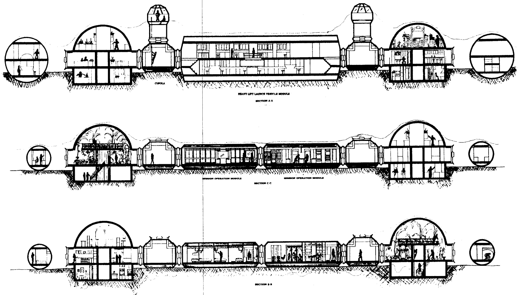
Figure 7.2.3-5. Section through all three arms of the base habitat.
