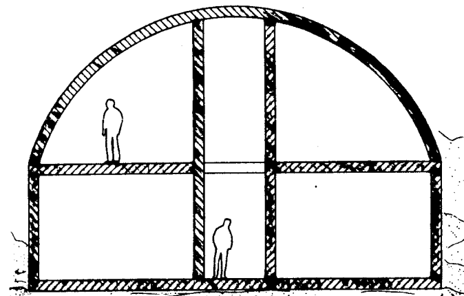
(h) The interior circulation core will finally be constructed, giving additional structural support.
