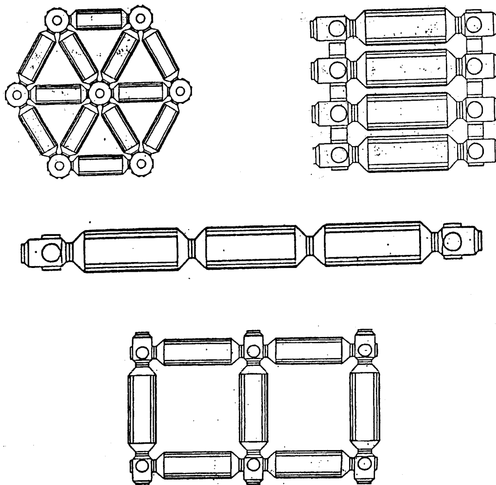
Figure 6.6.3-1. Comparison of triangular, raft, linear, and grid base layout configurations (SICSA, 1989).
