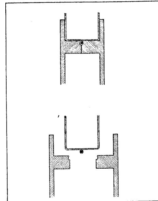
AIRLOCK AIRTIGHT SEAL DESIGN
