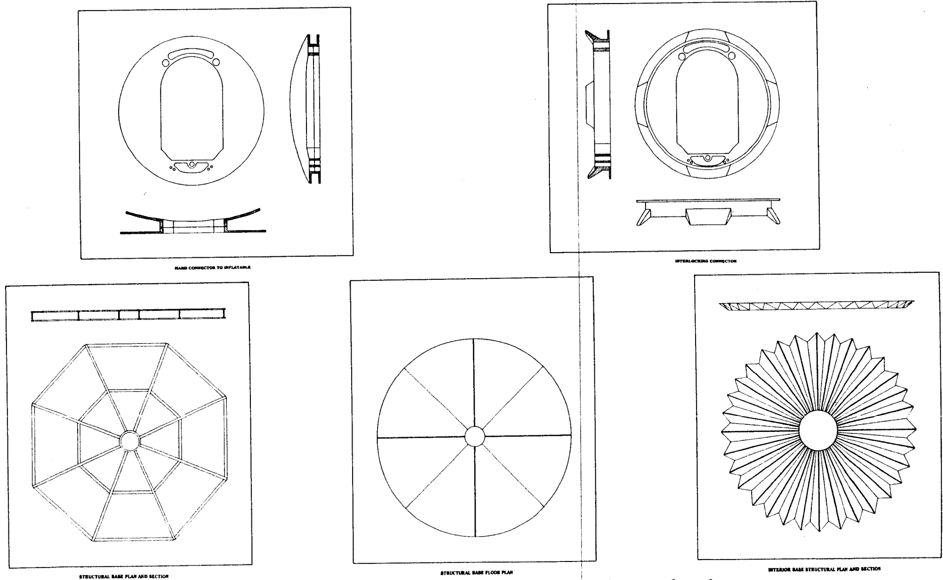
Figure 7.2.4-7. Hard connectors, interlocking connectors, and structural panels.
