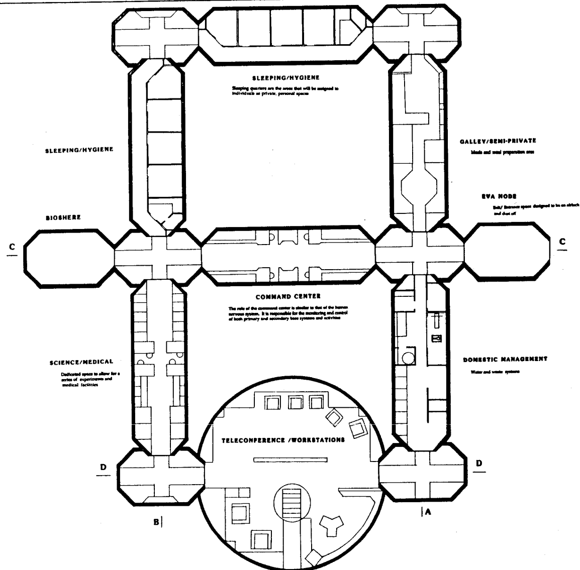
Figure 7.1.1-3. Base floor plan.
