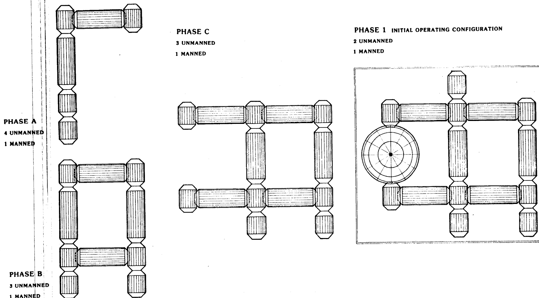
Figure 7.1.1-1. Initial three phases for the hard module scenario of a Lunar Outpost leading up to IOC.
