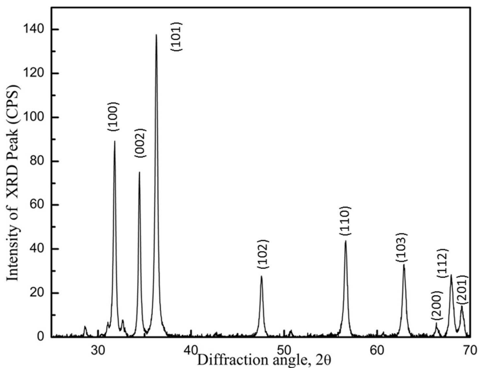
Figure 6.10: XRD pattern of ZnO NPs sample
