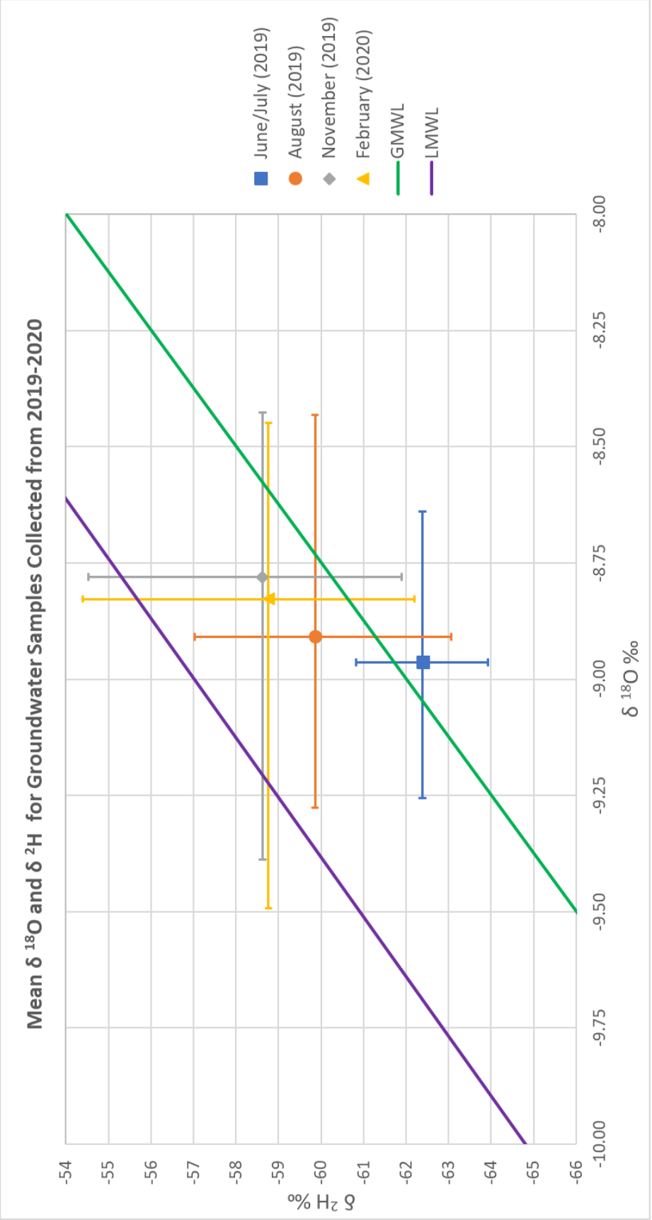
Figure 12: Mean Stable Oxygen and Hydrogen Isotope Data from Groundwater Samples
