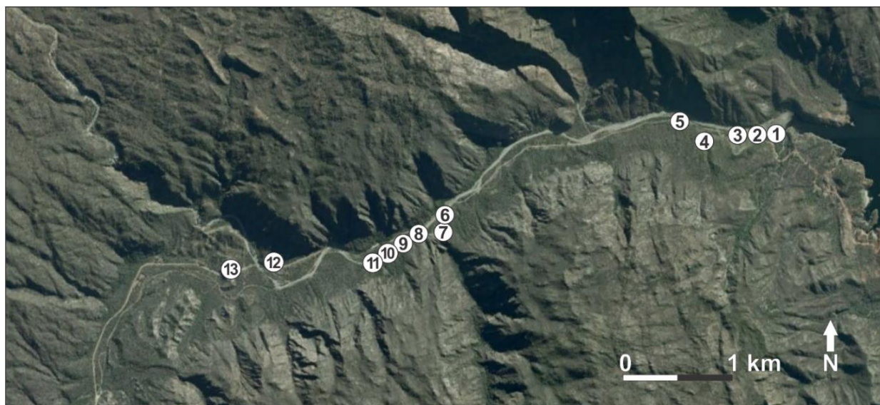
Figure 6. Aerial photo of the Olta paleovalley with locations of measured stratigraphic columns.
