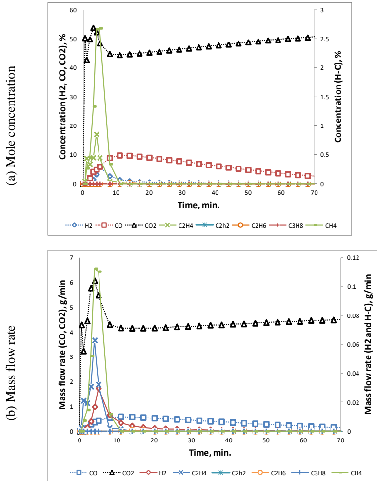
Figure 5-13 : The evolution of different gases at 800°C, case 1
