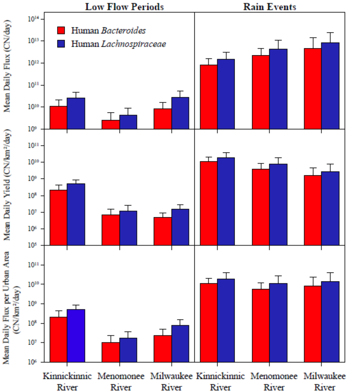
Figure 9: Mean daily fluxes, mean daily yields, and mean daily fluxes per urban area of human Bacteroides and human Lachnospiraceae in the Kinnickinnic (KK) River, Menomonee (MN) River, and Milwaukee (MKE) River for eleven rain events and four low flow periods collected in Milwaukee, Wisconsin in 2014 and 2015.
