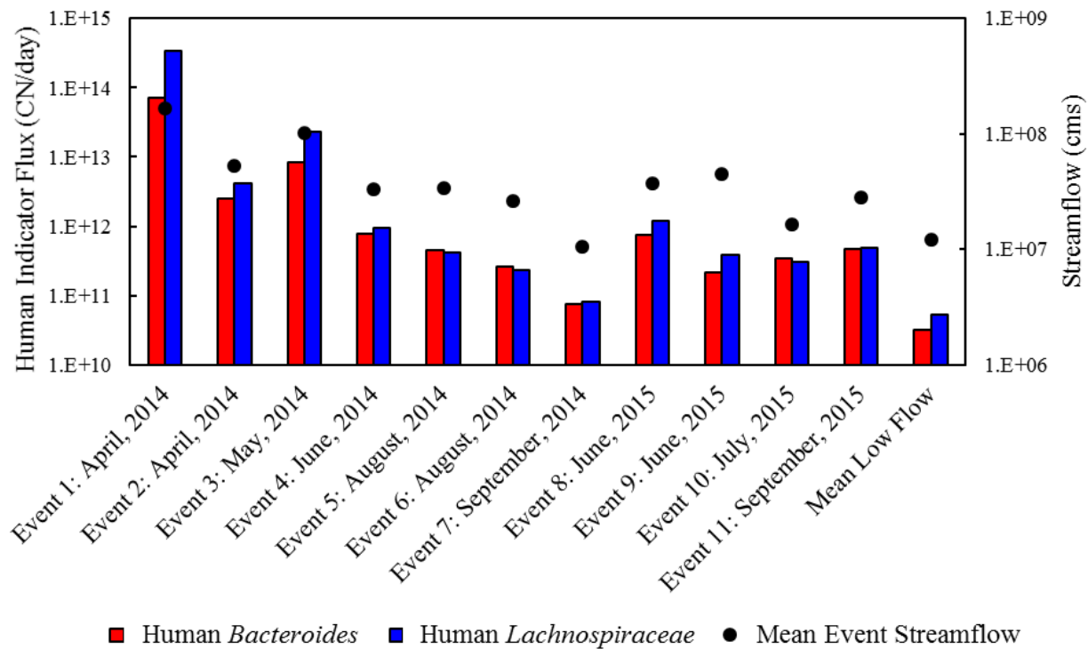
Figure 8: Daily fluxes of human Bacteroides and human Lachnospiraceae during 11 storm events, mean daily fluxes of these human fecal indicators collected during low flow, and mean streamflow of each event and low flow sampling period in the Milwaukee estuary in Milwaukee, Wisconsin in 2014 and 2015.
