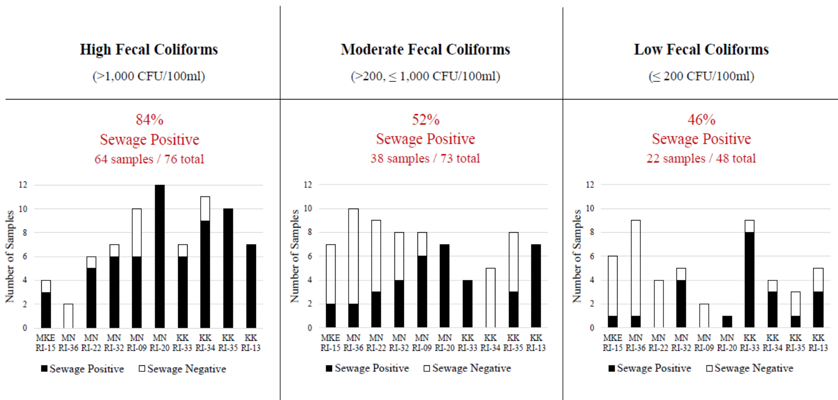
Figure 3: Distribution of sewage positive samples under three different fecal coliform concentration levels, across sampling locations in the Milwaukee (MKE), Menomonee (MN), and Kinnickinnic (KK) Rivers in metropolitan Milwaukee, Wisconsin in 2012 and 2013. Sites are listed from upstream to downstream in each river.
