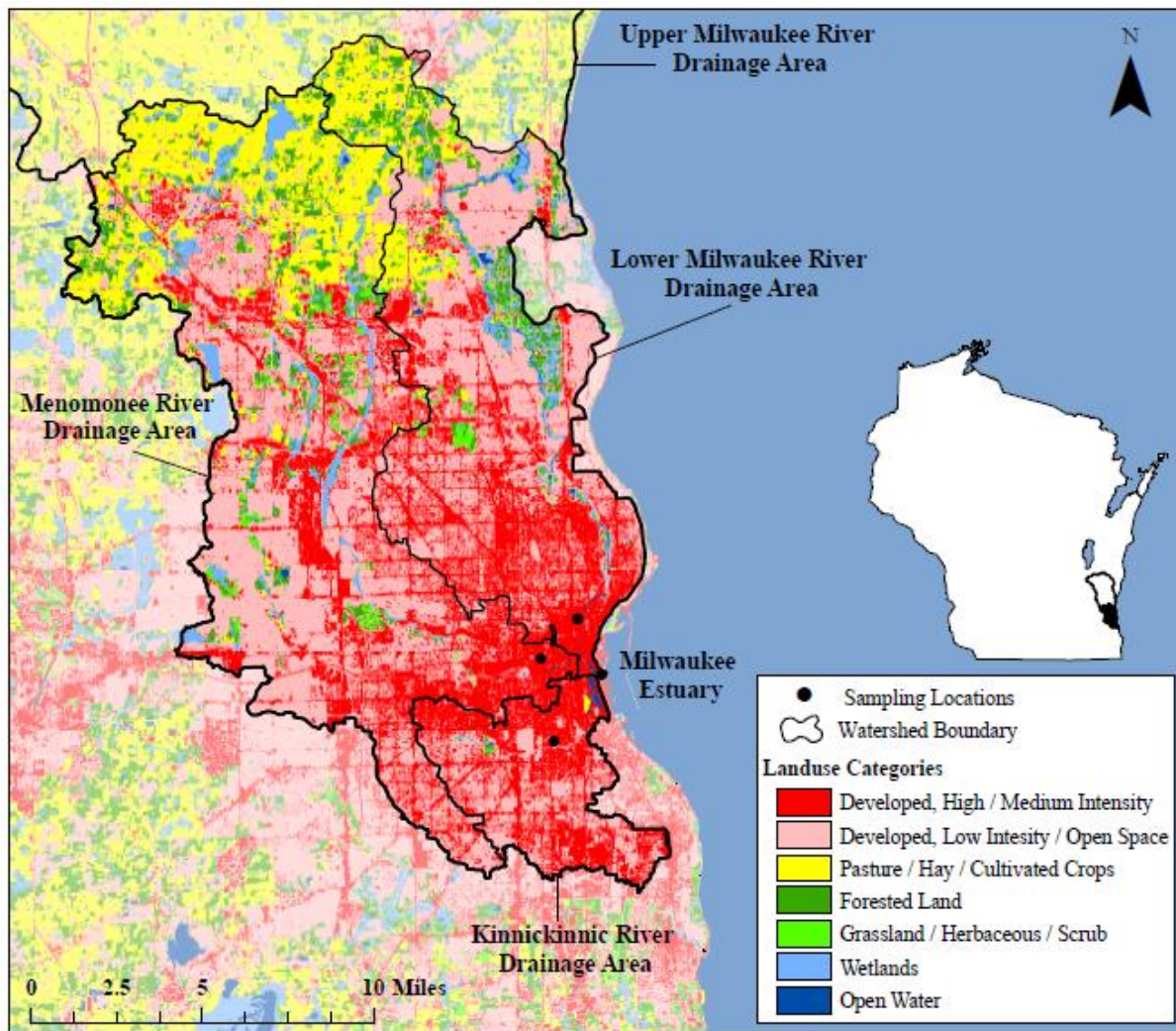
Figure 6: Sampling site locations, drainage areas, and land use in Milwaukee, Wisconsin. Base data from the National Land Cover Database (2011) Land Cover dataset (Jin et al., 2013).
