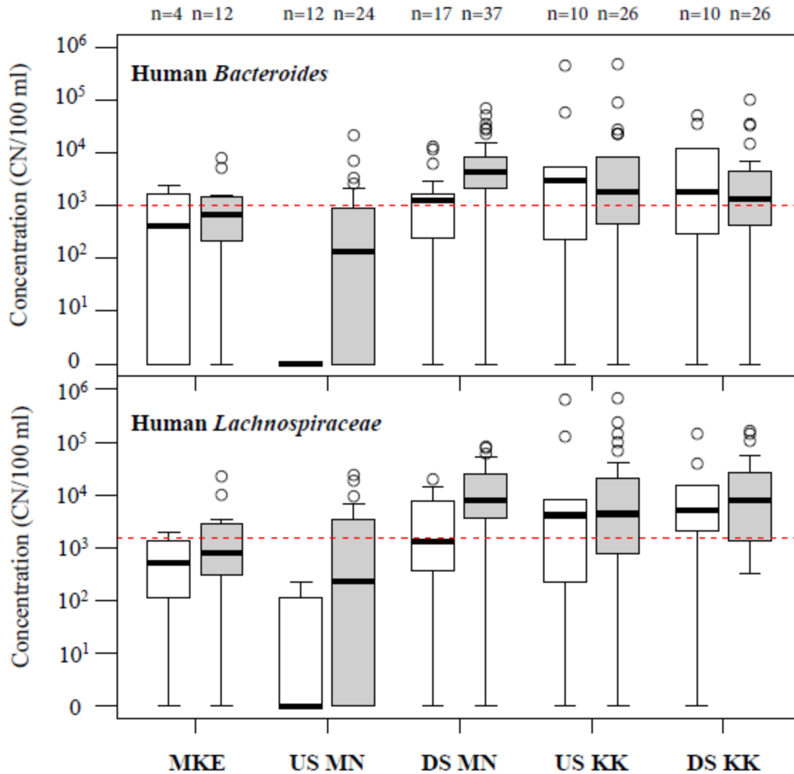
Figure 2: Human fecal indicator concentrations at baseflow (white plots) and wet weather (gray plots) in metropolitan Milwaukee, Wisconsin in 2012 and 2013. Dotted red lines represent sewage thresholds for human Bacteroides (1,000 CN/100 ml) and human Lachnospiraceae (1,500 CN/100 ml). The Milwaukee (MKE) River site MKE RI-15 is denoted as MKE. Upstream and downstream Menomonee (MN) River sites are denoted as US MN and DS MN, respectively. US MN sites include MN RI-36 and 22. DS MN sites include MN RI-32, 09, and 20. Upstream and downstream Kinnickinnic (KK) River sites are denoted as US KK and DS KK, respectively. US KK sites include KK RI-33 and 34. DS KK sites include KK RI-35 and 13.
