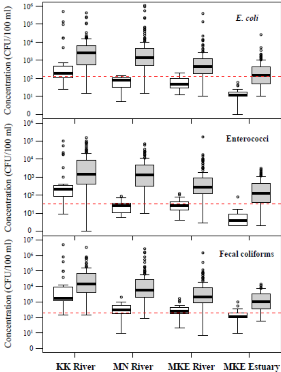
Figure 10: Concentrations of standard fecal indicator bacteria, Escherichia coli ( E. coli ), enterococci, and fecal coliforms, measured in the Kinnickinnic (KK), Menomonee (MN), and Milwaukee (MKE) Rivers, as well as the MKE estuary during dry weather (white plots) and rain events (gray plots) in Milwaukee, Wisconsin in 2014 and 2015. Red dotted lines represent the ambient water quality standards for E. coli (126 CFU/100 ml), enterococci (35 CFU/100 ml), and fecal coliforms (200 CFU/100 ml).
