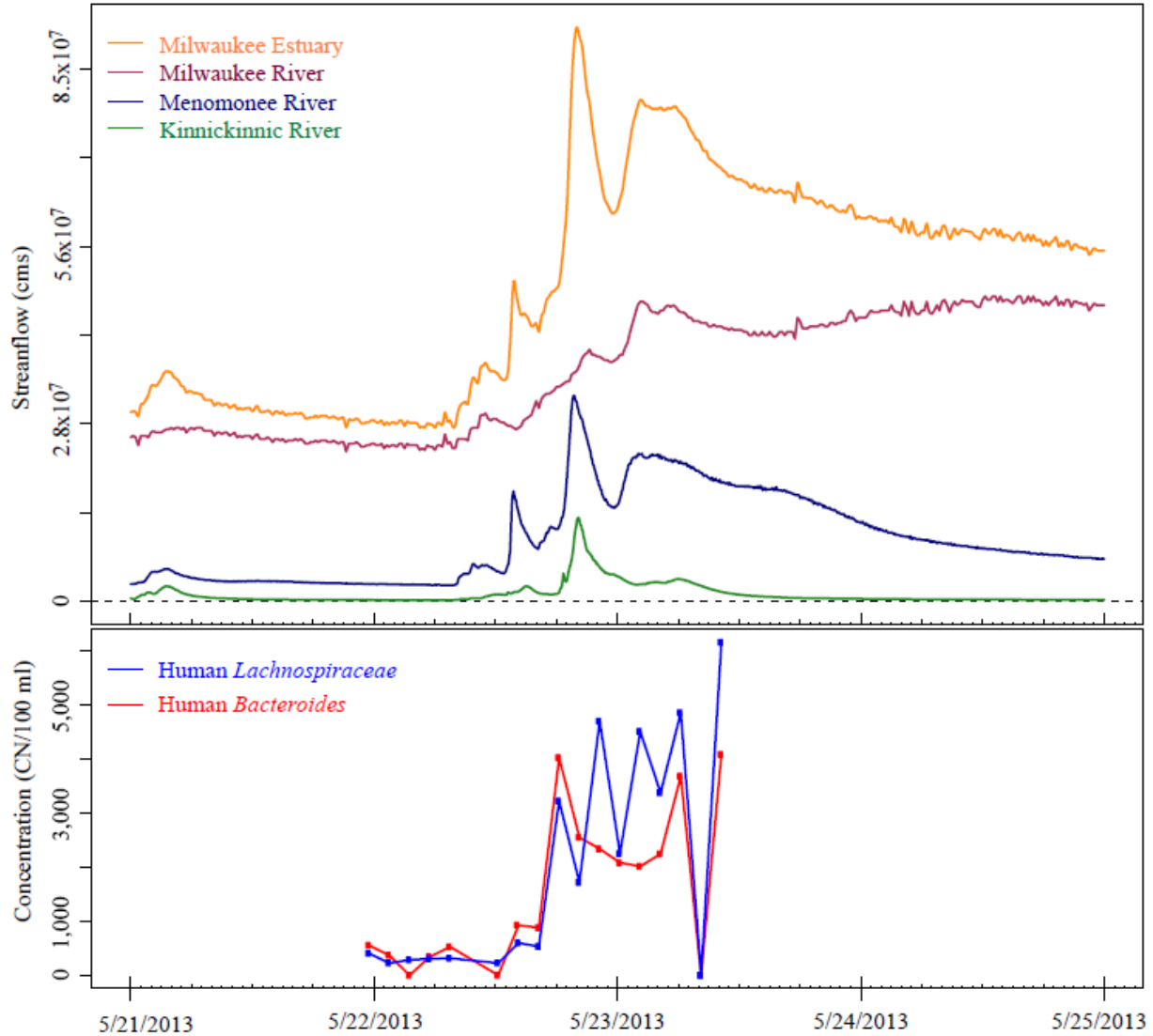
Figure 5: Streamflow in three rivers and the Milwaukee estuary (upper panel) and corresponding concentrations of human fecal indicators (lower panel) for a single rain event sampled across the hydrograph in the Milwaukee estuary at Jones Island wastewater reclamation facility in Milwaukee, Wisconsin in 2013.
