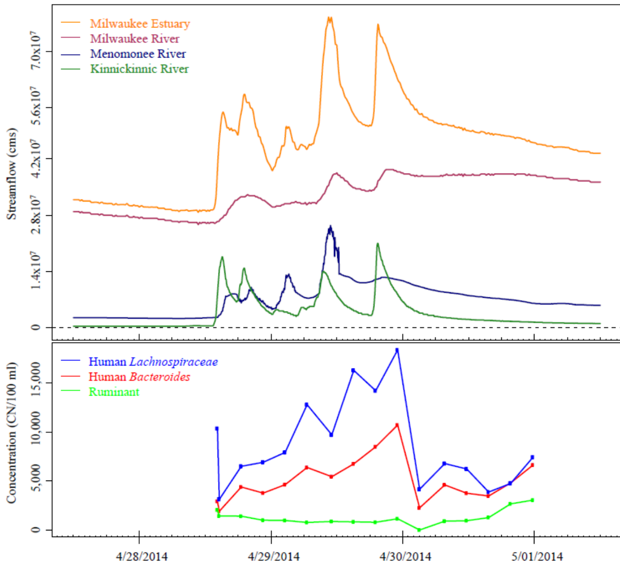
Figure 7: Streamflow (upper panel) and corresponding human Bacteroides , human Lachnospiraceae , and ruminant indicator concentrations (lower panel) measured during a single storm event in the Milwaukee estuary, collected at Jones Island water reclamation facility in Milwaukee, Wisconsin in 2014.
