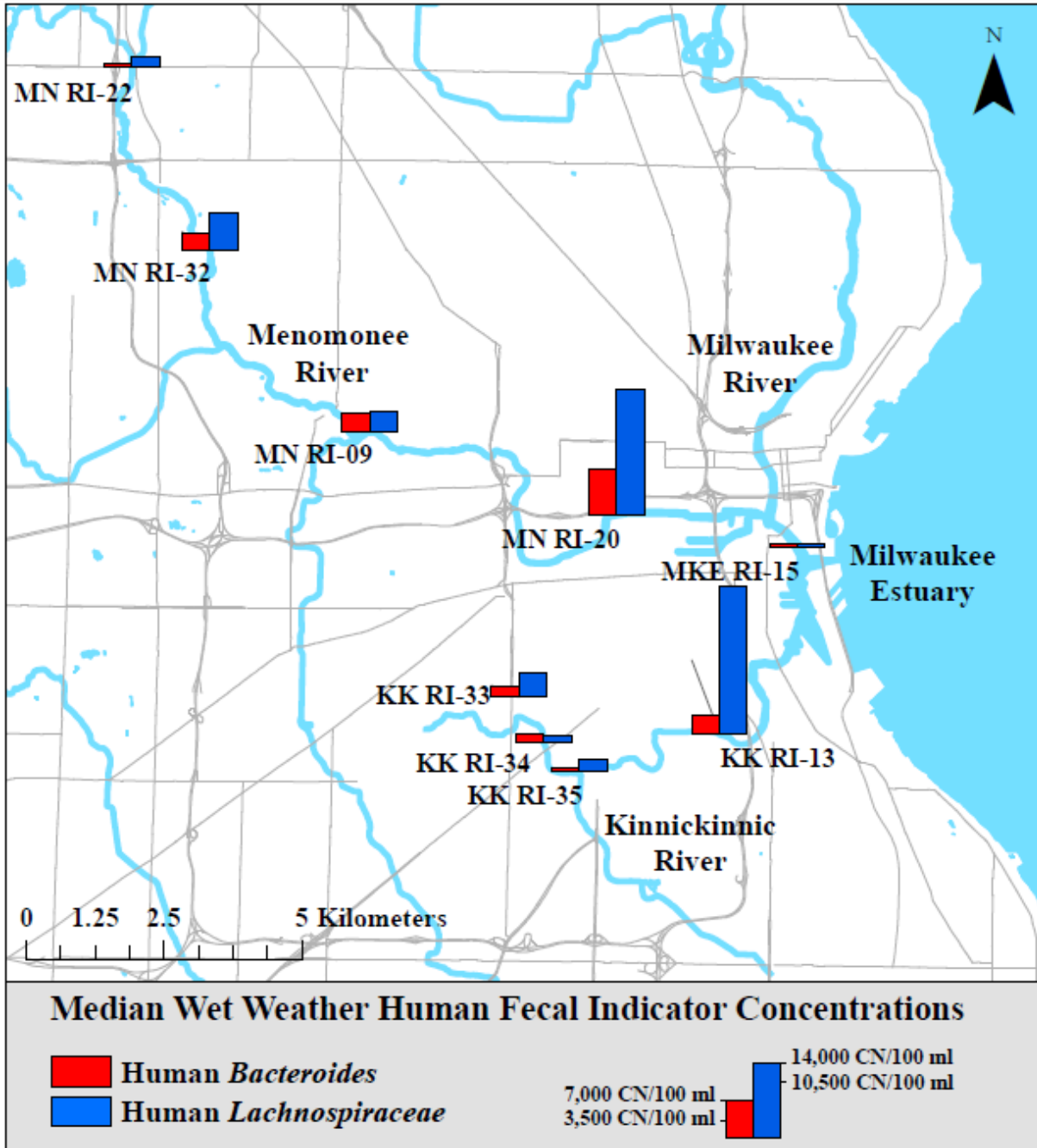
Figure 1: Median concentrations of Human Bacteroides and human Lachnospiraceae during wet weather on rivers in metropolitan Milwaukee, Wisconsin in 2012 and 2013. MN RI-36 is approximately 14 miles upstream of MN RI-22 and is not shown in this figure.
