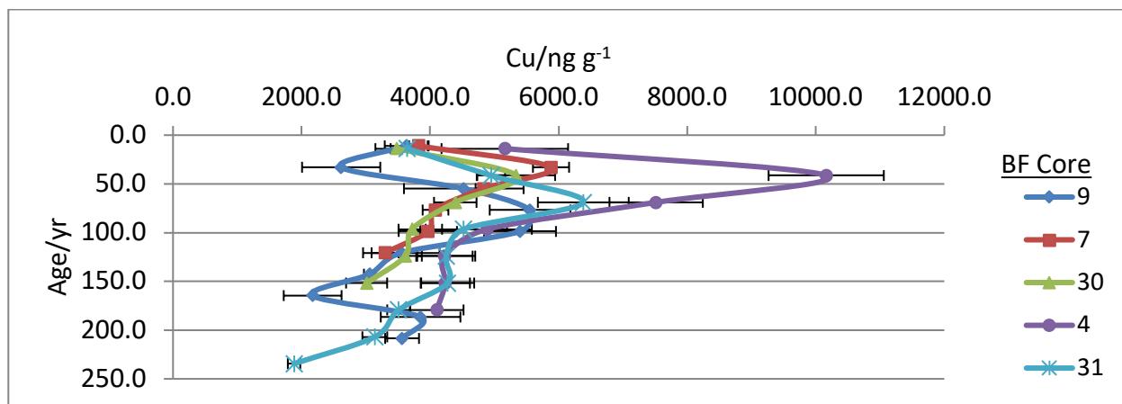
Figure 81. Soil core profiles for MOX-[Cu] in five cores from Region A; (n=3) at the 95% confidence level.
