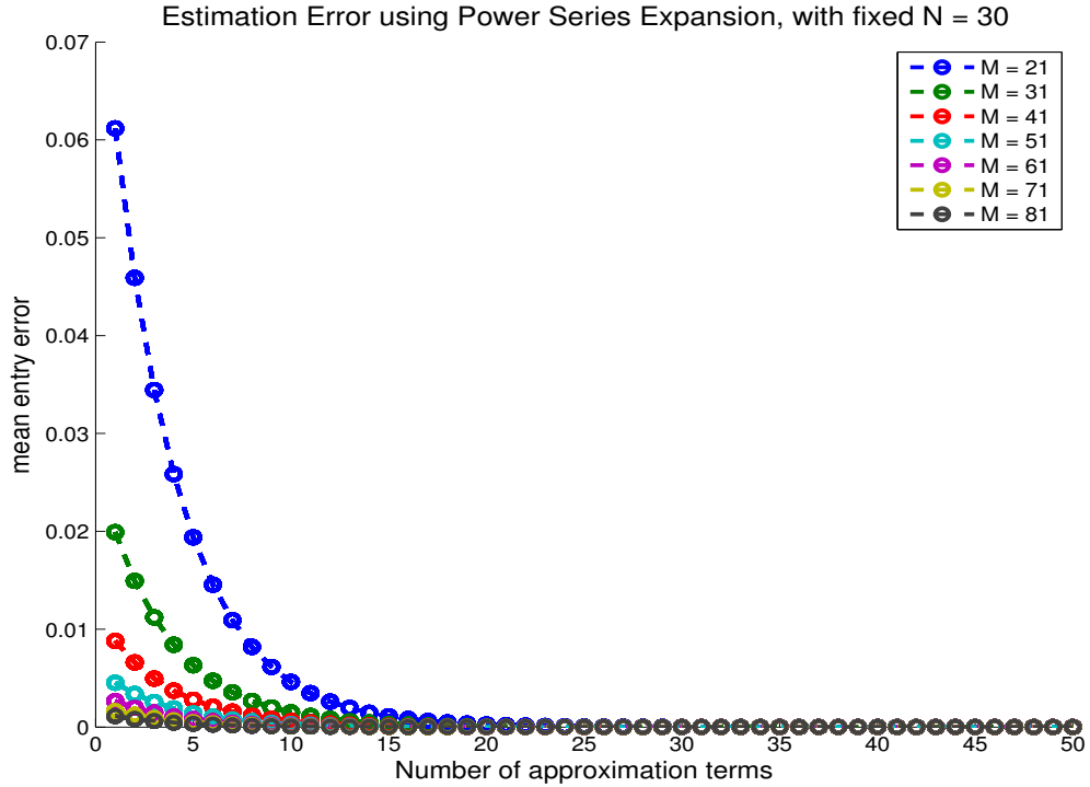
Figure 2.3: Comparing accuracy of the power series estimation of \Sigma_{j|j-1}^{(o)} with varying grid sizes (N fixed, M varies). Shown in figure is the mean entry difference between (\Sigma_{j|j-1}^{(o)})^{-1} and \sum_{j=2}^M G_{j|j-1}^* .
