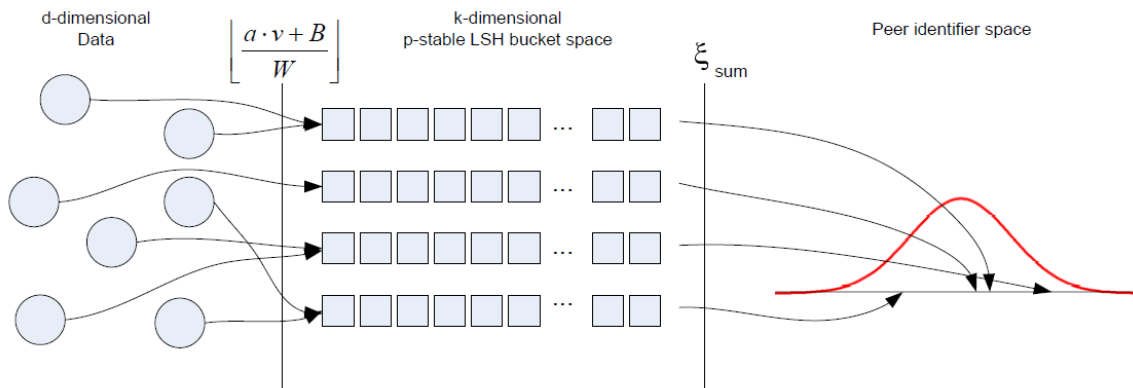
Figure 10: Locality sensitive hashing (Haghani et al., 2008). Two level hashing from d -dimensional data space to peer identifier space.
