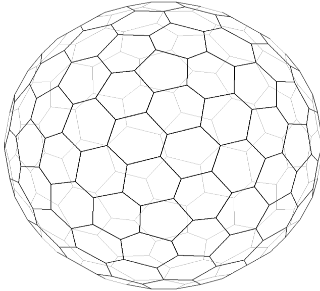
Figure 42: Schematic view of Lovisolò tessellations of a sphere.
