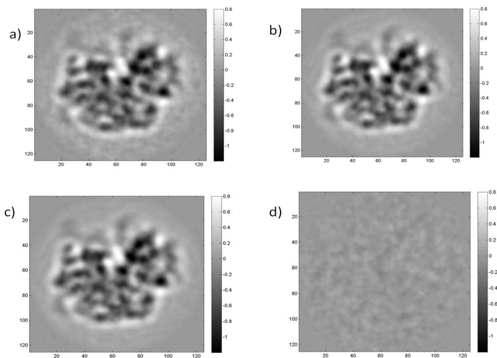
Figure 65: Average from tail (a), core (b) and all (c) snapshots. As the figure shows, averaging does not provide a significant difference between core and tail sections of manifold. d) demonstrate the intensity difference of tail and core averages.
