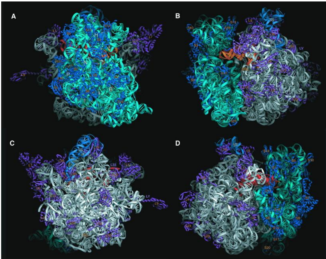
Figure 3: Structure of T. thermophilus ribosome (Yusupov et al., 2001). A) to D) represents 90o rotations of the molecule along vertical axis. Structure is determined with 5.5 Å resolution by X-ray crystallography.
