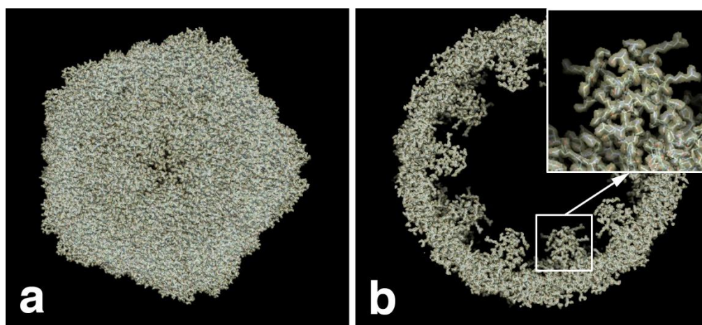
Figure 31: Atomic-resolution structure of the satellite tobacco necrosis virus (Hosseinizadeh et al., 2013). (a) The three-dimensional electron density map with resolution 1/100^{\text{th}} of the object diameter (0.2nm). (b) A slice of the electron density showing atomic resolution.
