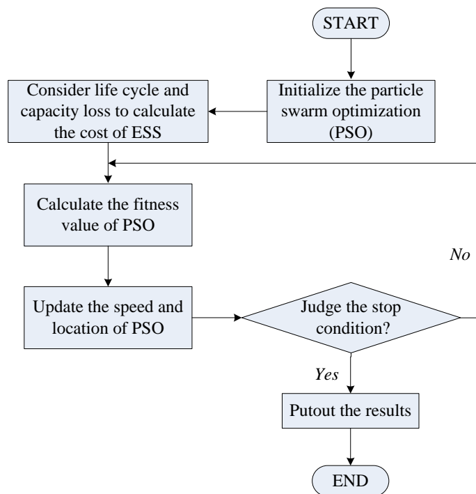
Figure 4-1 PSO flowchart
