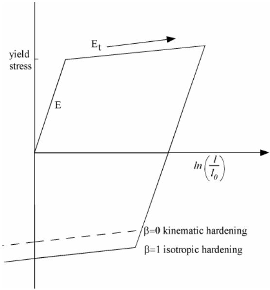
Figure 3-11: Elastic- Plastic behavior with kinematic and isotropic hardening where I_0 and I are undeformed and deformed lengths of uniaxial tension specimen. E_t is the slope of the bilinear stress strain curve.
