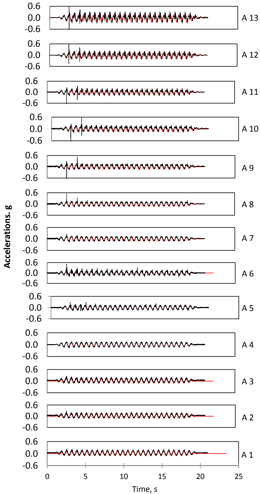
Figure 4-8: Measured (black) and Calculated (red) Acceleration History of GRS Wall Facing (Test 1)
