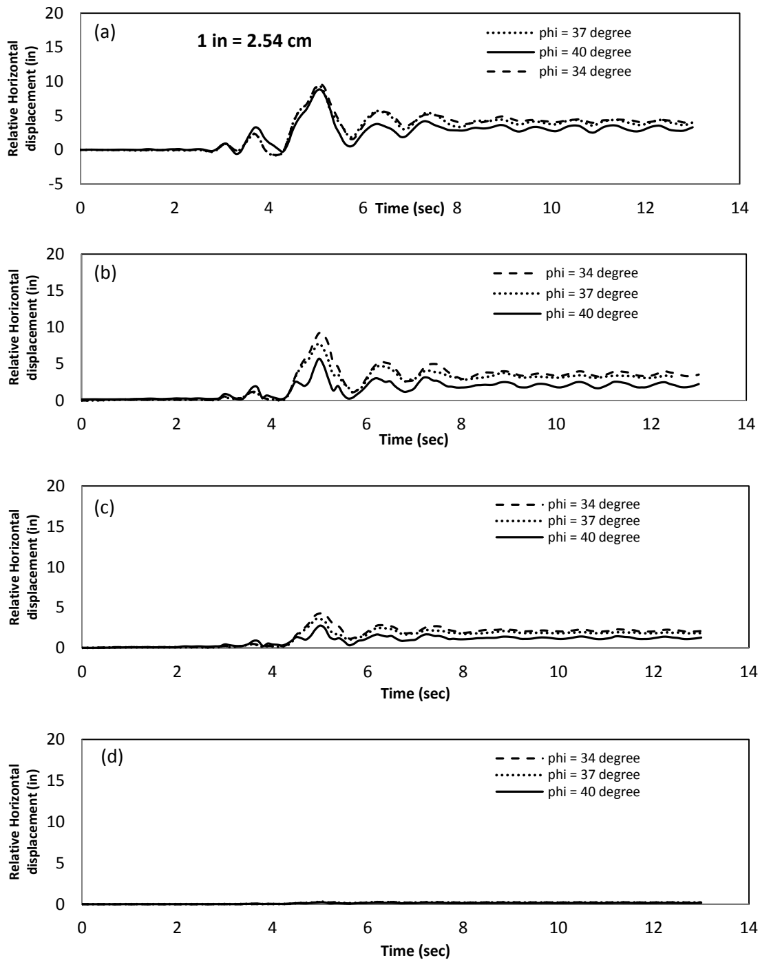
Figure 5-13 Effect of soil friction angle on relative horizontal displacement of the bridge and abutment facing (H=10ft, S=8in, E=700KN/m, Kobe earthquake), (a)bridge, (b)top of the abutment, (c)middle of the abutment, (d)bottom of the abutment.
