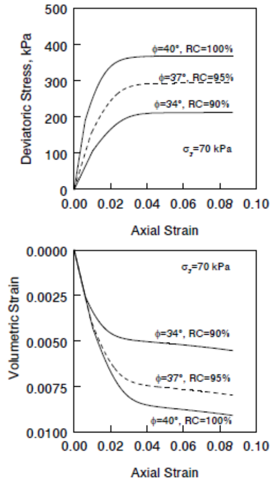
Figure 5-3 Assumed Behavior of Backfill Soils Used in the Parametric Analysis
